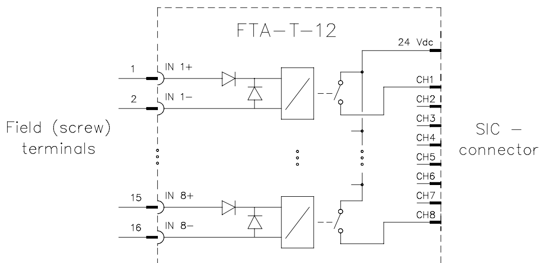
Figure 2 Schematic diagram
