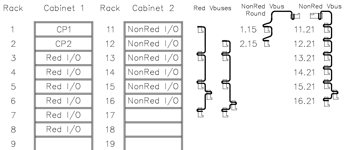
Figure 3 V-Buses example 3
