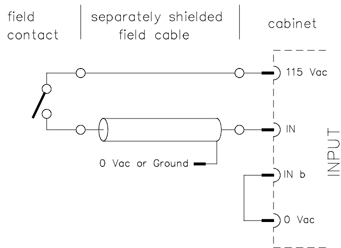
Figure 4 Field cable with separately shielded wires
