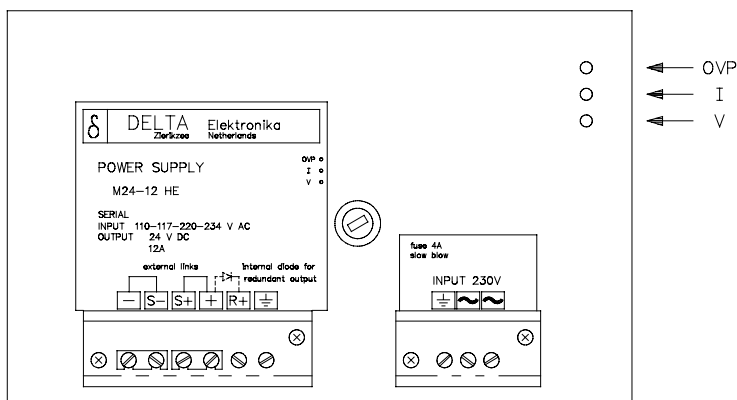
Figure 1 Back view
