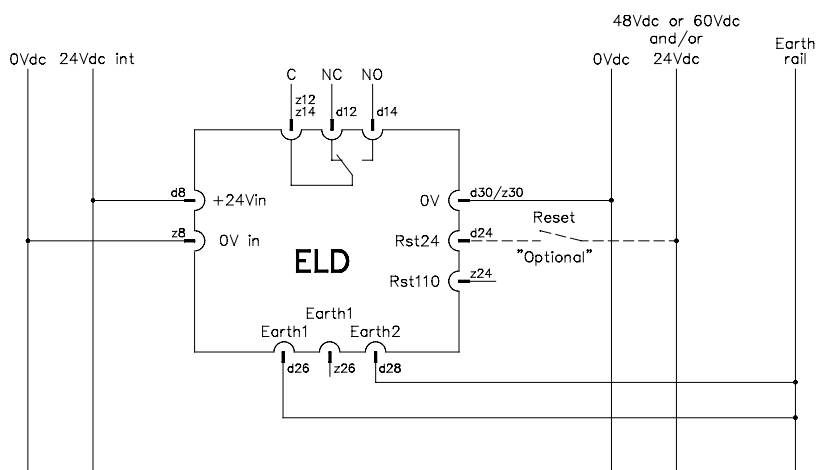
Figure 3 24 Vdc with 48 Vdc and/or 60 Vdc monitoring
