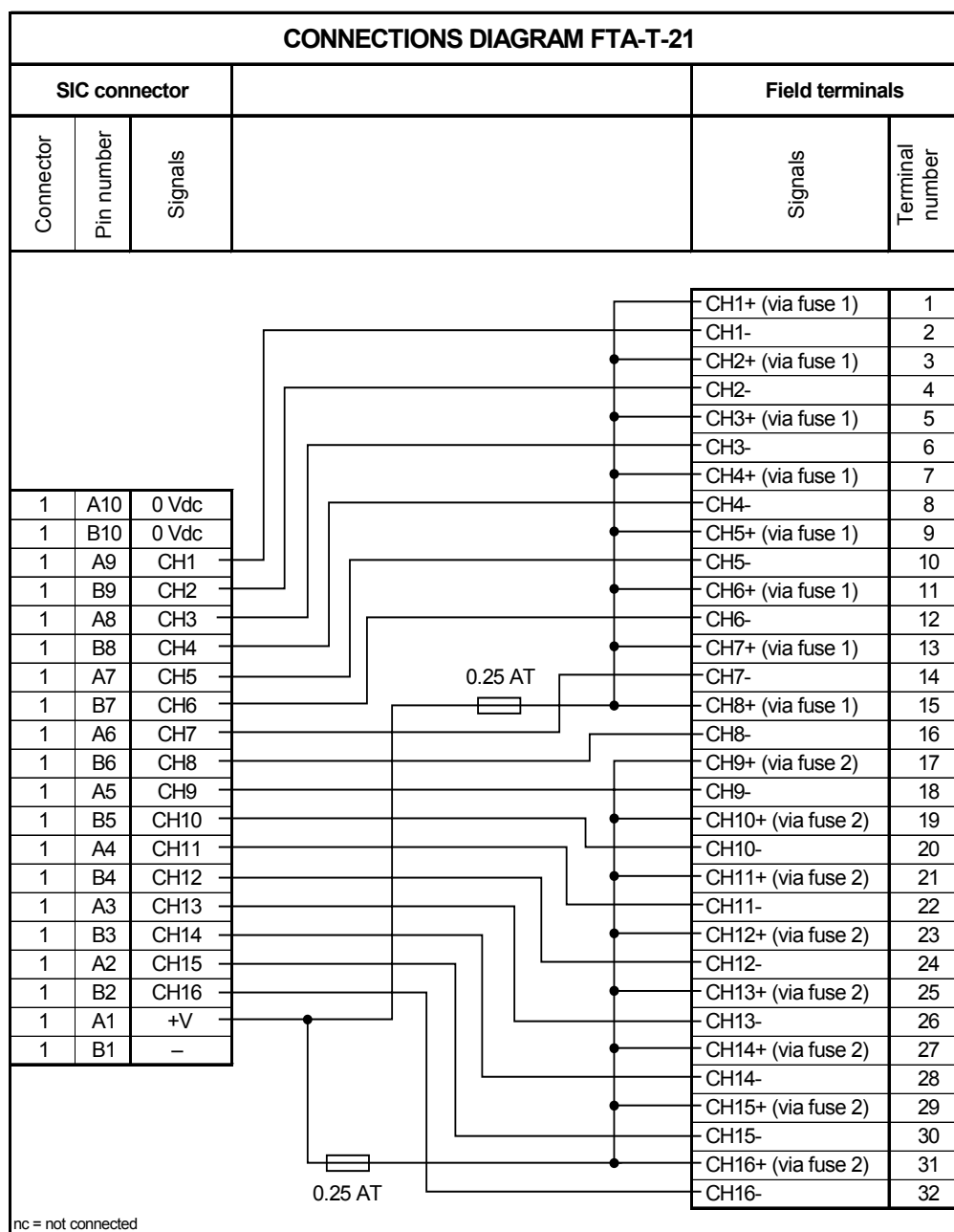
Figure 2 Connections diagram
