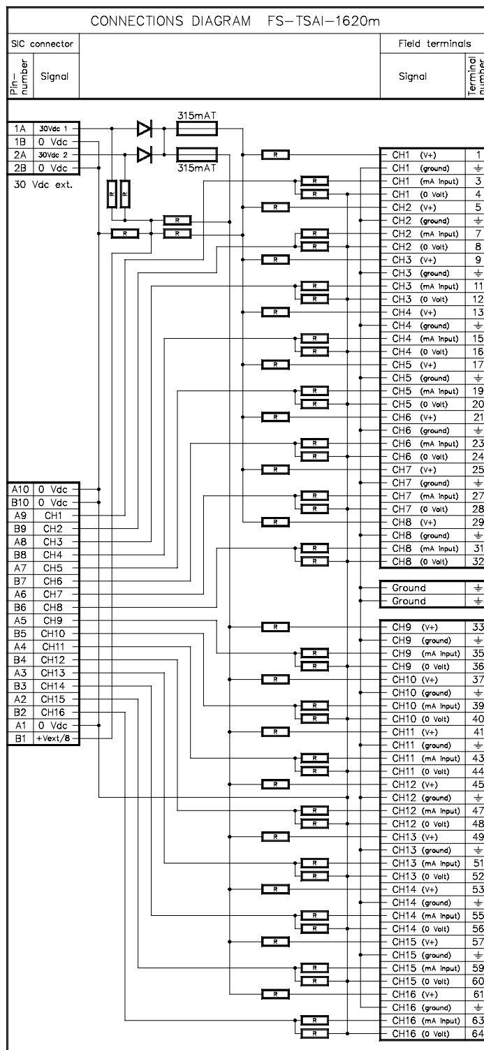
Figure 5 Connections diagram
