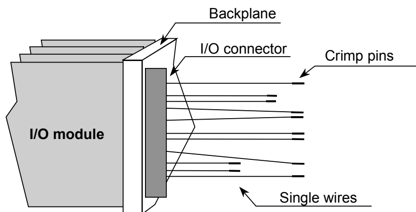
Figure 1 Principle of single-wire connection method
