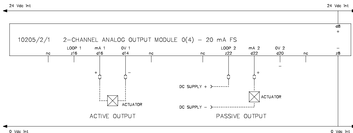
Figure 4 I/O connection example for 10205/2/1 module for non-redundant I/O configurations (one channel active, one channel passive)
