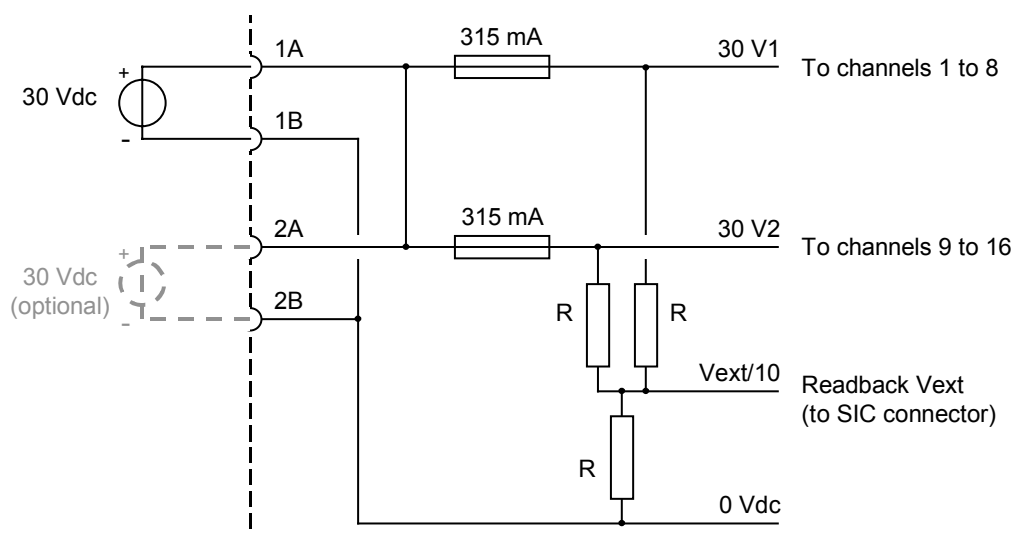
Figure 4 Schematic diagram for power distribution with monitoring
