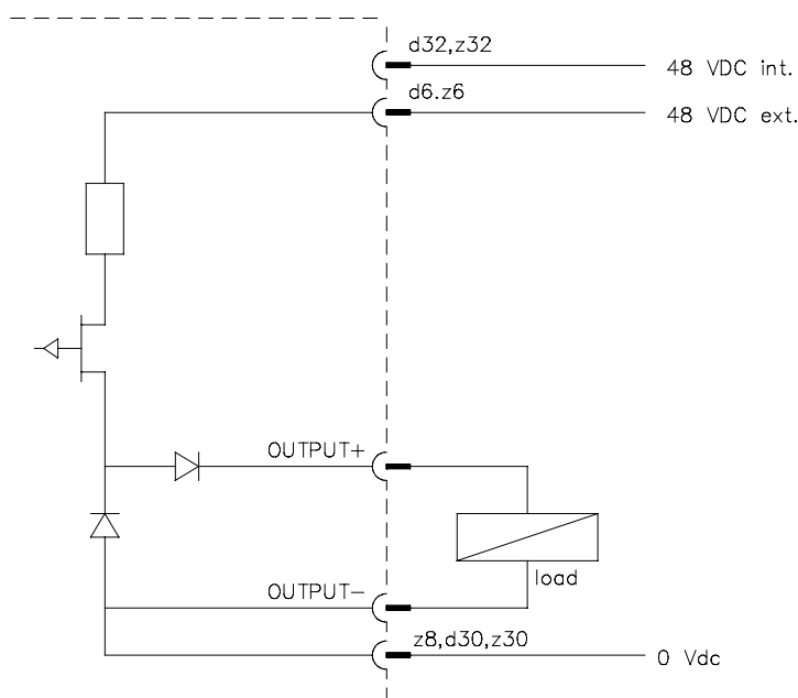
Figure 1 Schematic diagram for connection of one output to the 10213/2/3 module
