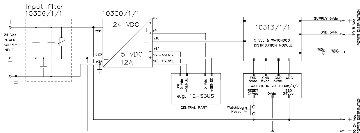
Figure 3 Connection details of 10005/O/2 for one Central Part
