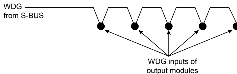
Figure 3 Watchdog wiring
