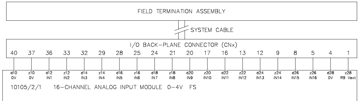
Figure 2 Connection example of 10105/2/1 module to FTA
