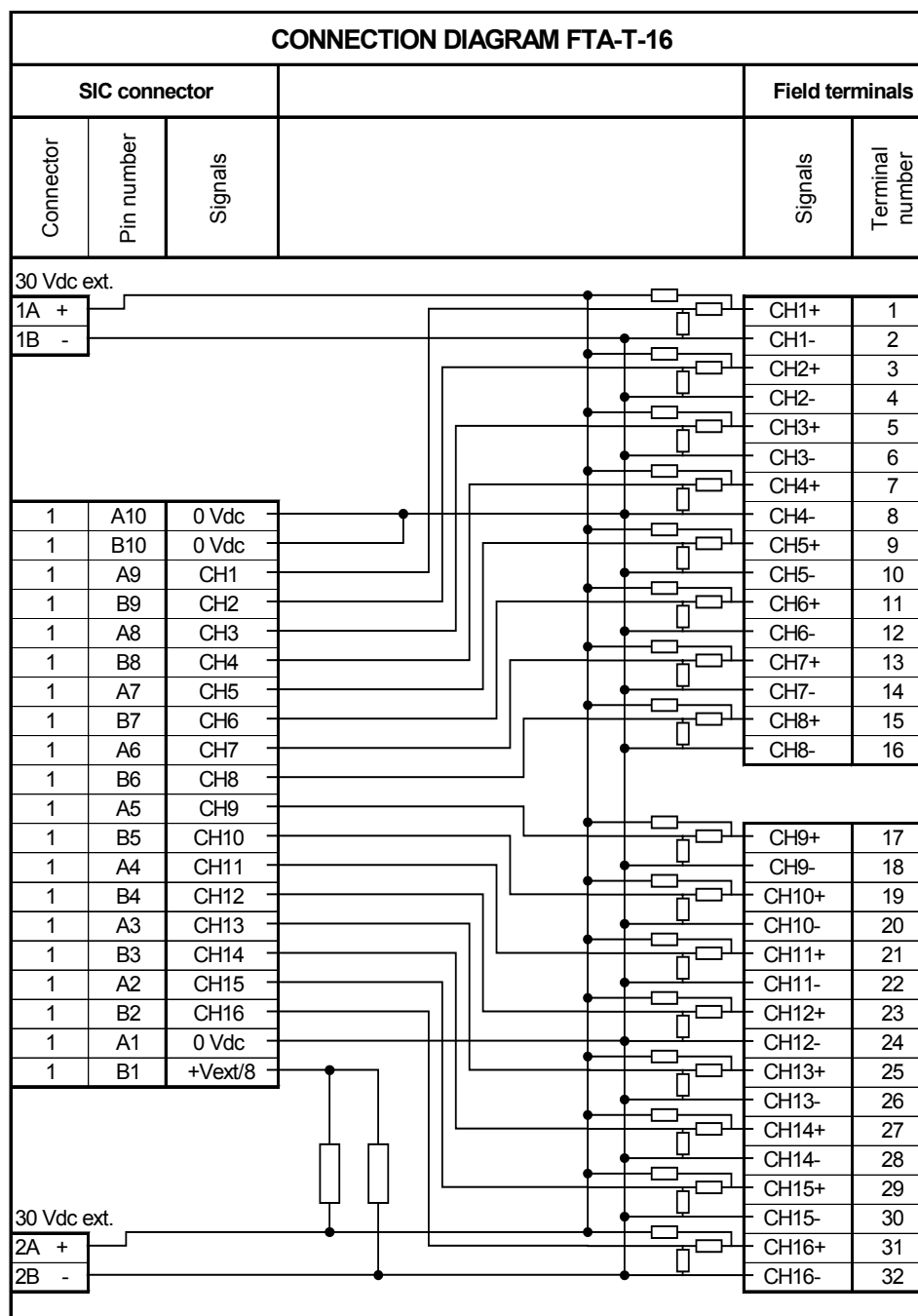
Figure 4 Connections diagram
