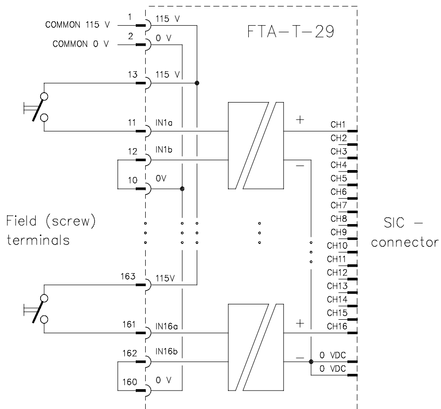
Figure 7 Schematic diagram for connecting passive inputs.
