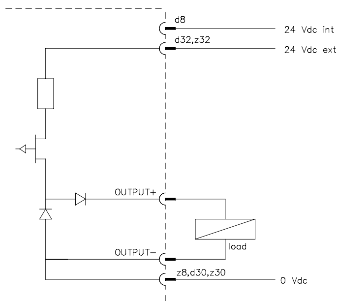
Figure 1 Schematic diagram for connection of one output to the 10201/2/1 module
