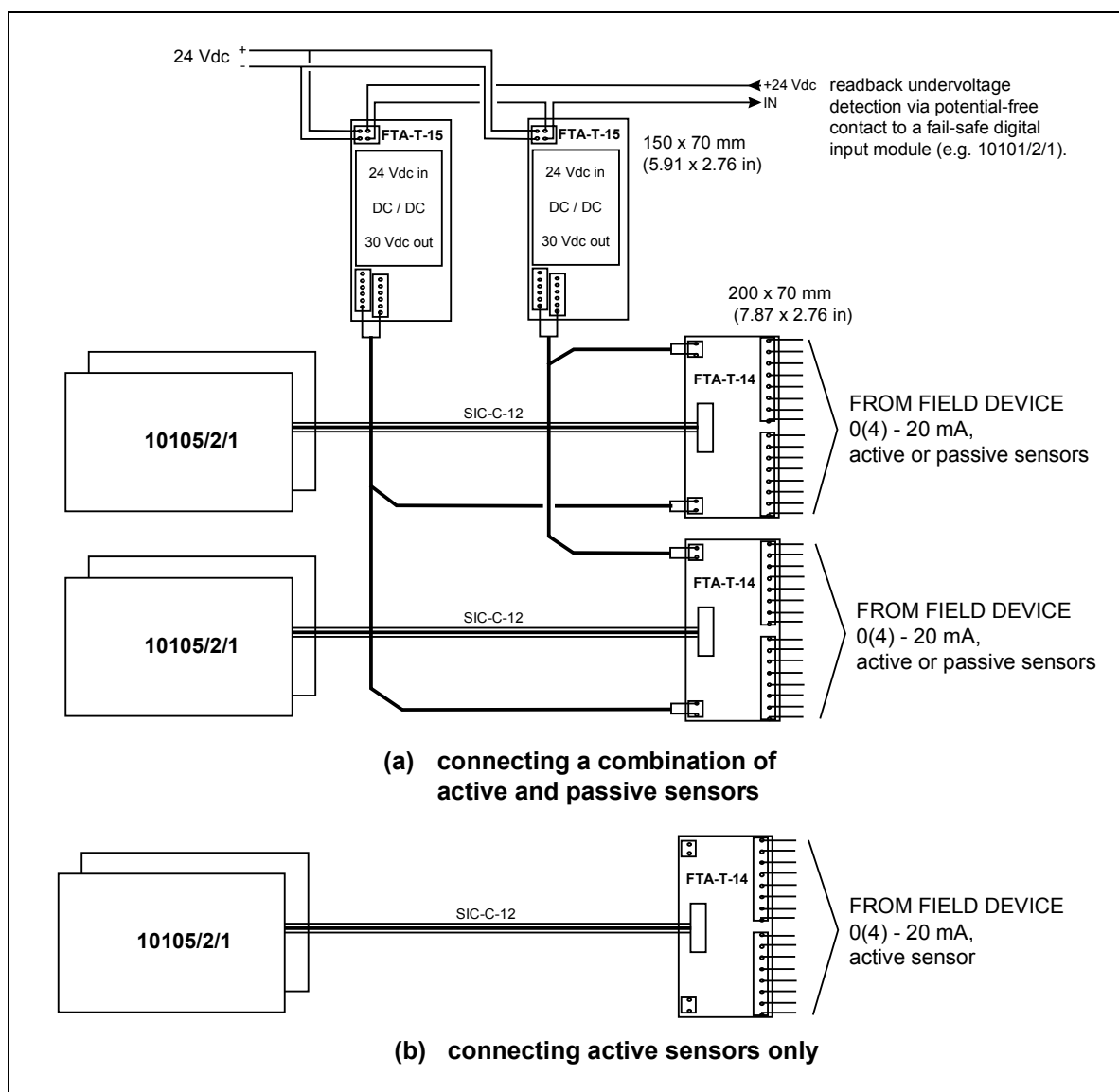
Figure 1 Relationship between FTA-T-14 and FTA-T-15
