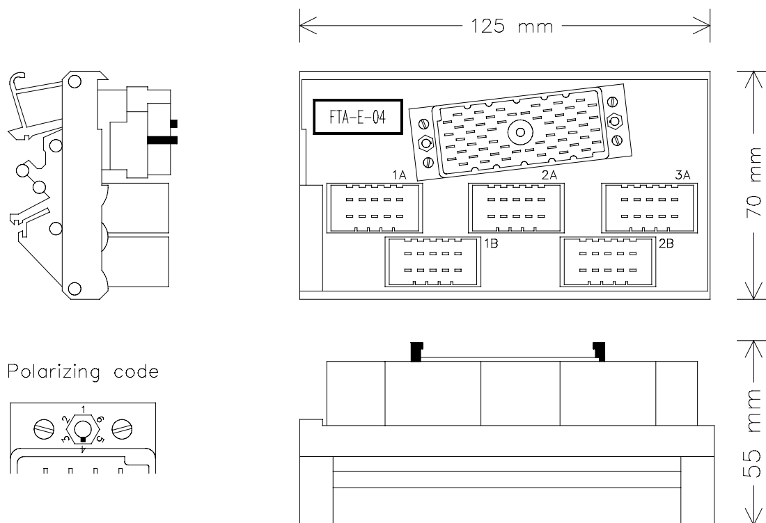
Figure 1 Mechanical layout
