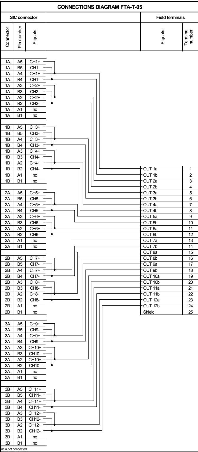
Figure 2 Connections diagram
