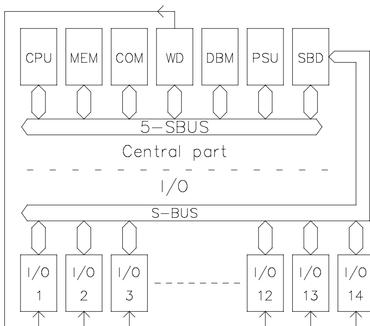
Figure 1 Typical layout
