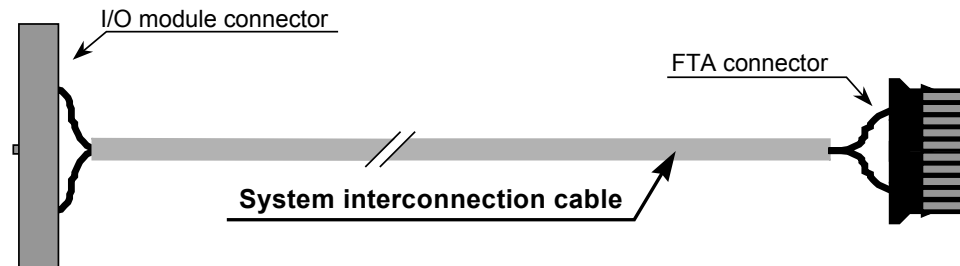
Figure 2 SIC-C cable, layout type 1
