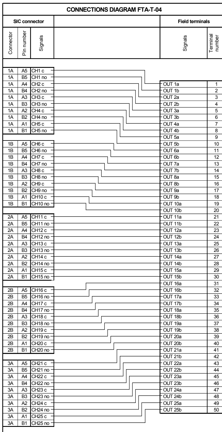
Figure 2 Connections diagram
