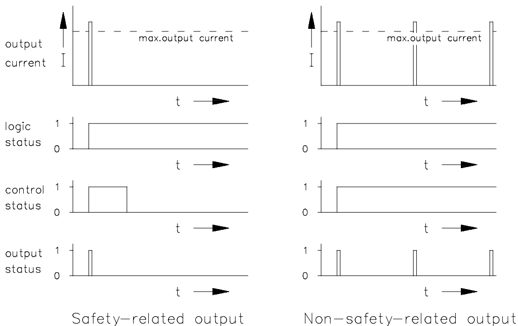
Figure 2 Output overload / short-circuit behavior
