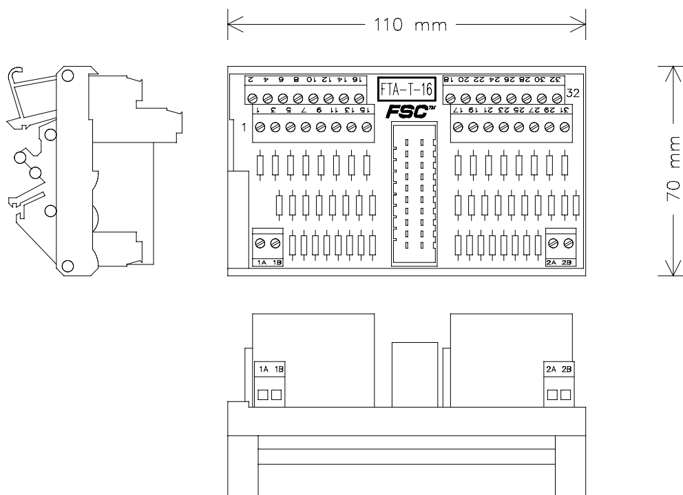
Figure 1 Mechanical layout
