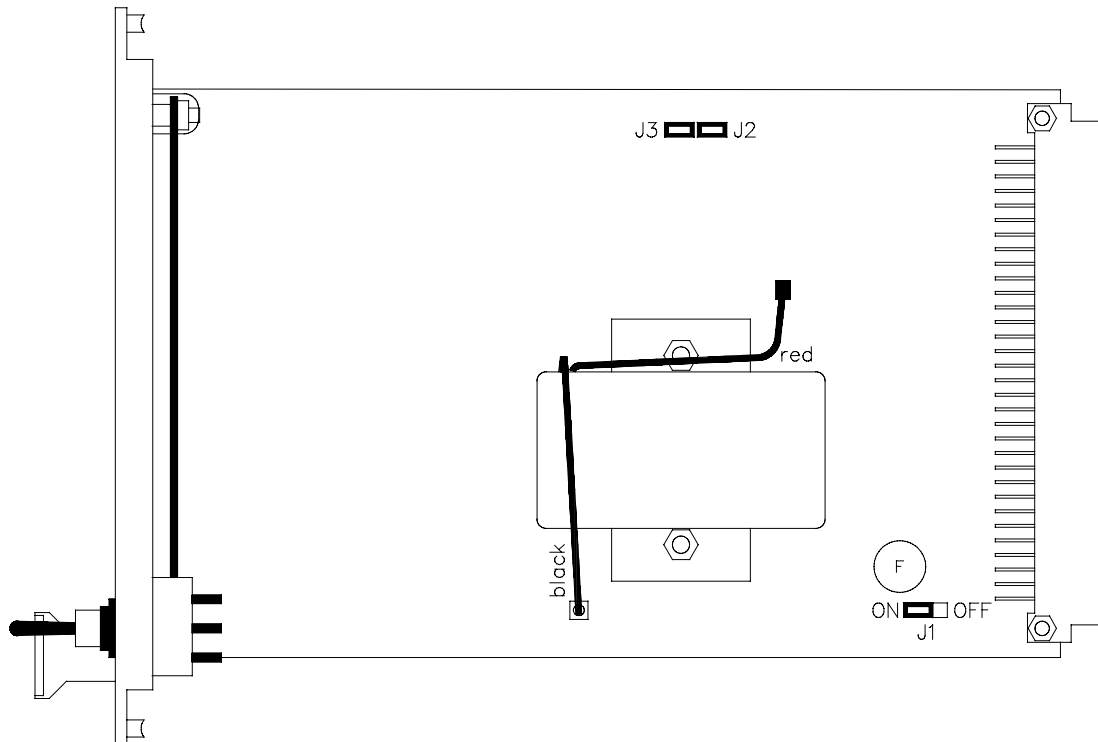
Figure 2 Jumper settings on 10006/2/1 module (08804 shown)
