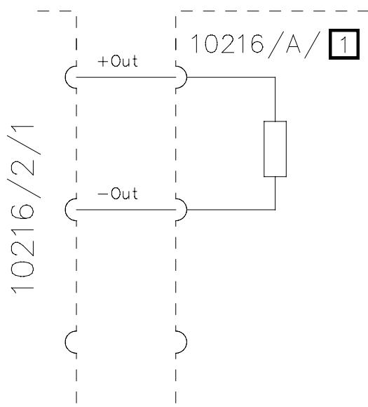
Figure 2 Schematic diagram of a 10216/A/1 module
