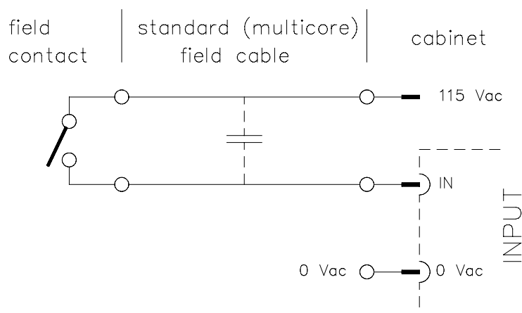
Figure 3 Standard (multicore) field cable
