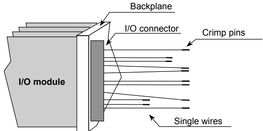
Figure 3 Principle of single-wire connection method
