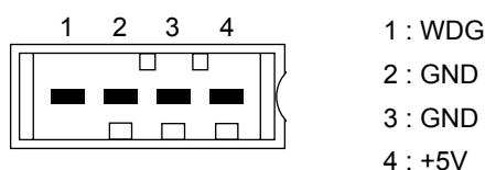
Figure 5 Pin connections of 'CP' and 'CP/CP-1' connector
