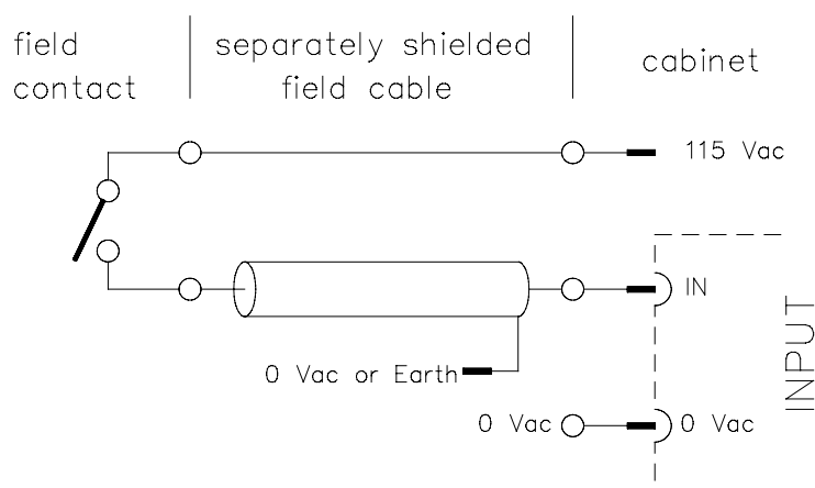
Figure 4 Field cable with separately shielded wires
