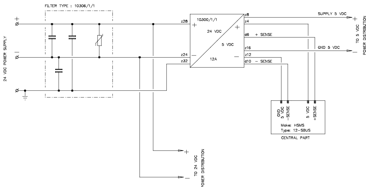
Figure 4 Wiring diagram
