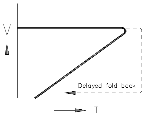
Figure 2 Delayed foldback
