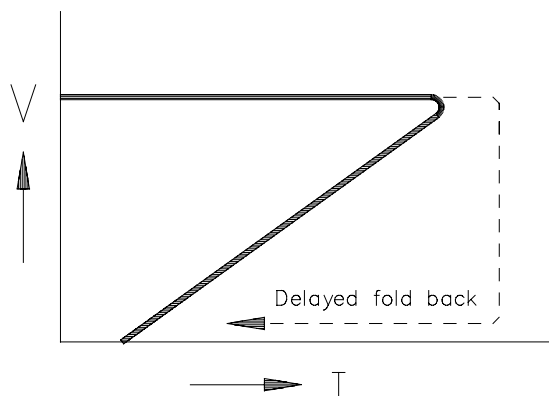
Figure 2 Delayed foldback
