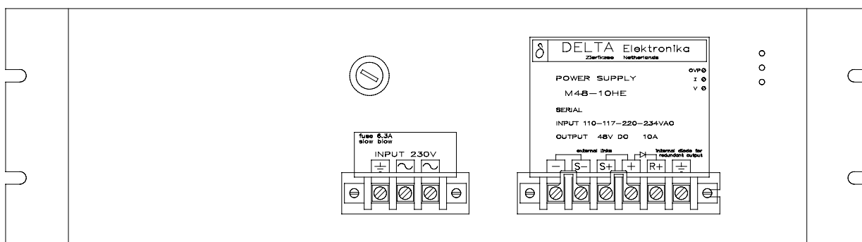
Figure 1 Front view
