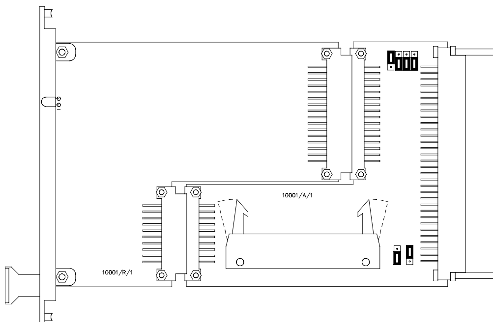
Figure 2 Module layout
