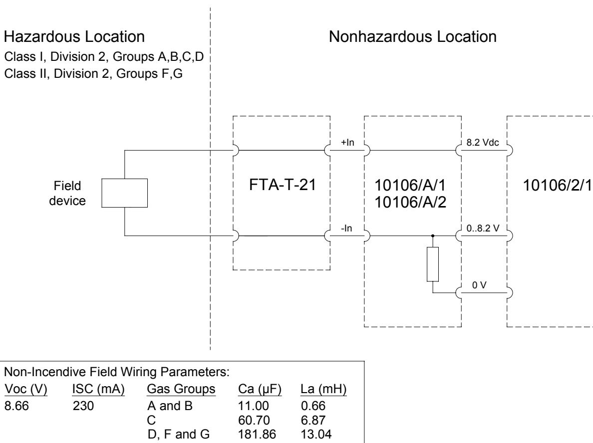
Figure 4 Connection of input in hazardous locations
