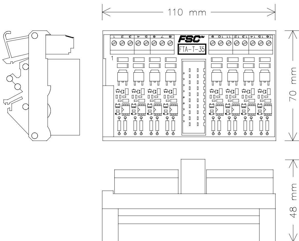
Figure 1 Mechanical layout
