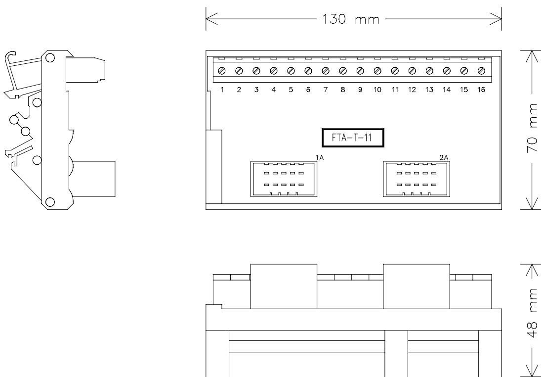
Figure 1 Mechanical layout
