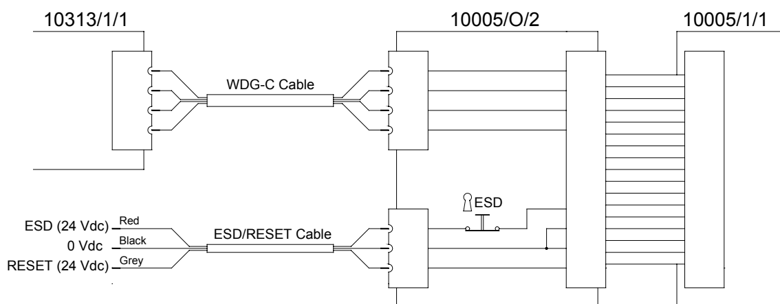
Figure 2 Schematic diagram
