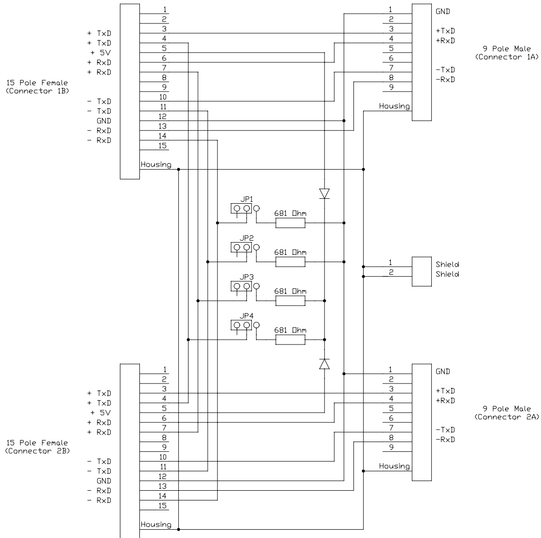
Figure 2 Connection diagram
