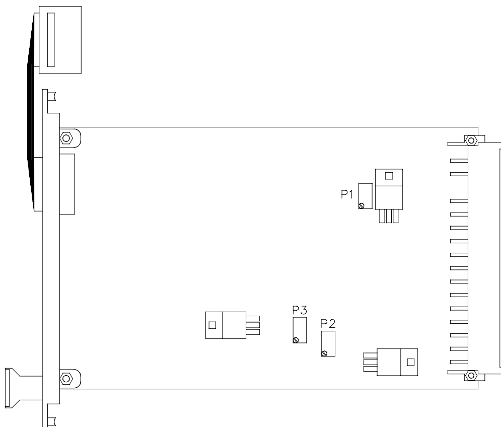
Figure 6 Location of potentiometers on 10205/2/1 module
