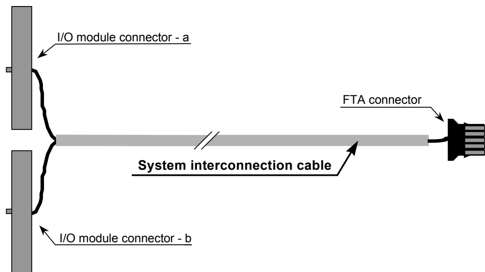
Figure 6 SIC-C cable, layout type 5
