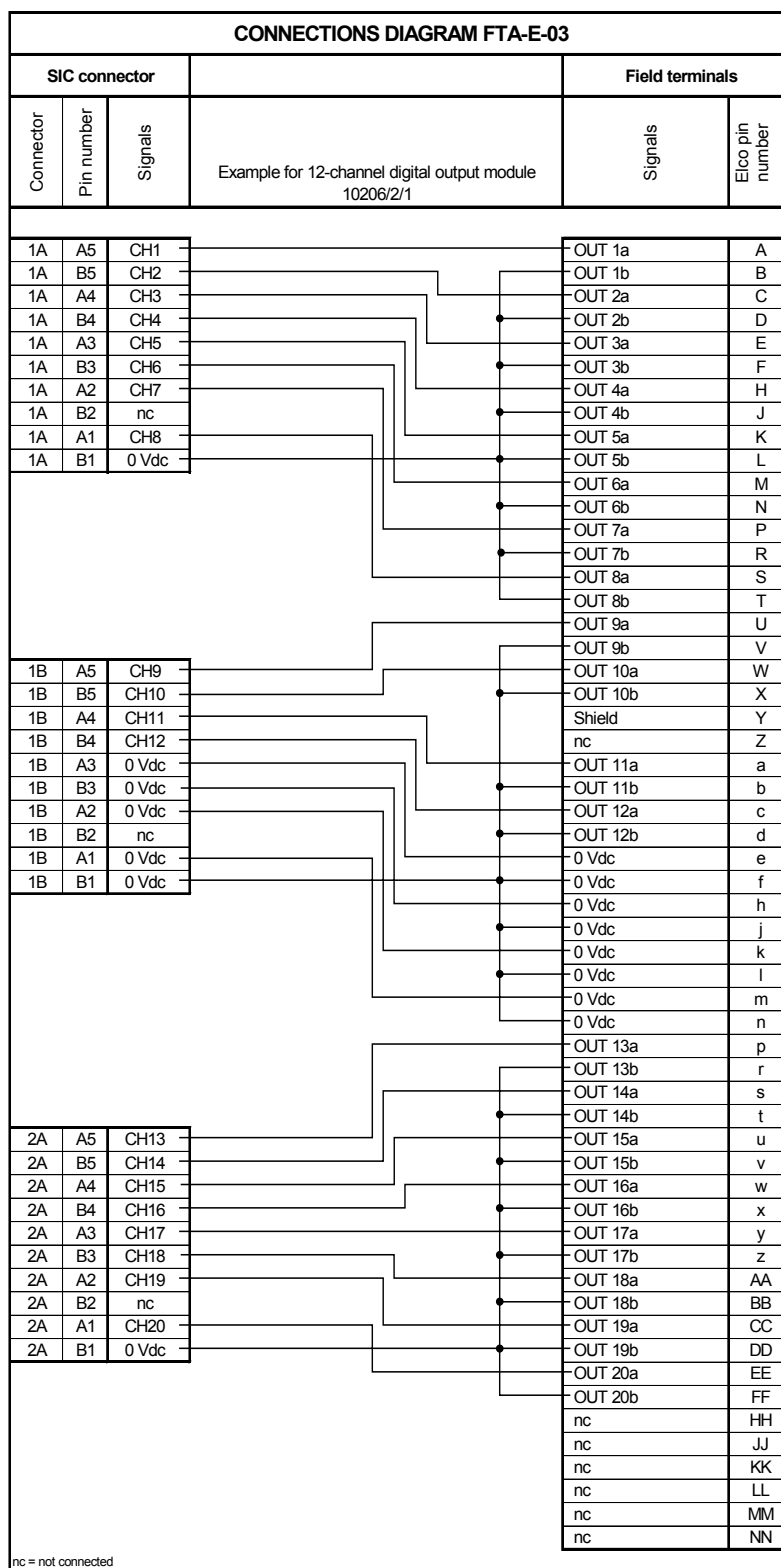
Figure 3 Connections diagram (example for 12-channel digital output module 10206/2/1)
