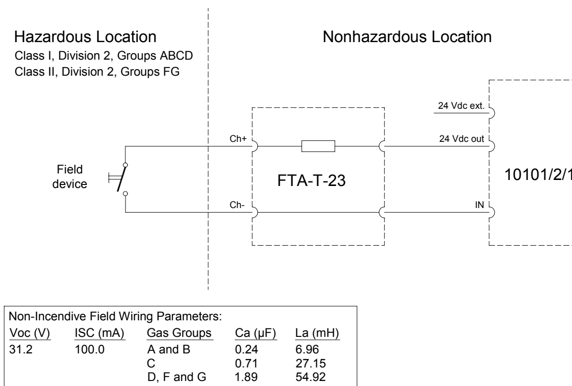
Figure 5 Connection of input in hazardous locations
