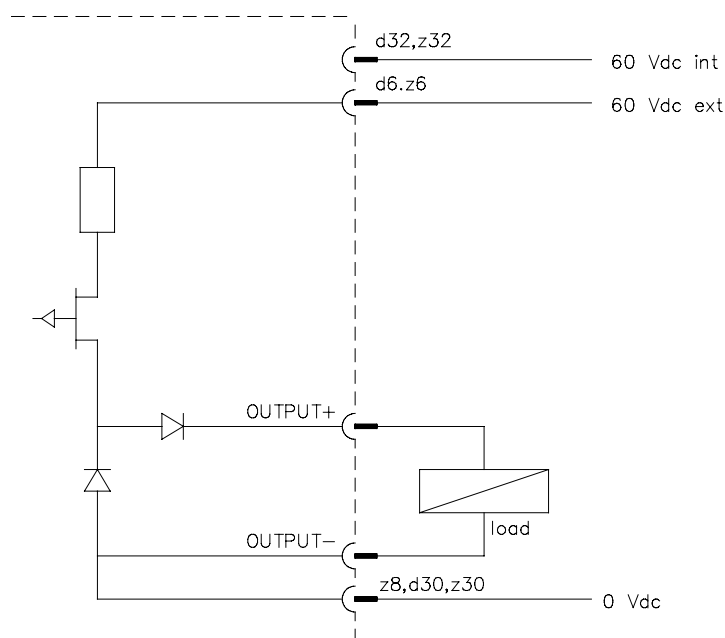
Figure 1 Schematic diagram for connection of one output to the 10213/2/2 module
