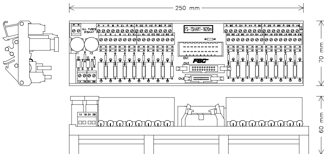
Figure 1 Mechanical layout
