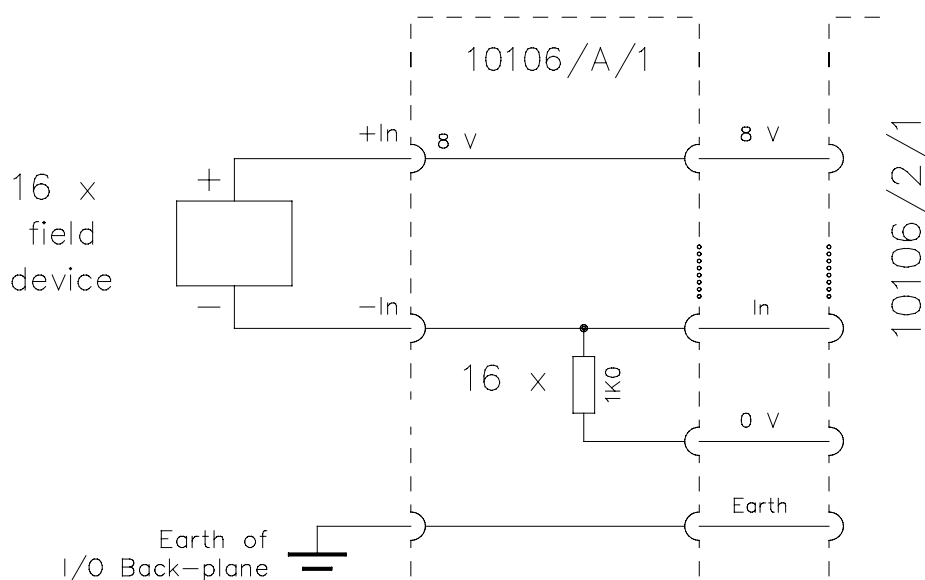
Figure 1 Schematic diagram
