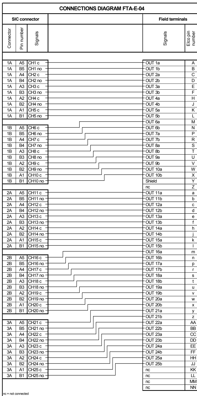
Figure 2 Connections diagram
