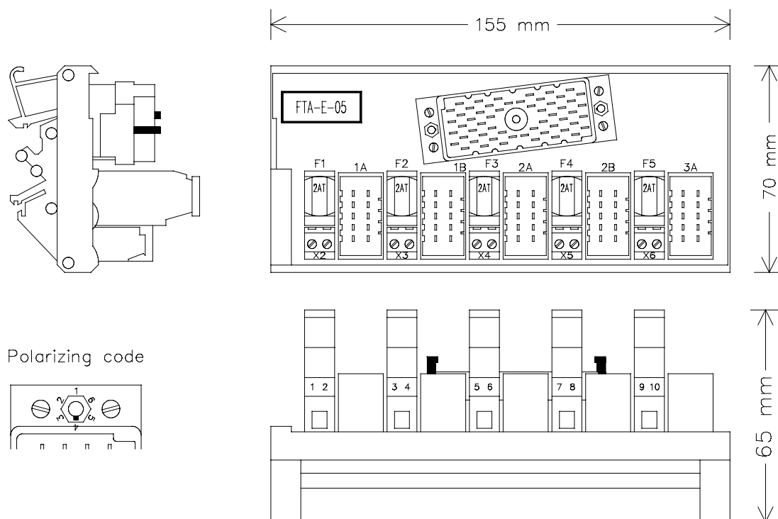
Figure 1 Mechanical layout
