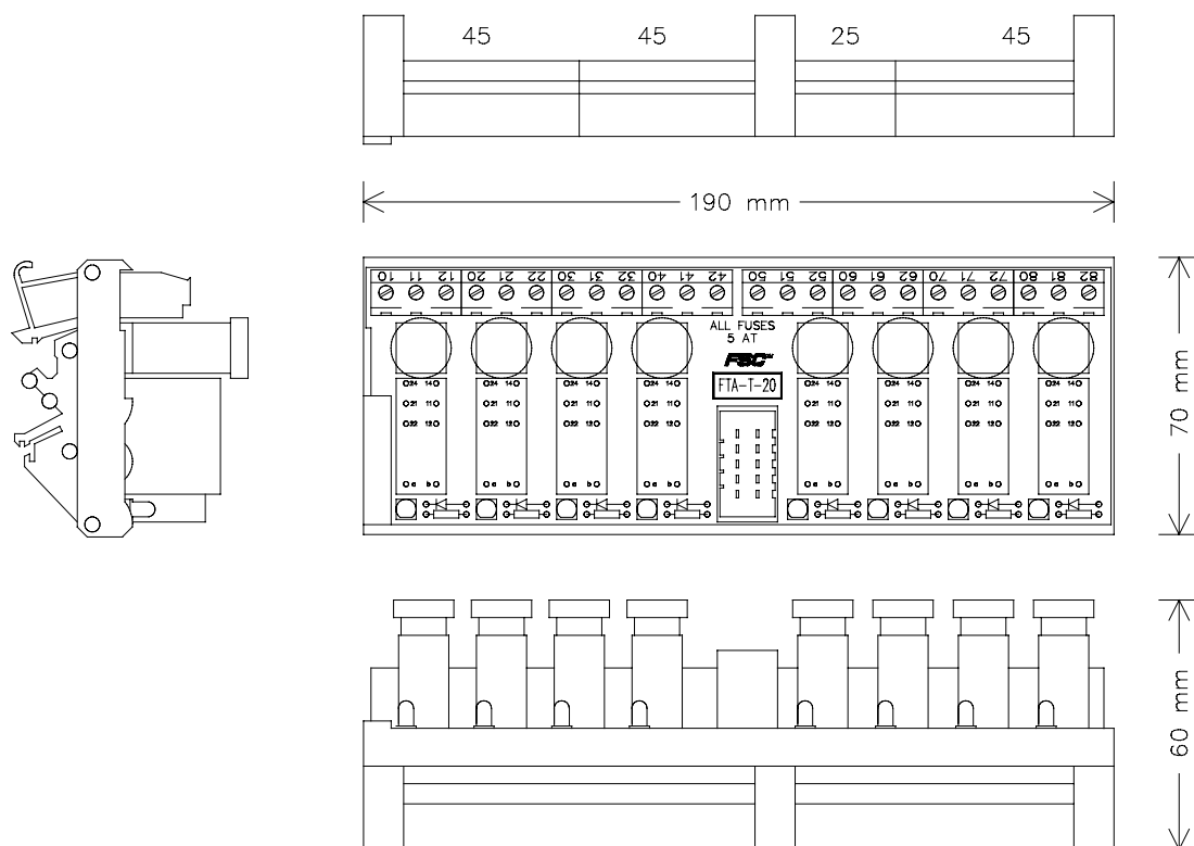
Figure 1 Mechanical layout
