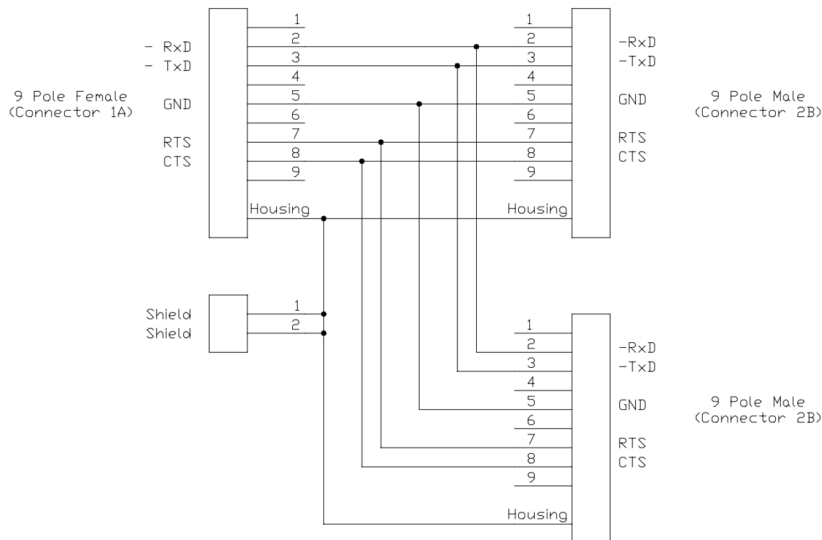
Figure 2 Connection diagram
