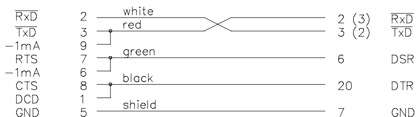
Figure 23 Connection between FSC system and printer: 25-pin connector with hardware handshake (using F-interface)
