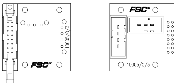
Figure 1 Mechanical layout
