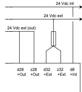
Figure 3 I/O connection example of 10101/2/3 module for non-redundant I/O configurations
