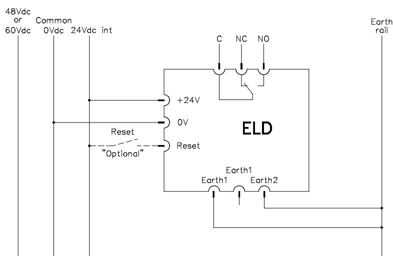
Figure 3 24 Vdc with 48 Vdc or 60 Vdc monitoring
