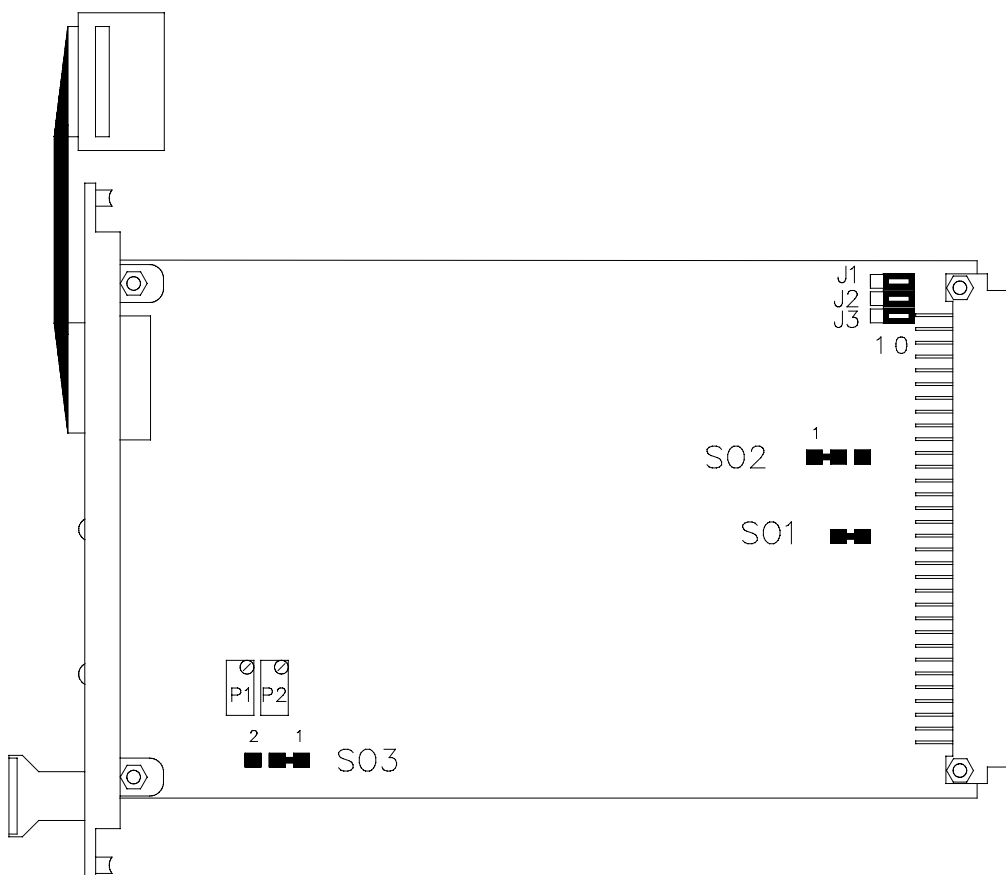
Figure 3 Jumper settings on 10005/1/1 module
