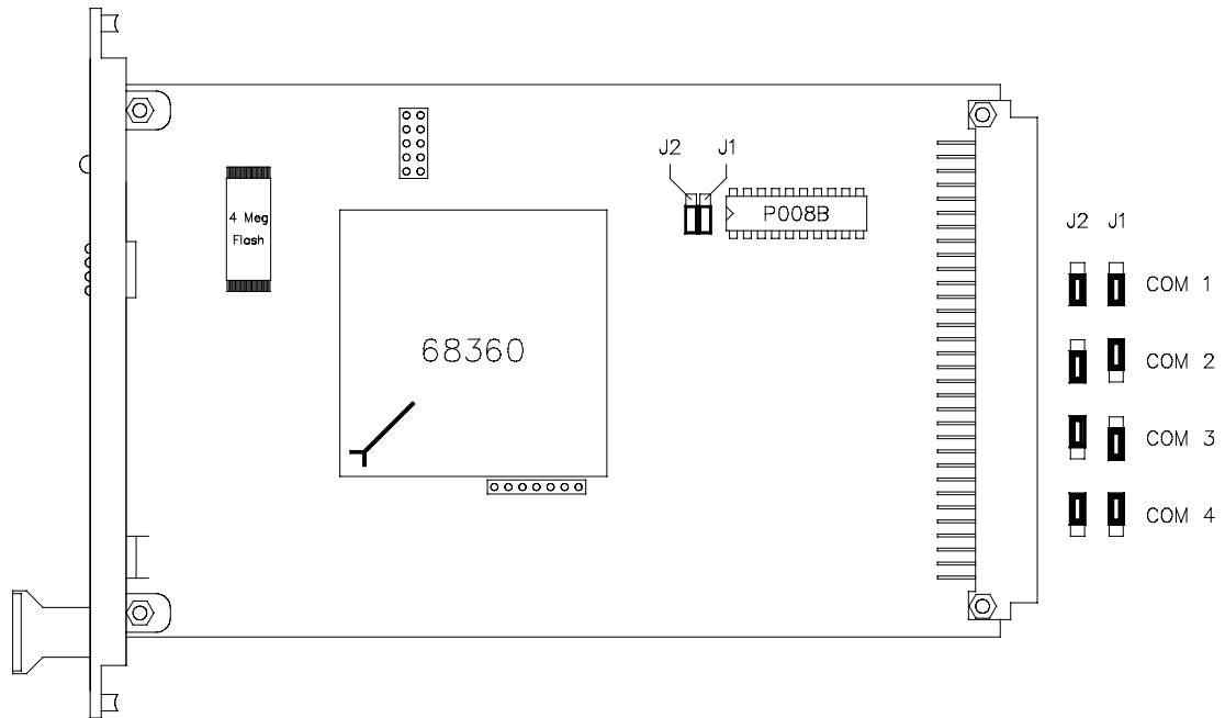
Figure 2 Jumper positions on 10018/2/U
