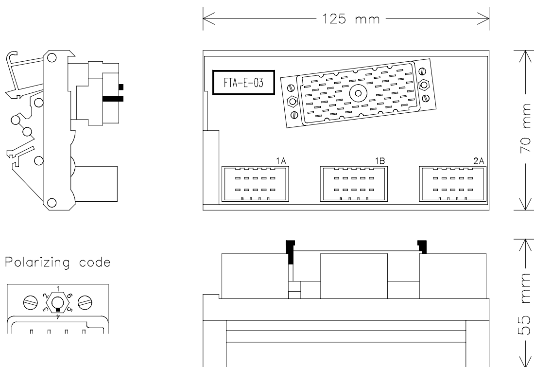
Figure 1 Mechanical layout
