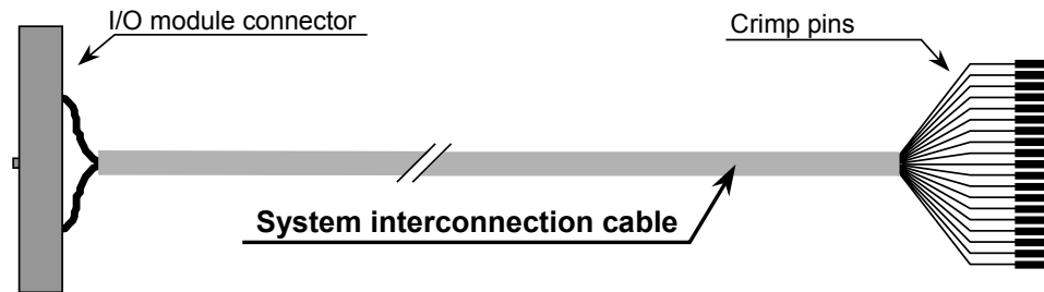
Figure 2 SIC-P cable, layout type 1
