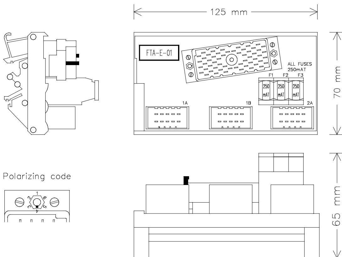
Figure 1 Mechanical layout
