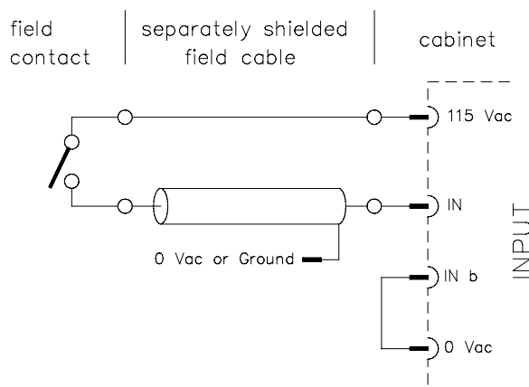
Figure 3 Standard (multicore) field cable
