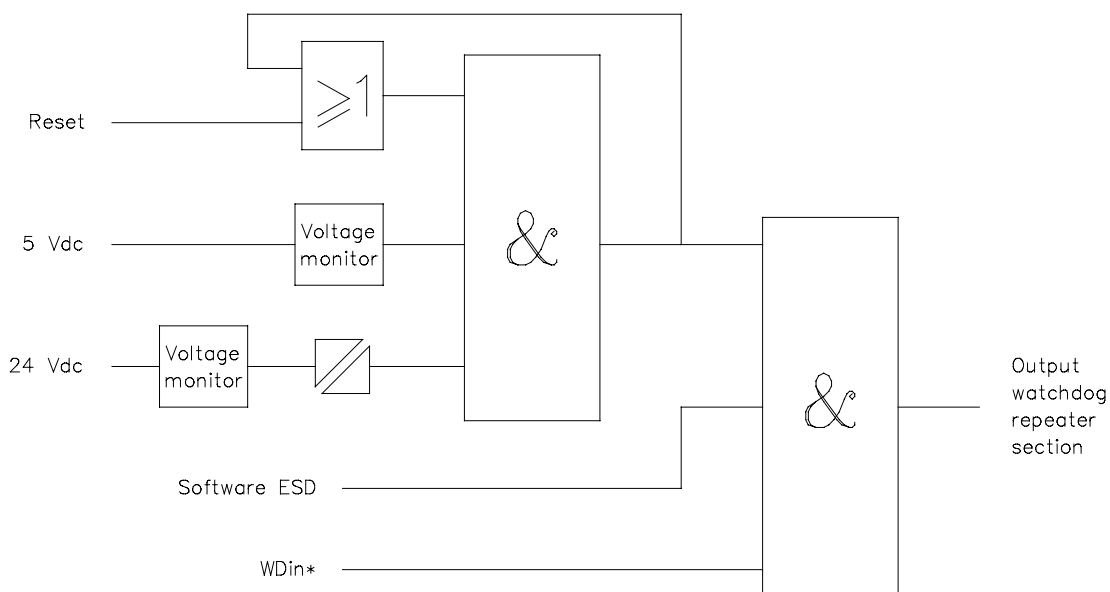
Figure 1 Logic diagram for a watchdog repeater section
