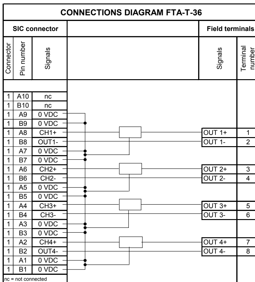
Figure 3 Connections diagram
