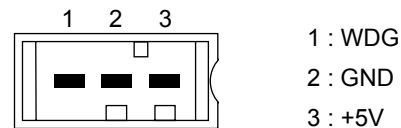
Figure 4 Pin connections of SCN-x
