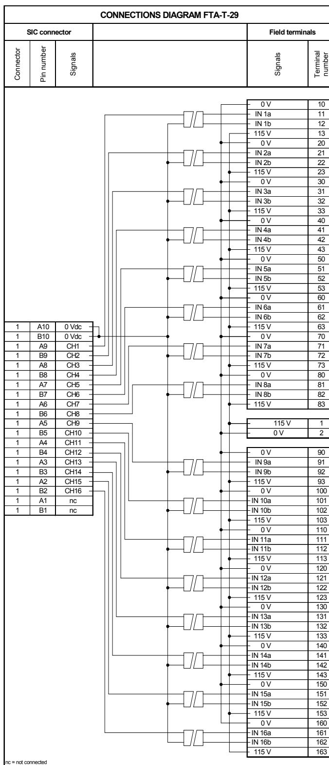
Figure 8 Connections diagram
