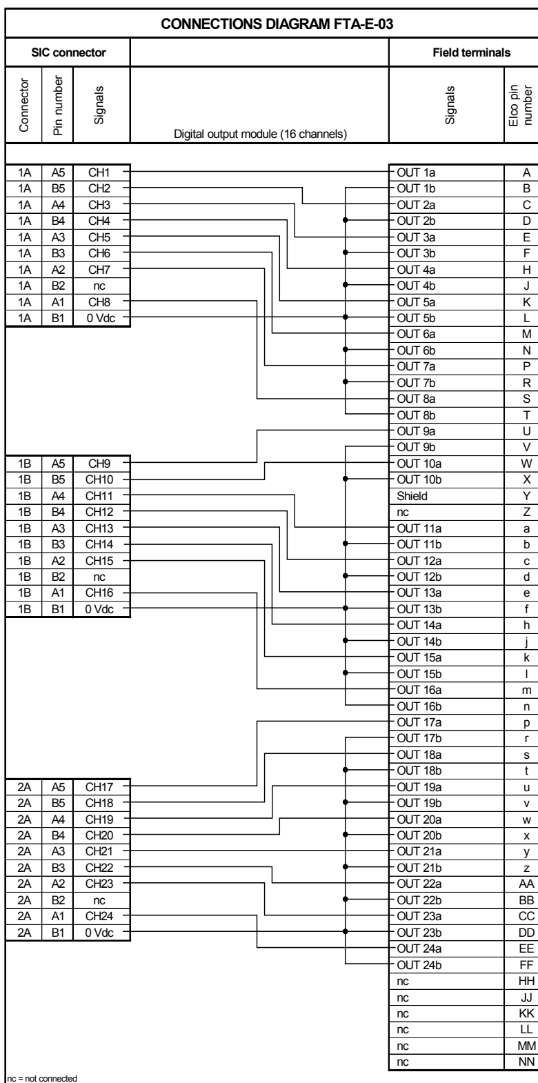
Figure 2 Connections diagram (for 16-channel digital output modules)
