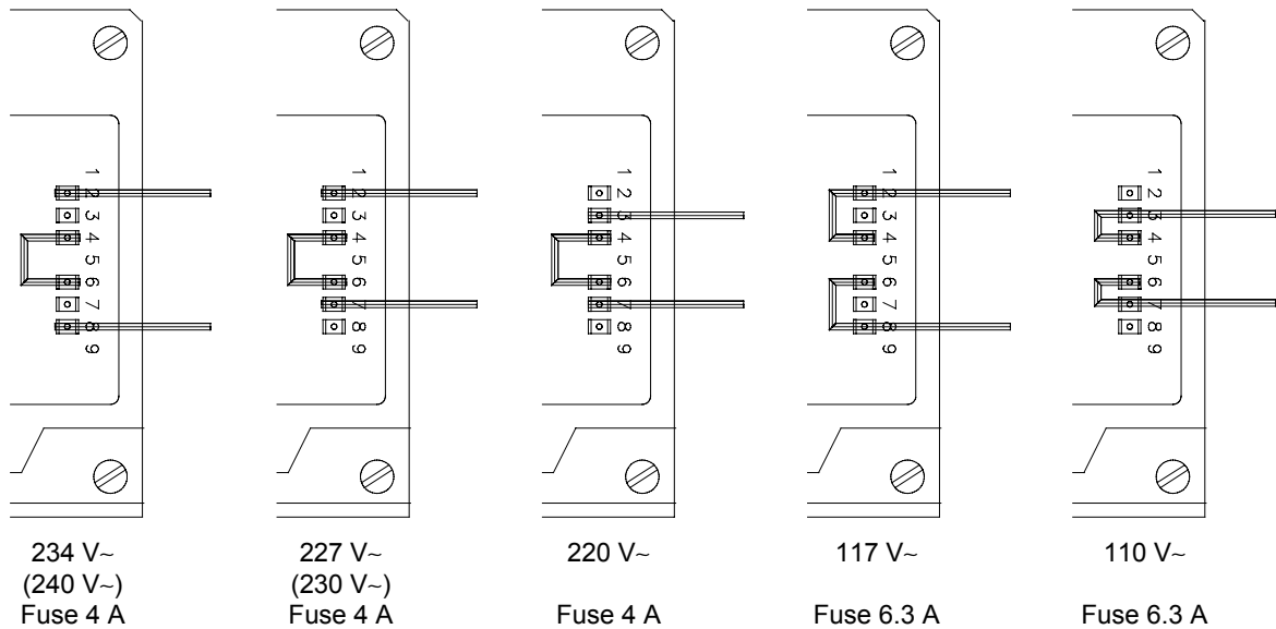
Figure 4 Transformer connections: primary side
