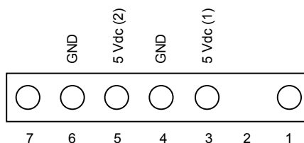
Figure 2 Connector CN5 (detail)
