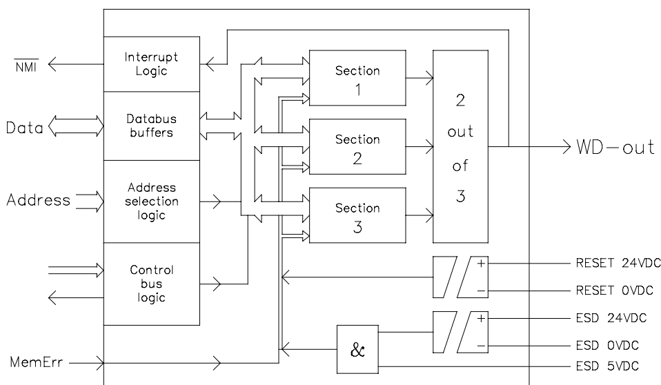
Figure 2 Watchdog module
