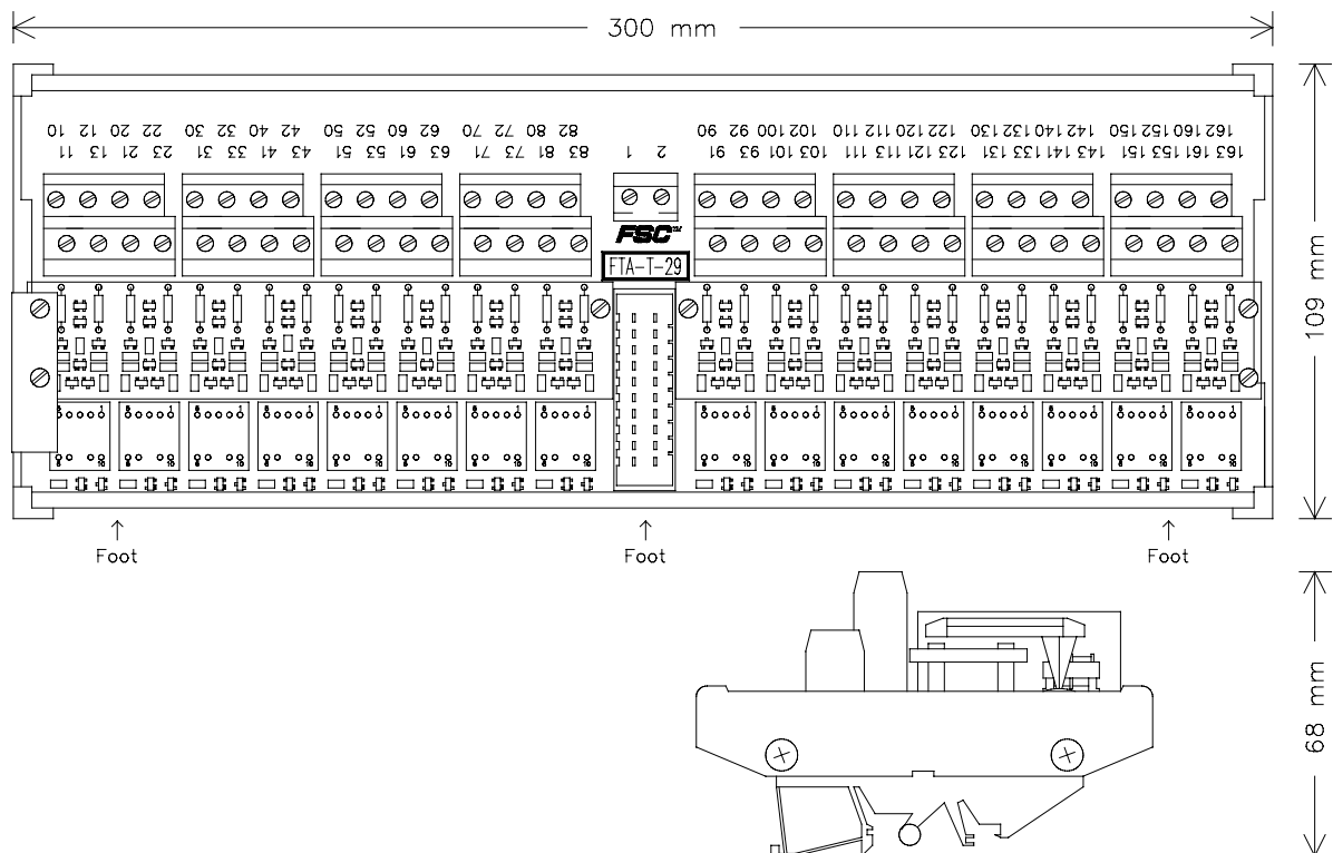
Figure 1 Mechanical layout
