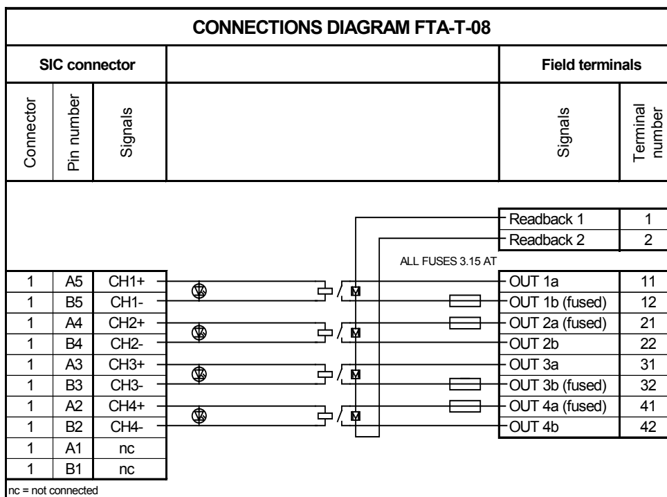
Figure 3 Connections diagram
