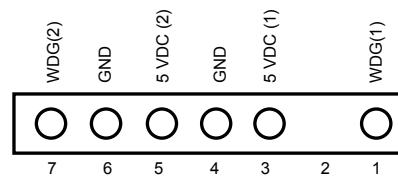
Figure 6 Connector CN22 (detail)
