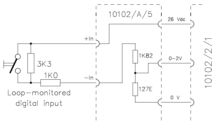
Figure 6 Schematic diagram of 10102/A/5 module
