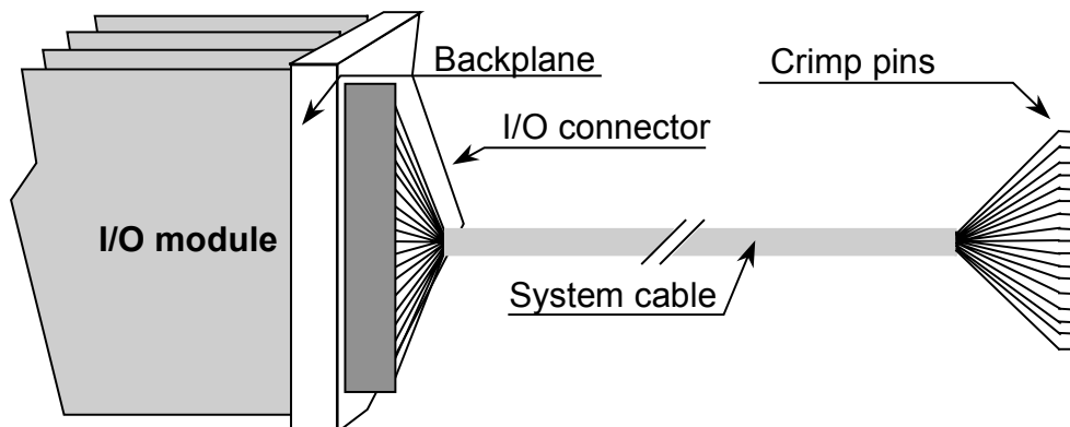
Figure 2 Principle of SIC-P connection method
