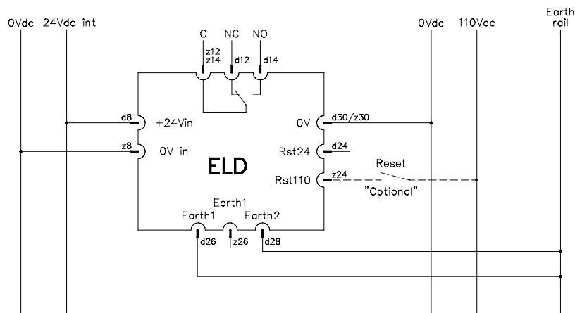
Figure 4 110 Vdc monitoring
