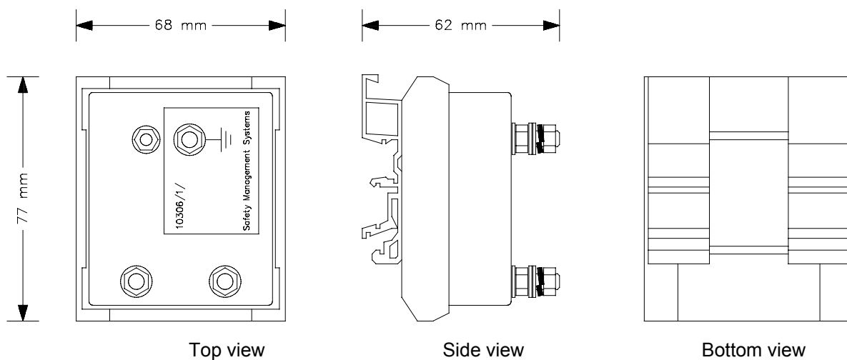
Figure 1 10306/1/. mechanical layout
