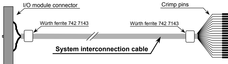
Figure 3 SIC-P cable, layout type 2
