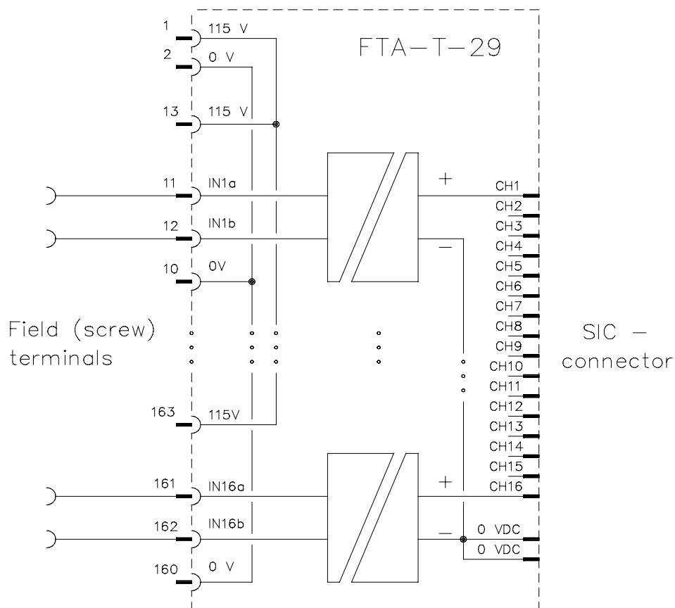
Figure 6 Schematic diagram for connecting active inputs.
