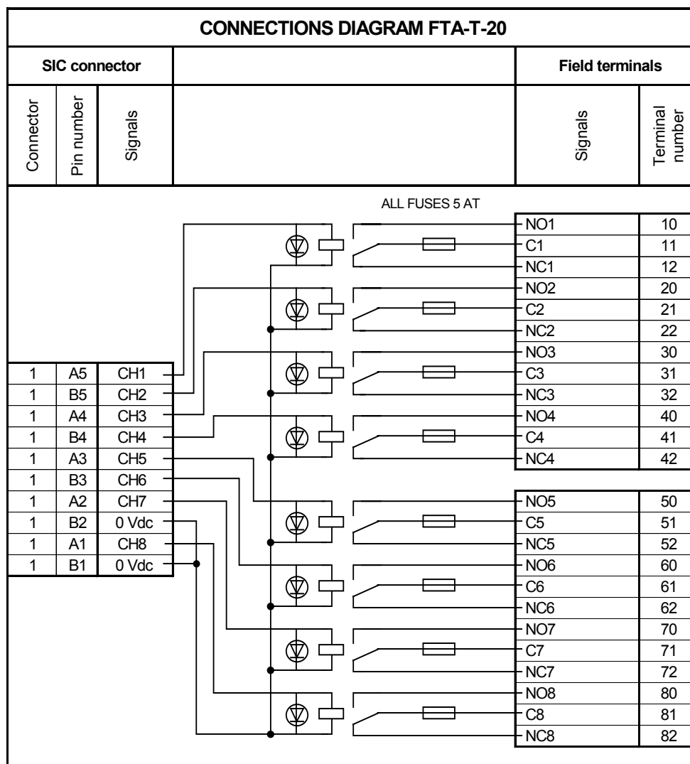
Figure 3 Connections diagram
