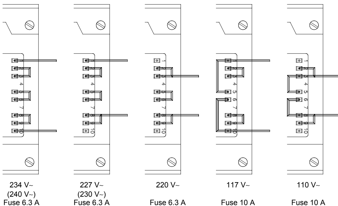
Figure 4 Transformer connections
