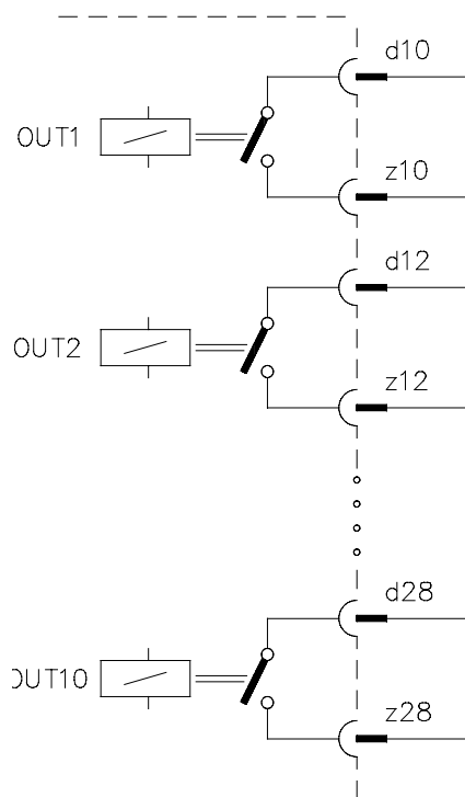
Figure 1 Schematic diagram for 10208/2/1 module
