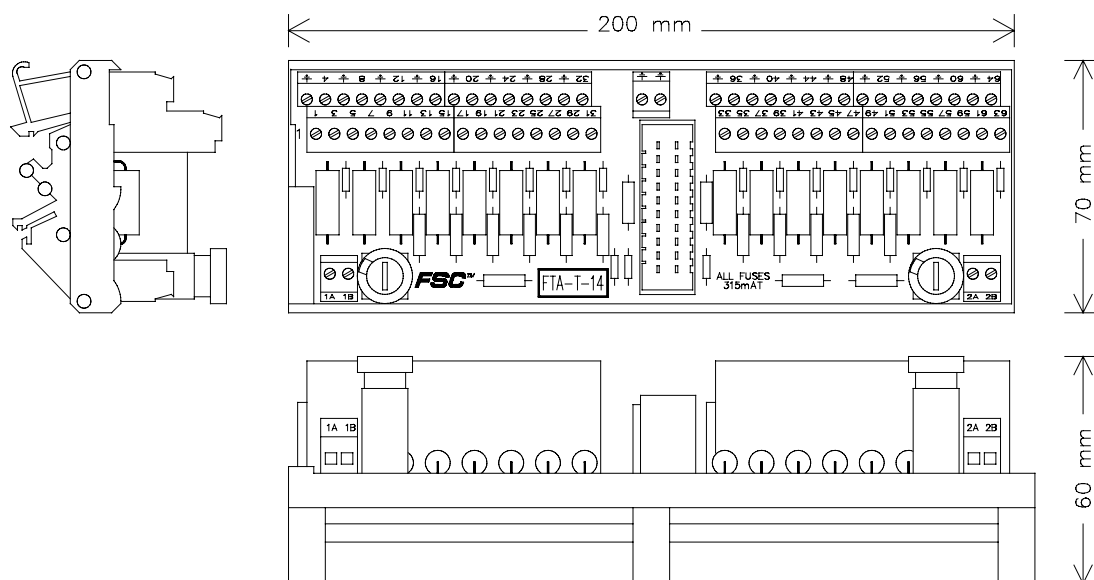
Figure 1 Mechanical layout
