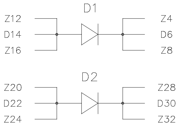
Figure 1 Schematic diagram of 10303/1/1 module
