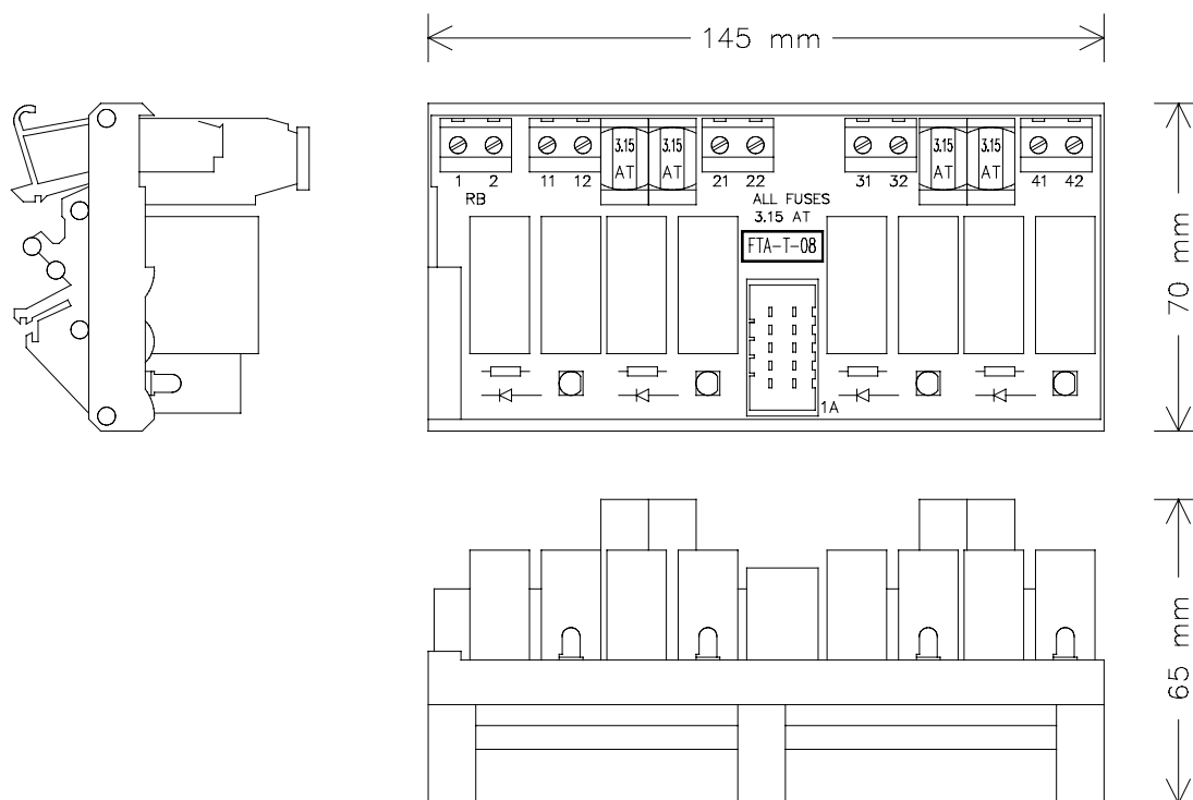
Figure 1 Mechanical layout
