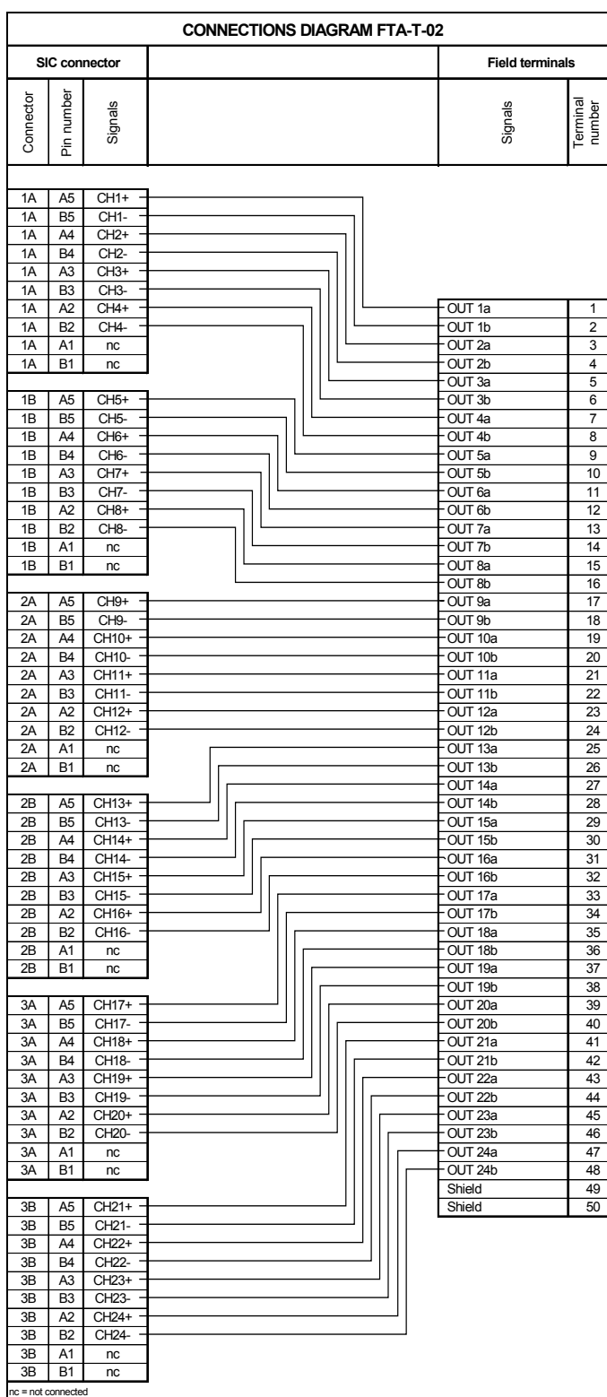
Figure 2 Connections diagram
