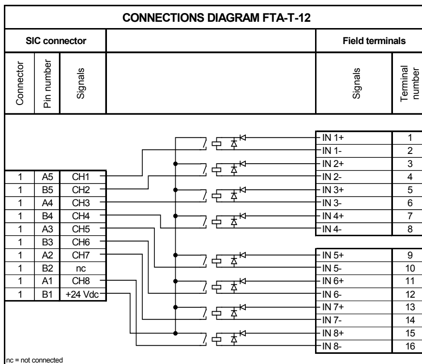
Figure 3 Connections diagram
