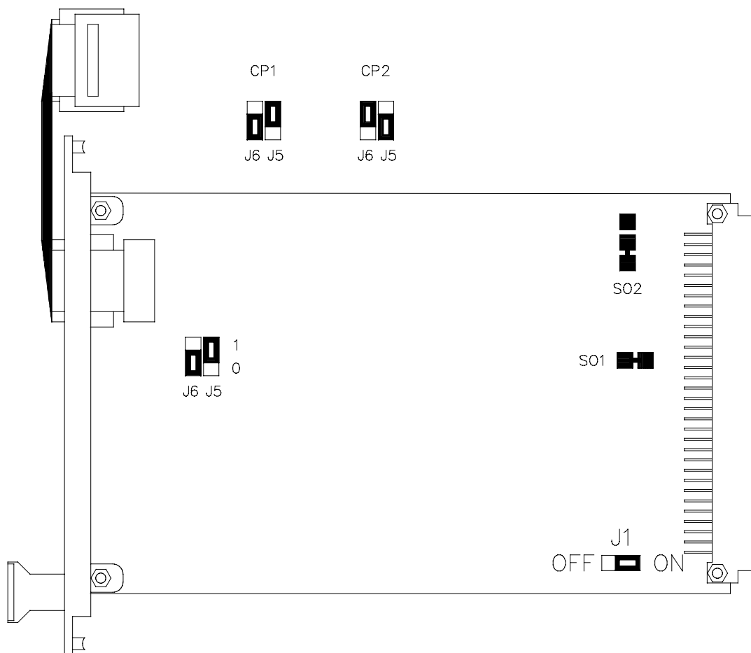
Figure 2 Jumper setting on 10007/1/1
