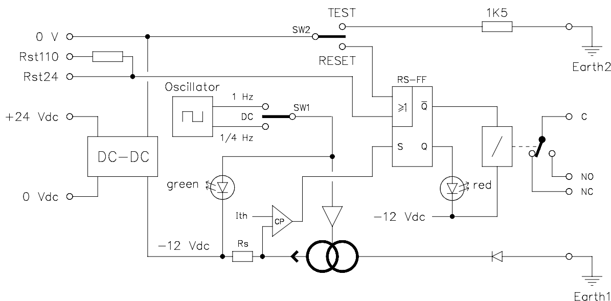
Figure 2 Block diagram of 10310/2/1 ELD
