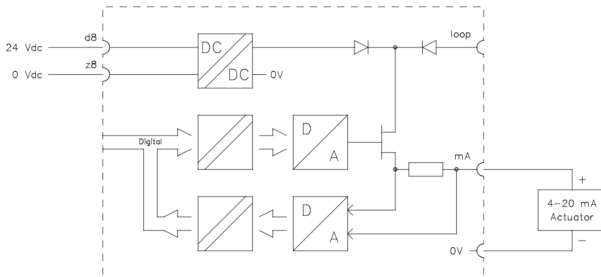
Figure 1 Schematic diagram for connection of the 10205/2/1 module as an active output
