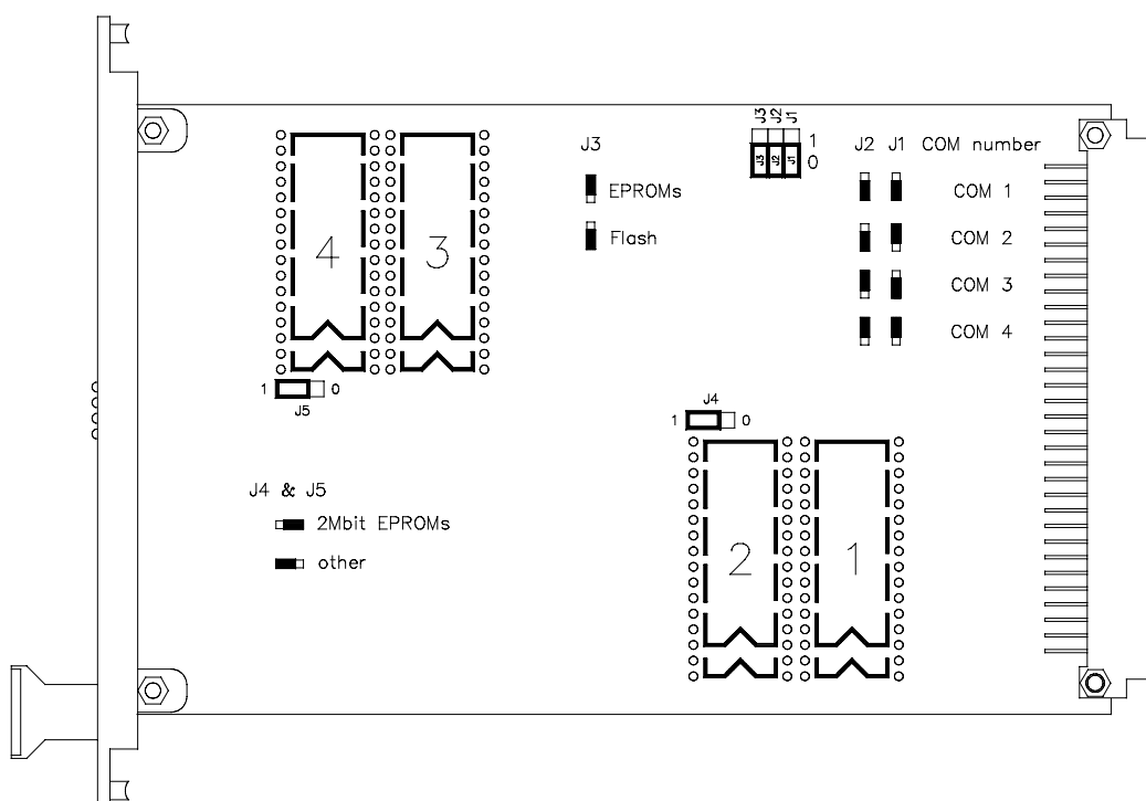
Figure 3 Location of jumpers and EPROM sockets on 10024/. main board
