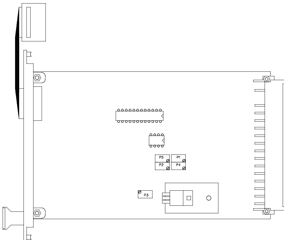
Figure 4 Location of potentiometers on 10102/2/1 module
