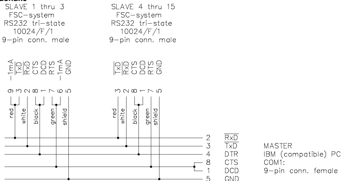
Figure 18 Connection between FSC system and FSC user station: 9-pin connector with hardware handshaking (using an F-interface)
