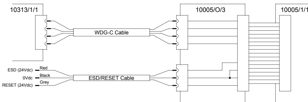
Figure 2 Schematic diagram
