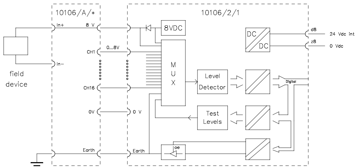
Figure 1 Schematic diagram for connection of inputs to 10106/2/1 module
