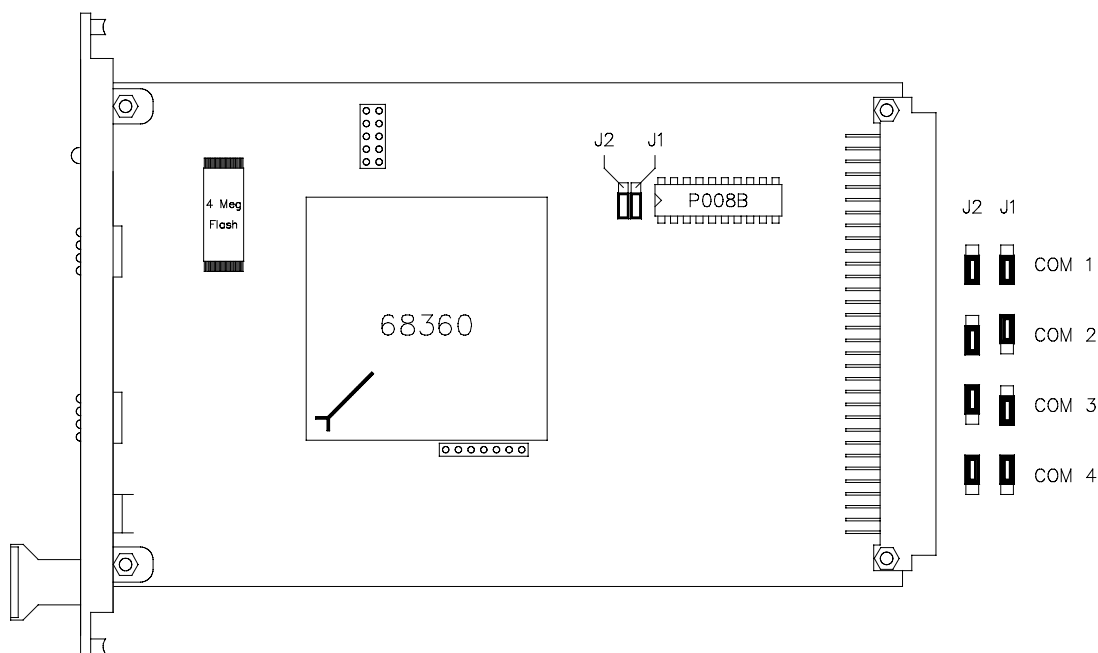
Figure 2 Jumper positions on 10018/E/1 & 10018/E/E main board
