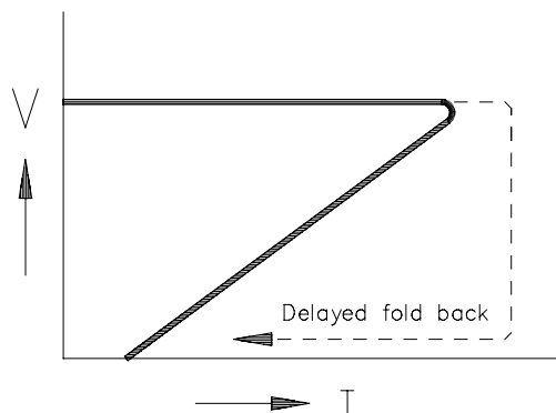
Figure 2 Delayed foldback
