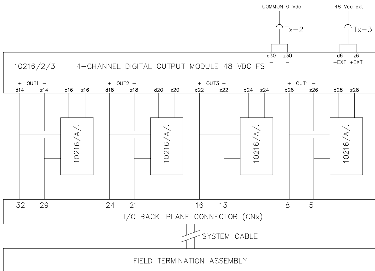
Figure 2 Connection example of 10216/2/3 module to FTA for both non-redundant and redundant I/O configurations
