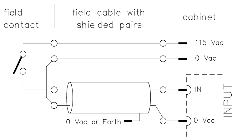
Figure 5 Field cable with shielded pairs
