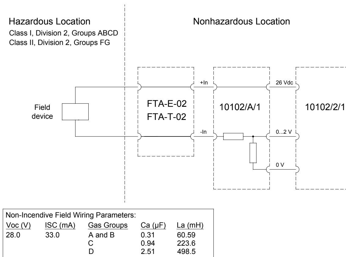
Figure 3 Connection of input in hazardous locations
