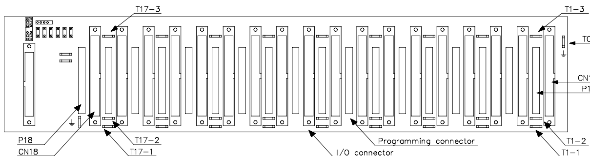
Figure 2 Back view
