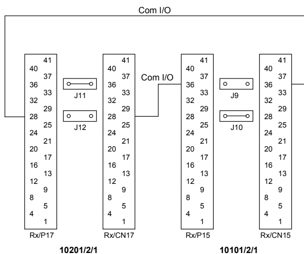
Figure 3 Example of 'Com I/O' configuration
