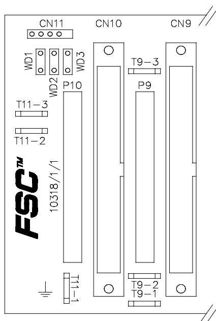
Figure 3 Back view detail
