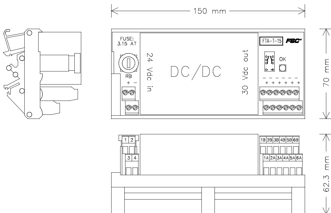
Figure 1 Mechanical layout
