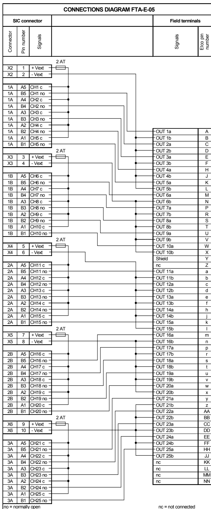
Figure 3 Connections diagram
