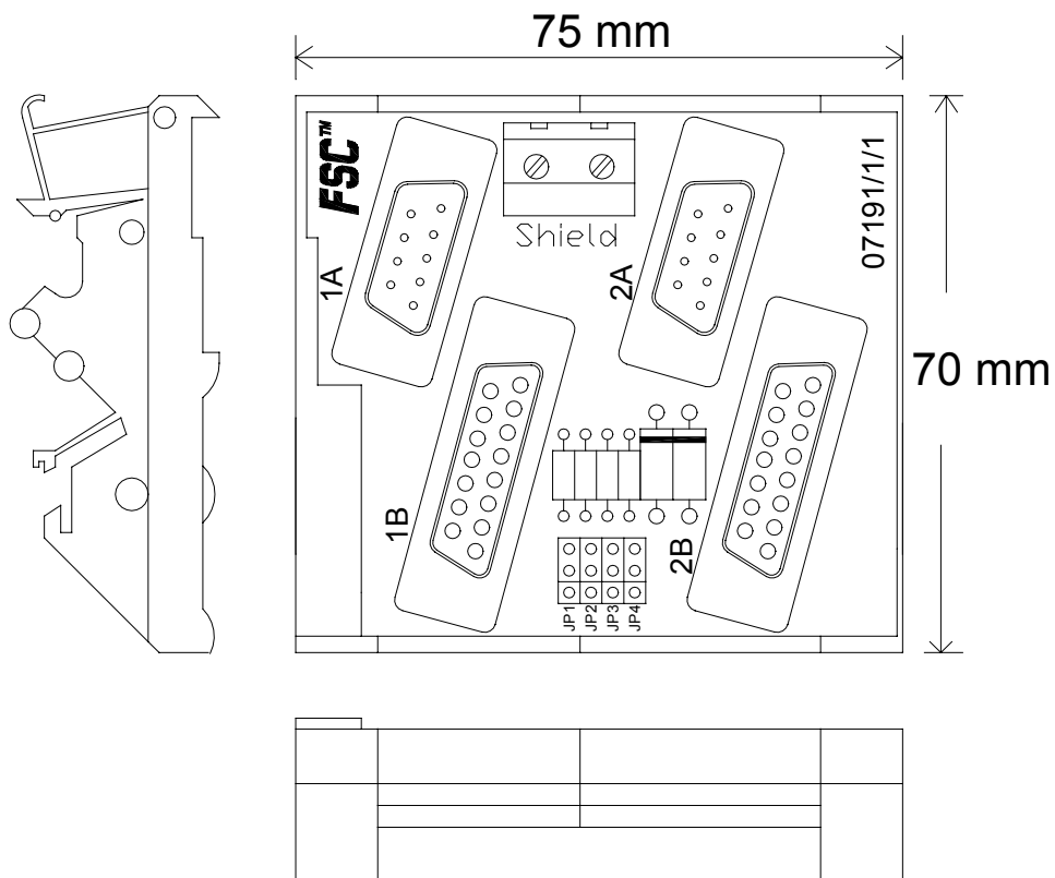
Figure 1 Top view
