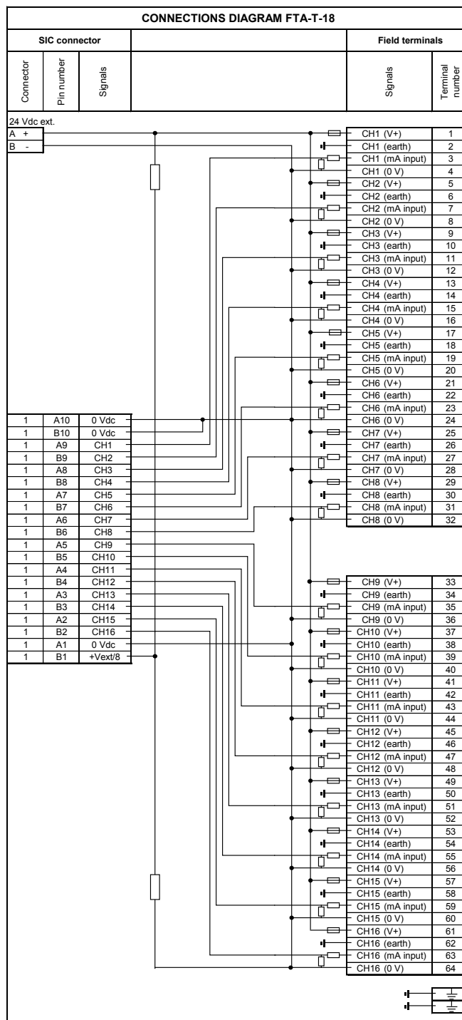
Figure 3 Connections diagram
