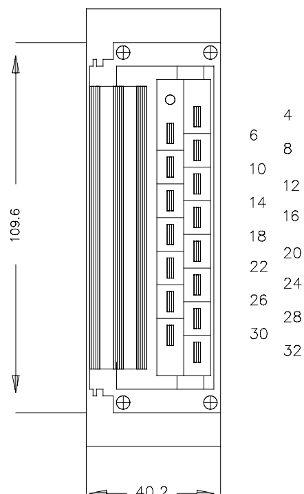
Figure 2 Back view
