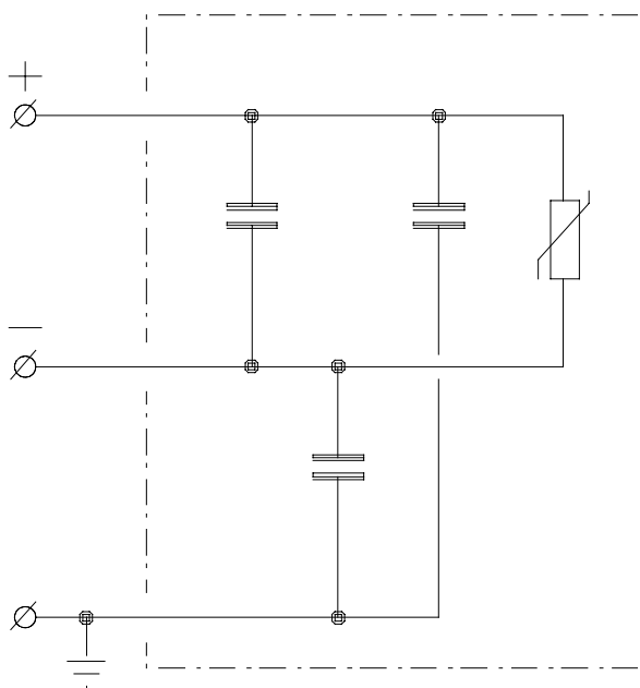
Figure 2 10306/1/. circuit
