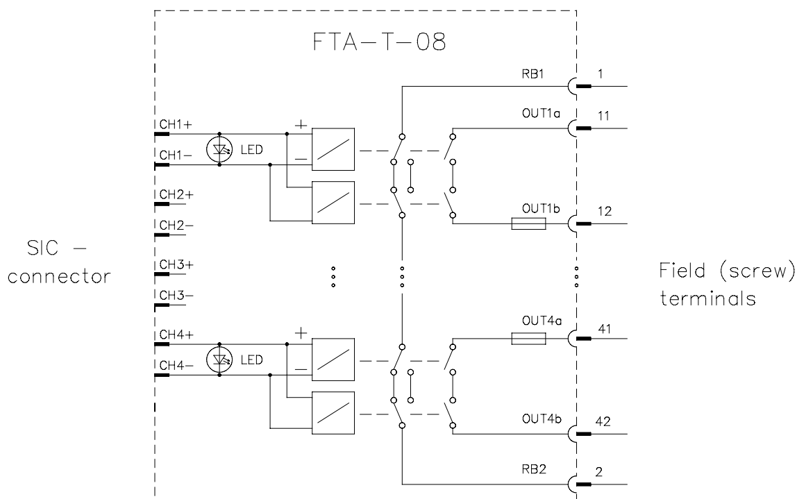
Figure 2 Schematic diagram
