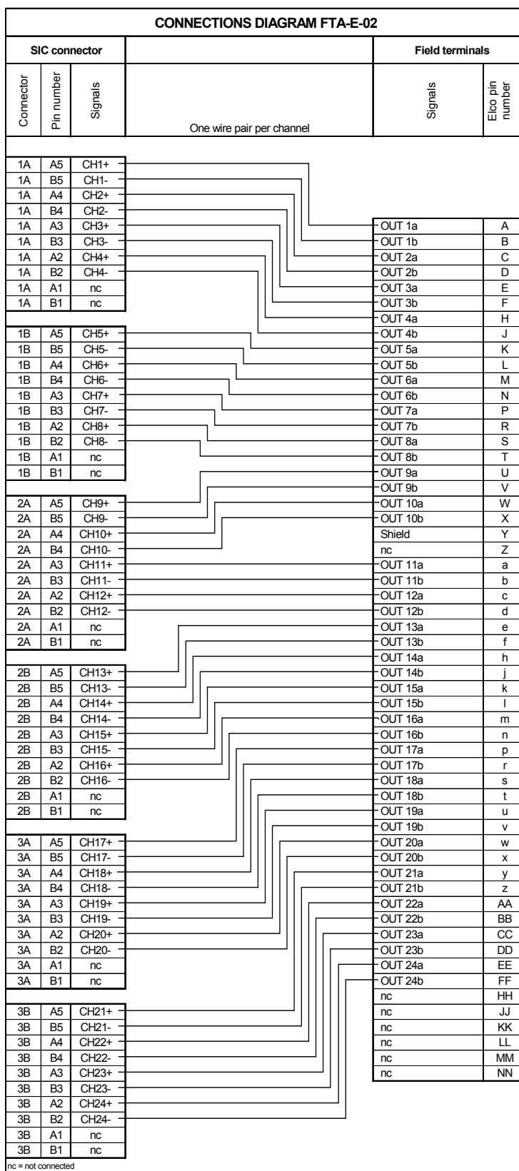
Figure 2 Connections diagram (one wire pair per channel)
