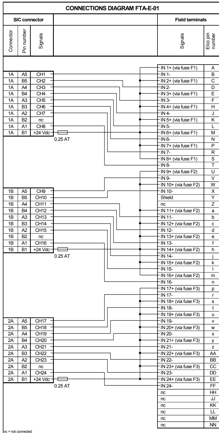
Figure 2 Connections diagram
