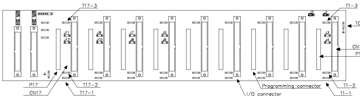
Figure 2 Back view
