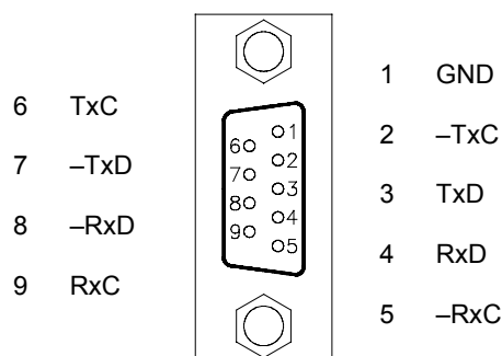
Figure 7 Front view of H-interface connector
