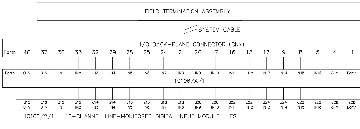
Figure 3 Connection example of 10106/2/1 module with signal converter 10106/A/1
