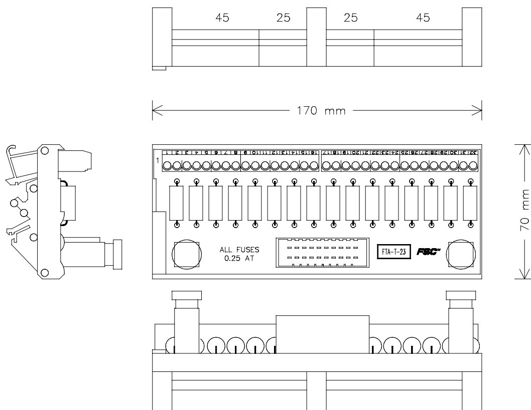
Figure 1 Mechanical layout
