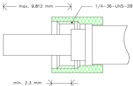
Figure 5 Cable connector type FSMA
