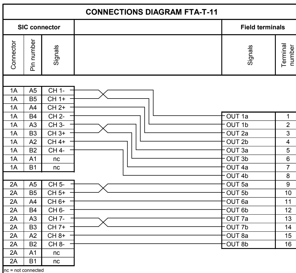
Figure 2 Connections diagram
