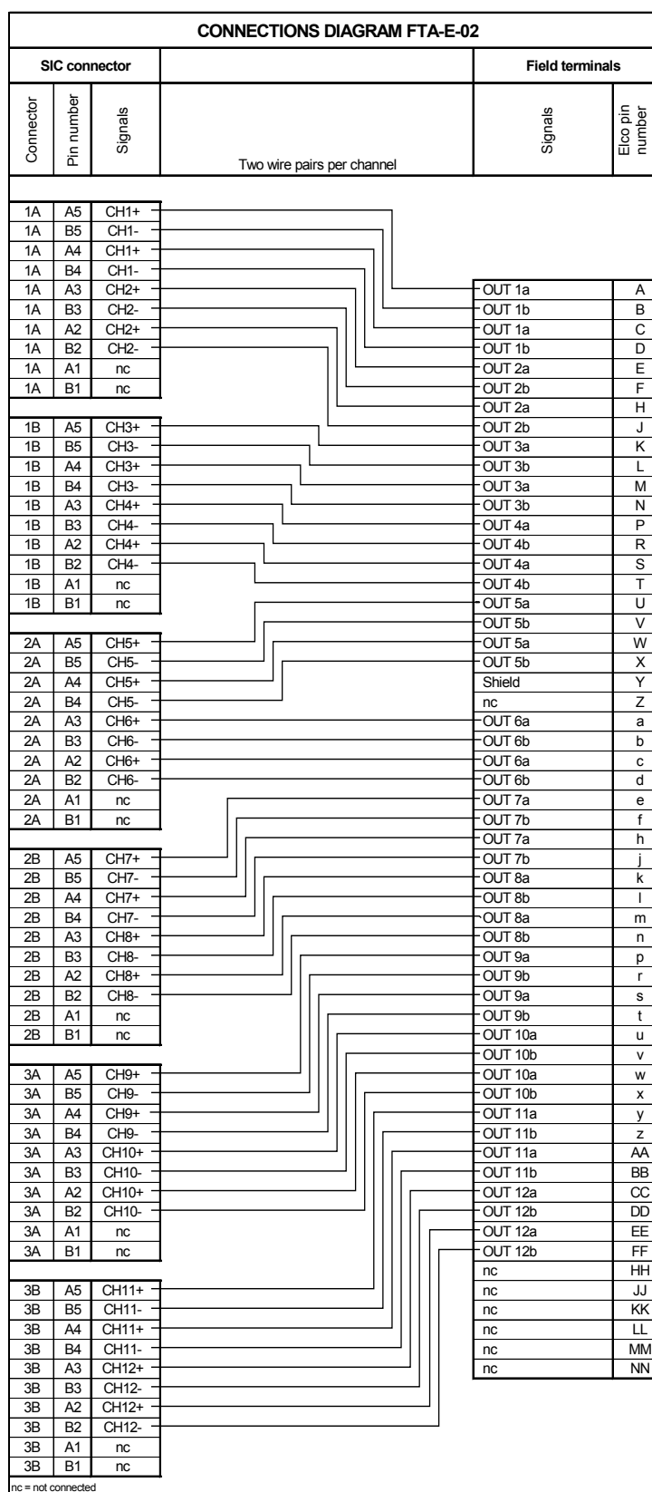
Figure 3 Connections diagram (two wire pairs per channel)
