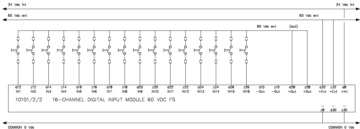
Figure 3 I/O connection example of 10101/2/2 module for non-redundant I/O configurations
