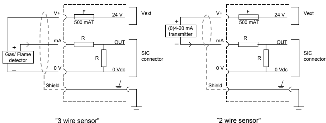
Figure 2 Schematic diagram for connecting a transmitter
