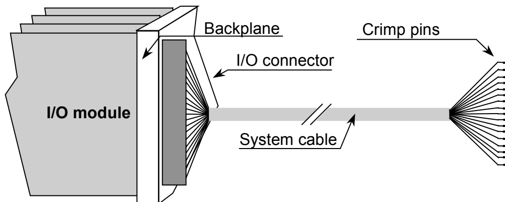
Figure 1 Principle of SIC-P connection method
