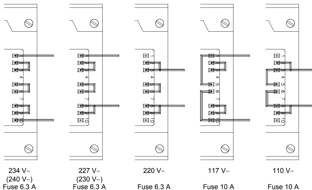
Figure 4 Transformer connections
