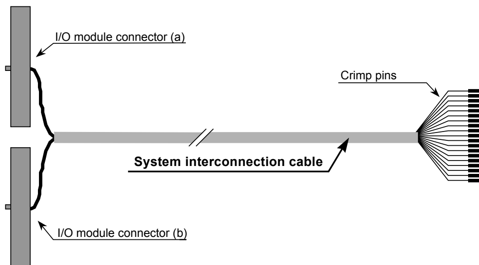
Figure 4 SIC-P cable, layout type 3
