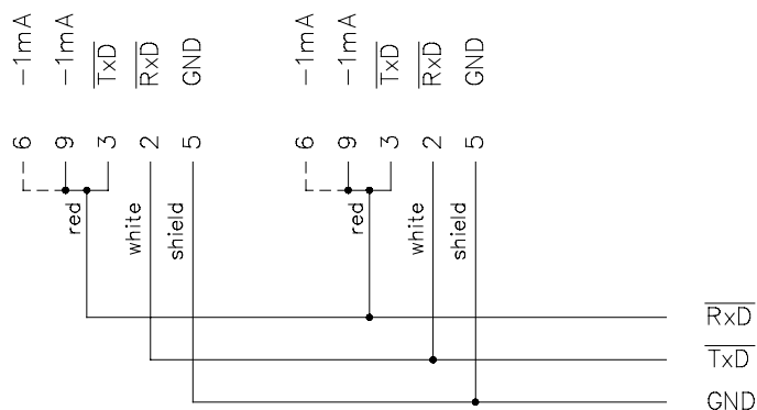
Figure 21 Connection between FSC system and DCS: without hardware handshaking, using an F-interface (RS-232)
