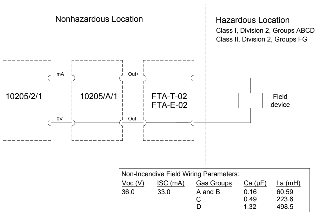
Figure 5 Connection of output in hazardous locations
