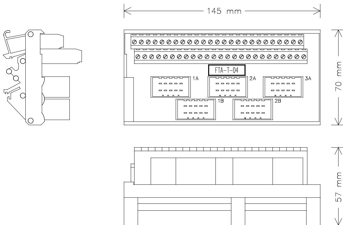
Figure 1 Mechanical layout
