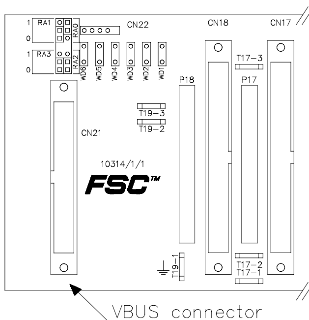
Figure 3 Back view detail
