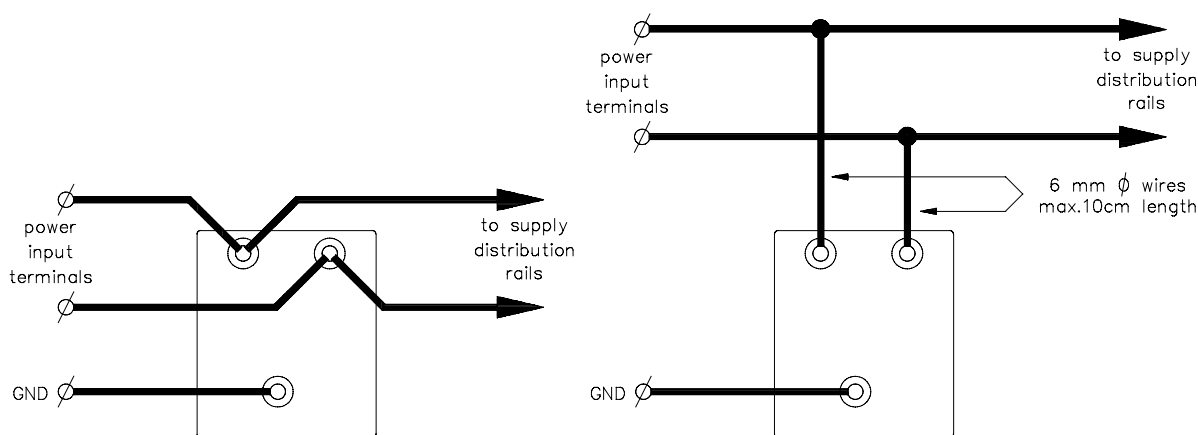
Figure 3 Wiring examples for 10306/1/. modules
