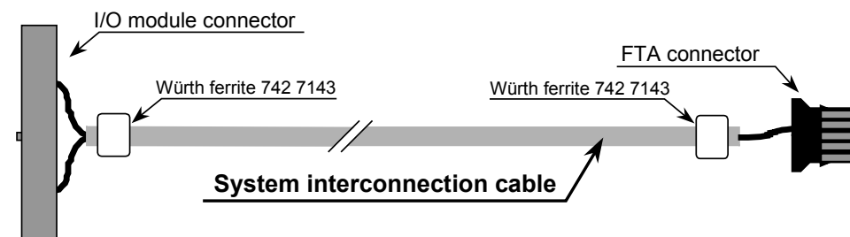
Figure 4 SIC-C cable, layout type 3
