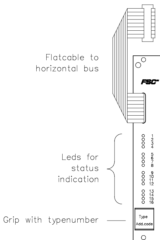
Figure 1 Front of a digital output module
