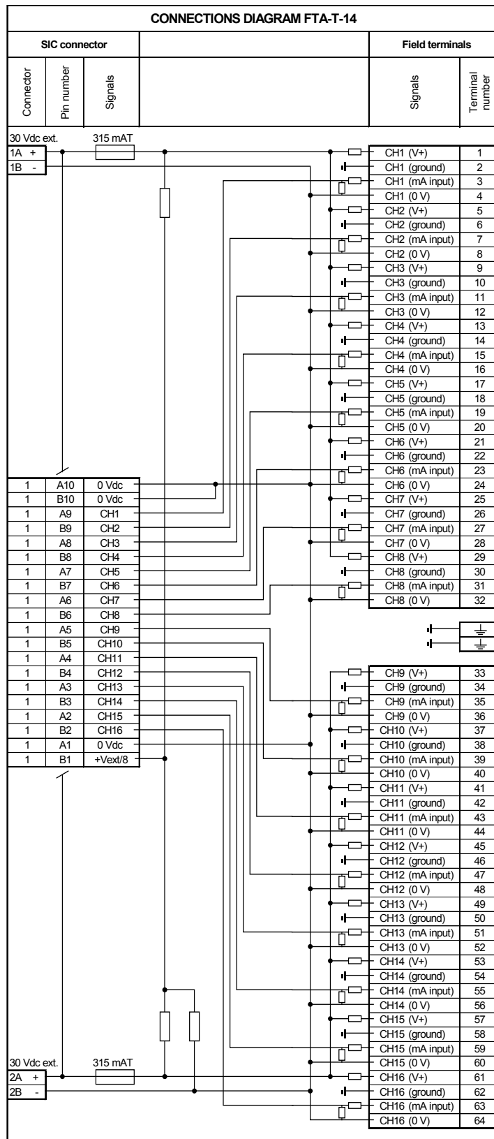
Figure 5 Connections diagram
