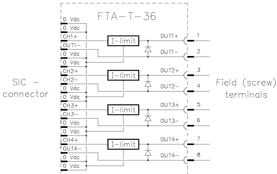
Figure 2 Schematic diagram
