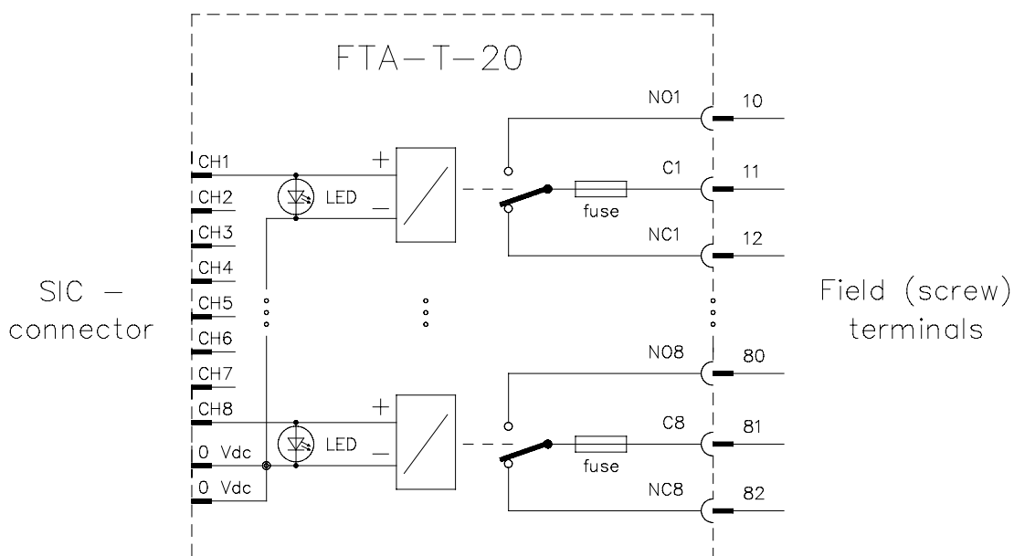
Figure 2 Schematic diagram
