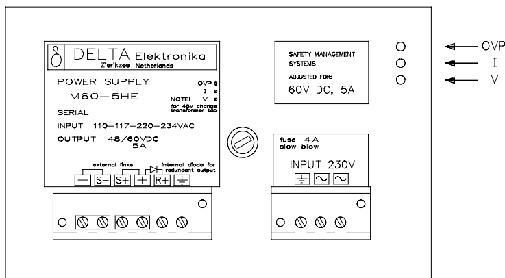
Figure 1 Back view
