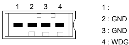
Figure 7 Pin connections of 'OUT/IN' connectors
