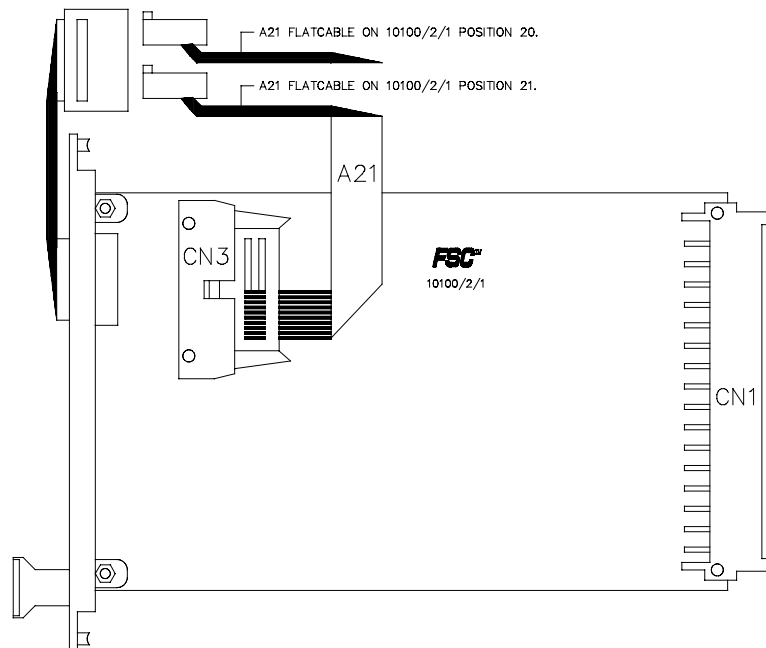
Figure 3 Schematic diagram for flatcable routing from the HBD (redundant I/O with one rack per HBD)
