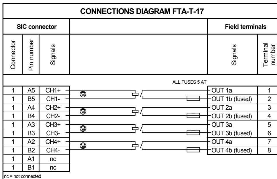
Figure 3 Connections diagram
