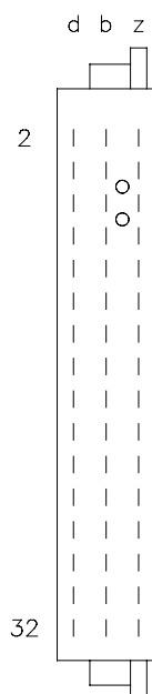
Figure 1 Back view of 10100/2/1 connector
