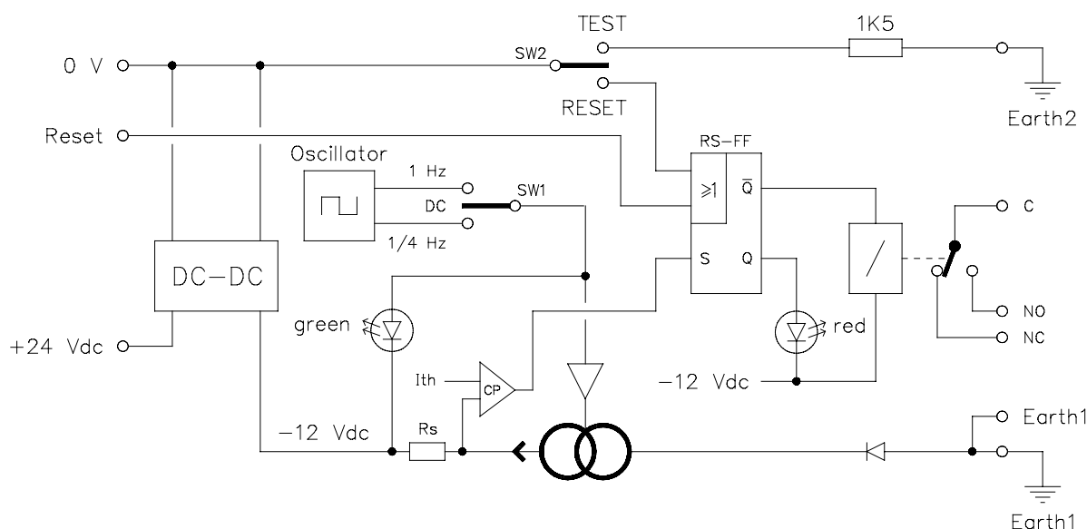
Figure 2 Block diagram of 10310/1/1 ELD
