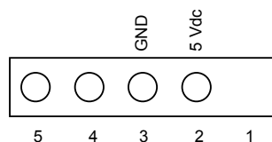
Figure 2 Connector CN3 (detail)
