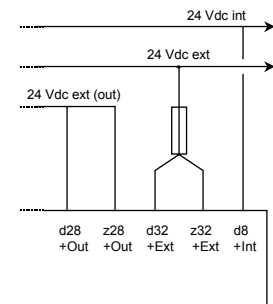
Figure 3 I/O connection example of 10101/2/1 module for non-redundant I/O configurations
