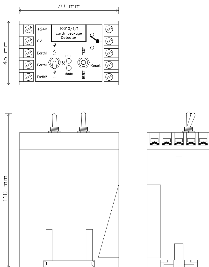
Figure 1 Module layout
