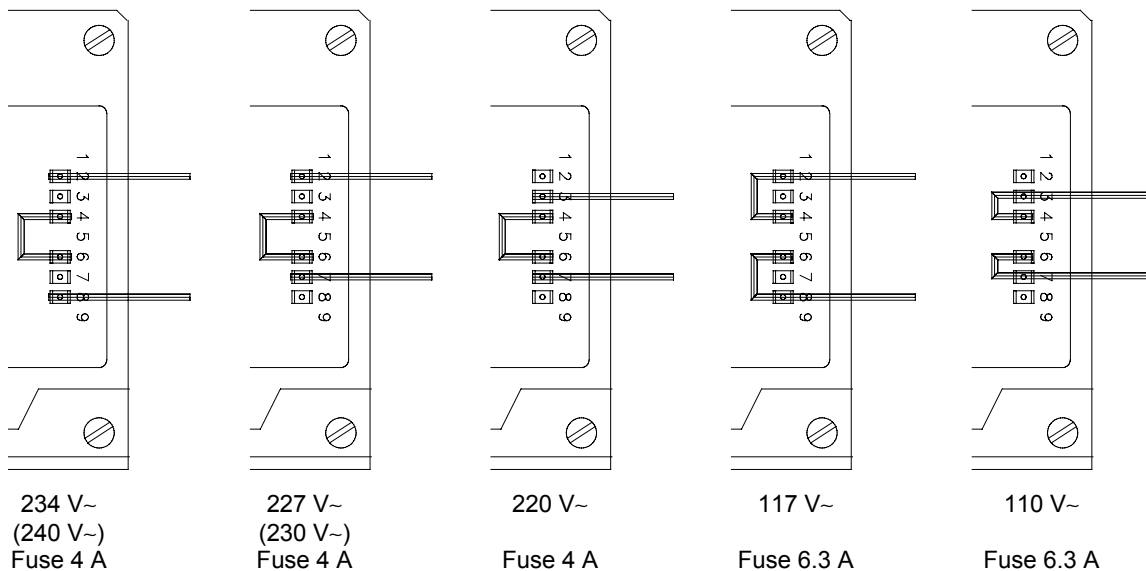
Figure 4 Transformer connections
