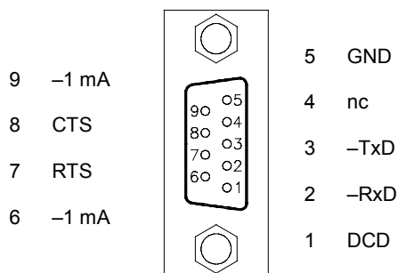
Figure 4 Front view of F-interface connector
