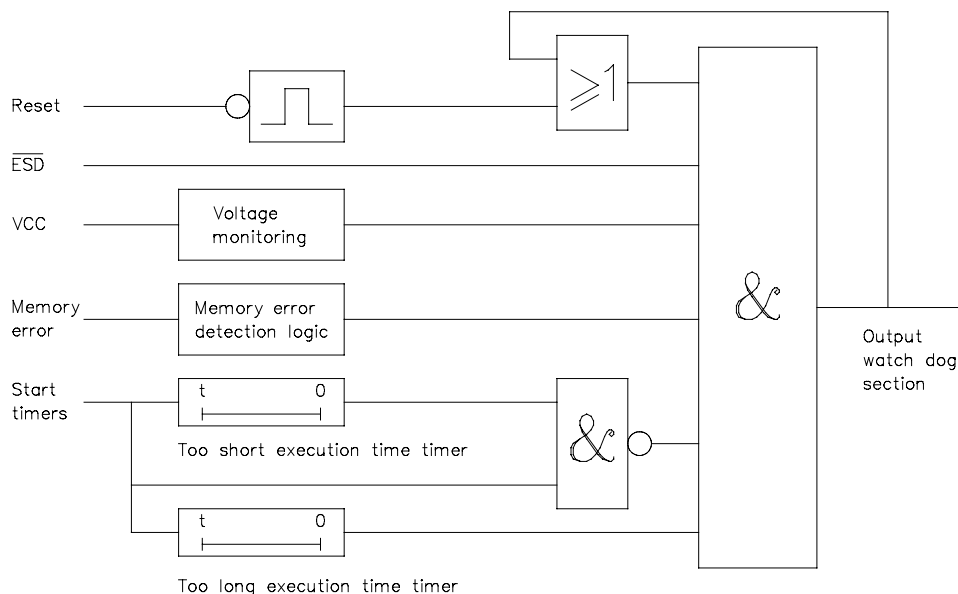
Figure 1 Watchdog section
