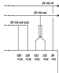
Figure 3 I/O connection example of 10101/2/2 module for non-redundant I/O configurations
