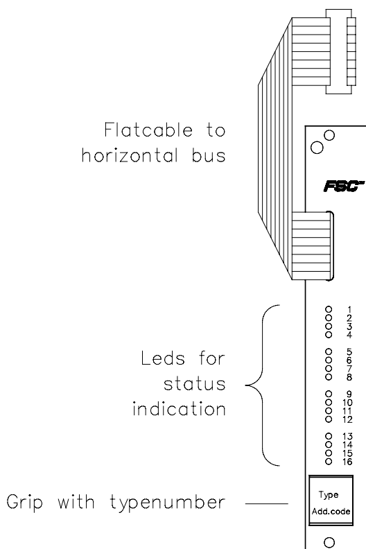
Figure 1 Front of a digital input module
