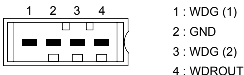
Figure 6 Pin connections of 'WDR', 'WDR-1' and 'WDR-2' connectors
