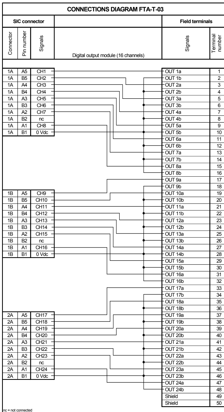
Figure 2 Connections diagram (for 16-channel digital output modules)
