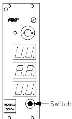
Figure 1 Front view
