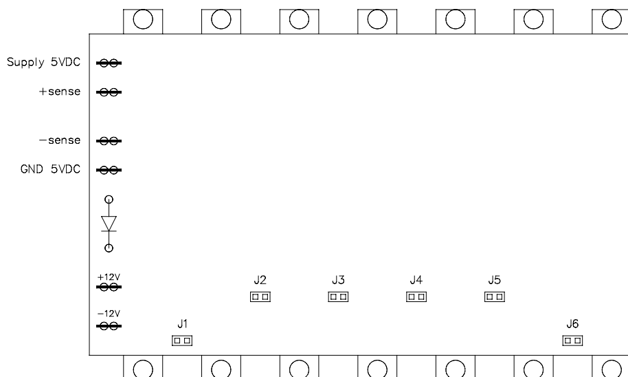
Figure 2 System bus (7-SBUS) back view with jumpers and faston terminations
