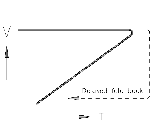
Figure 2 Delayed foldback
