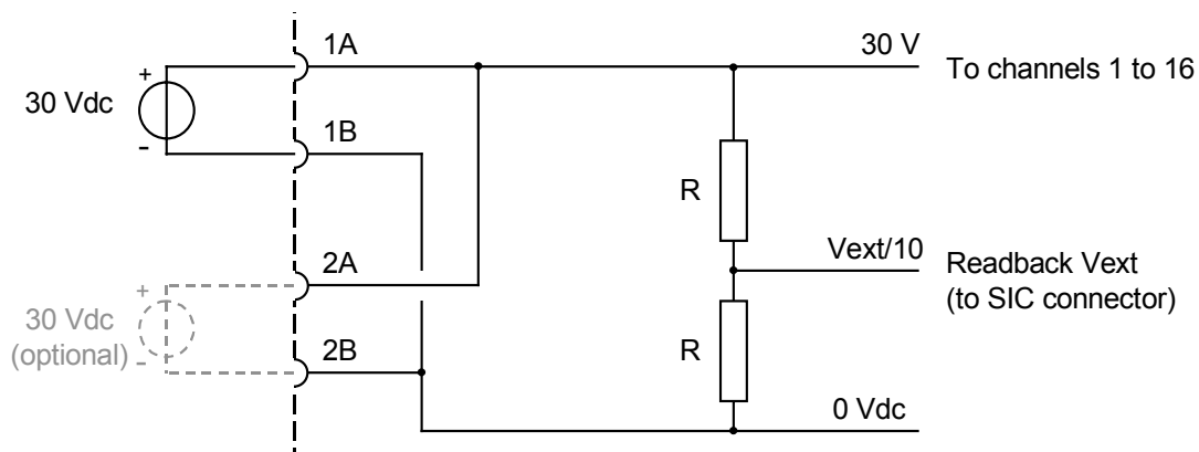
Figure 3 Schematic diagram for power distribution with monitoring
