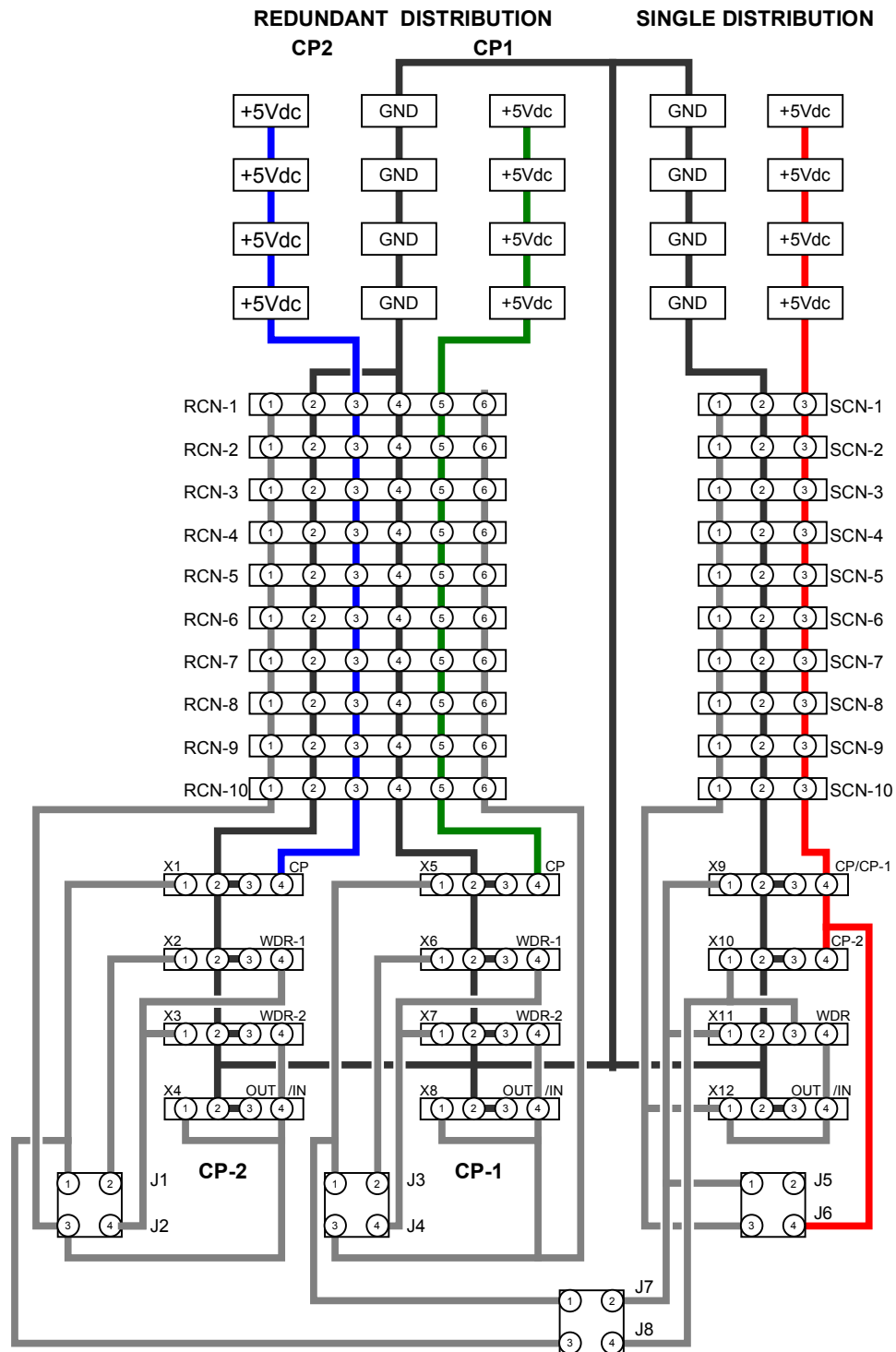
Figure 2 Connection diagram
