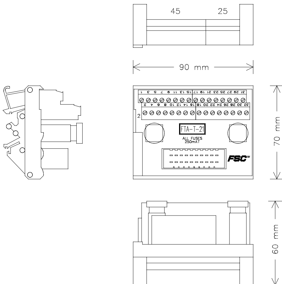
Figure 1 Mechanical layout
