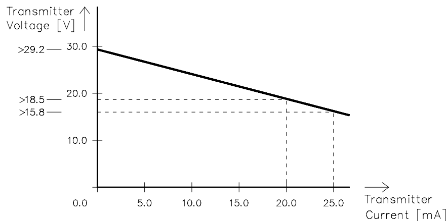
Figure 3 Transmitter voltage for passive transmitters
