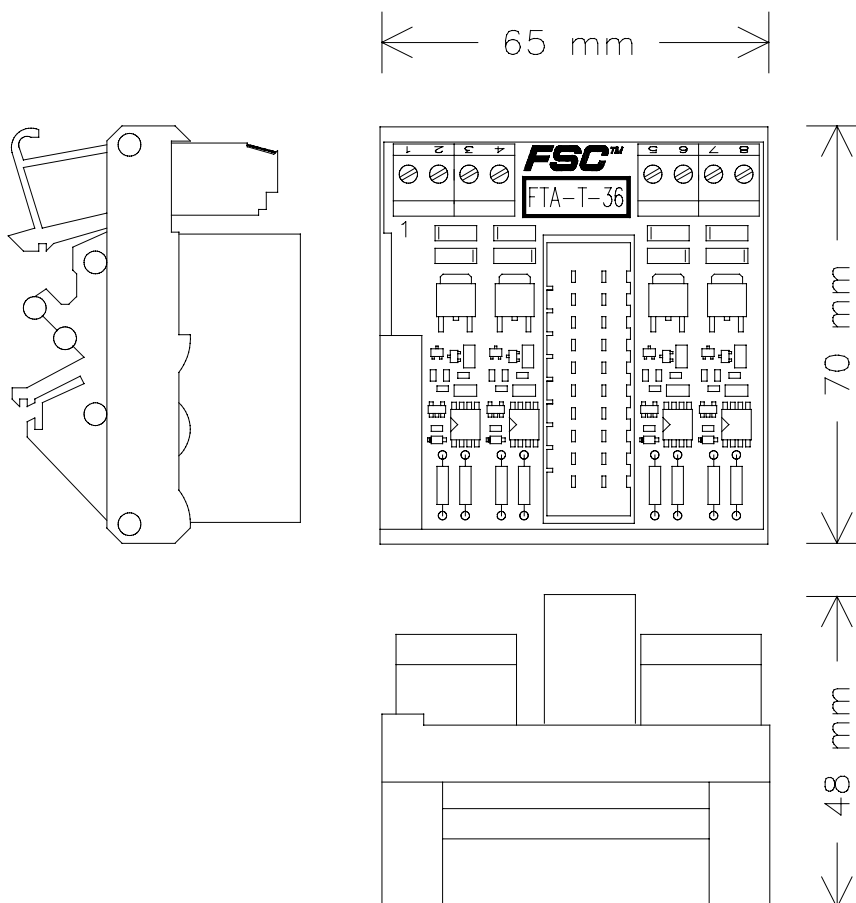
Figure 1 Mechanical layout
