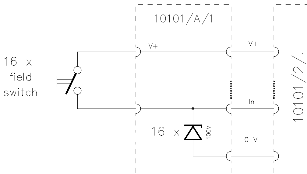
Figure 1 Schematic diagram
