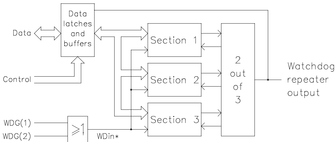
Figure 2 Block diagram for the watchdog repeater module
