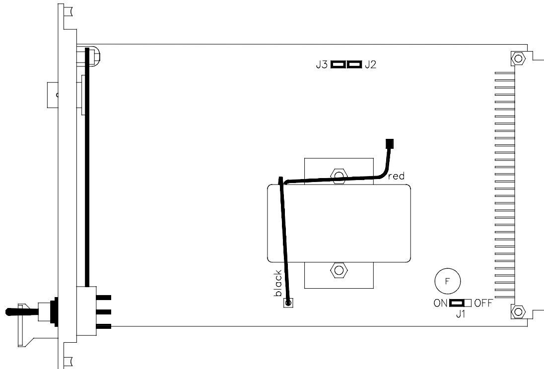
Figure 2 Jumper settings on 10006/2/2 module (08905 shown)
