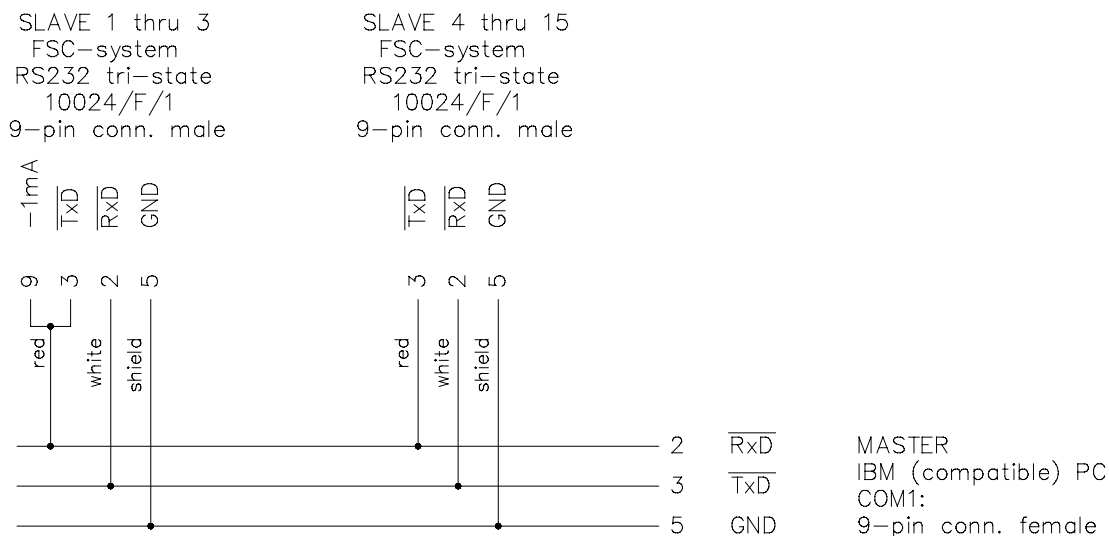
Figure 17 Connection between FSC system and FSC user station: 9-pin connector without hardware handshake (using an F-interface)
