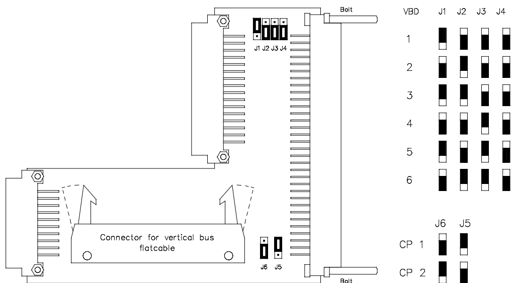
Figure 3 Jumper setting on 10001/A/1 module for CP 1, VBD 1
