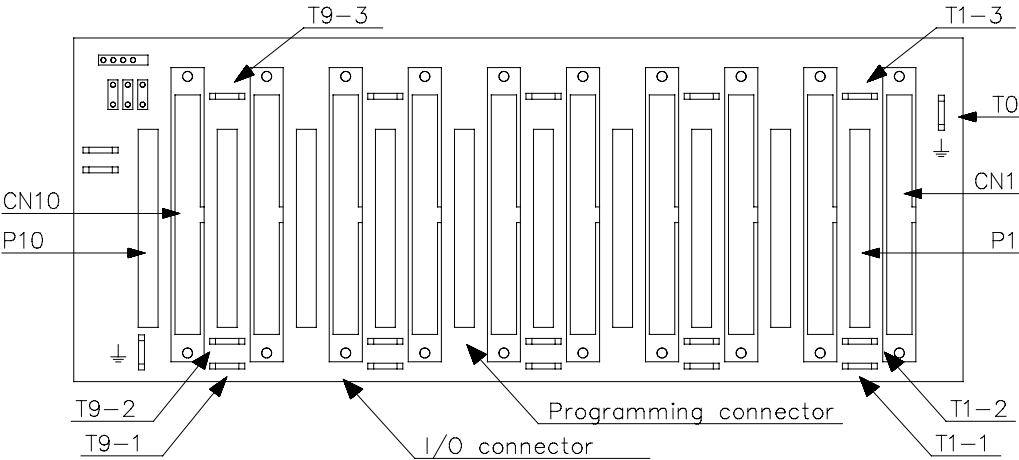
Figure 2 Back view
