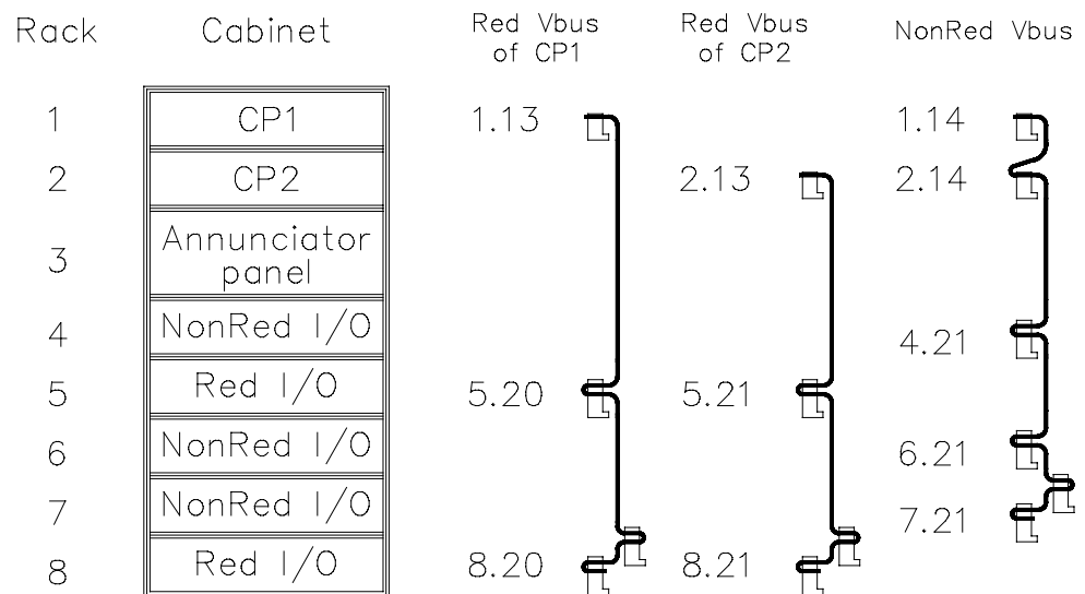
Figure 4 V-Buses example 4
