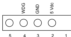
Figure 4 Connector CN11 (detail)
