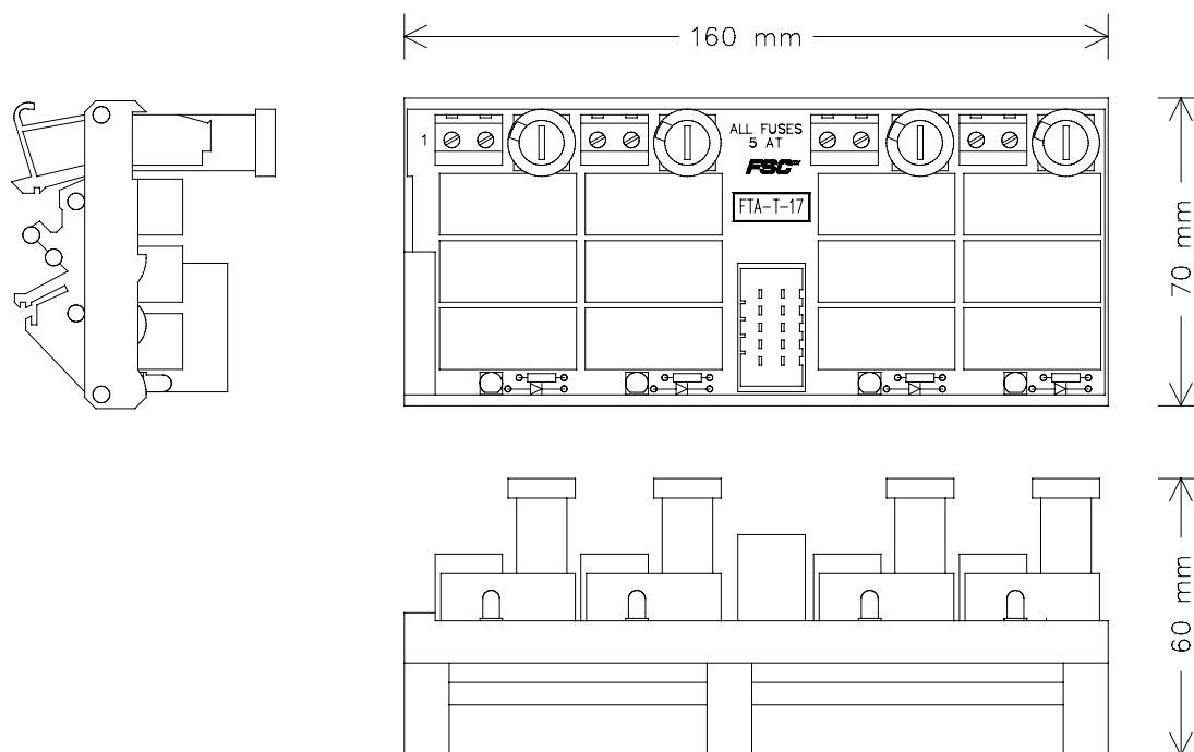
Figure 1 Mechanical layout
