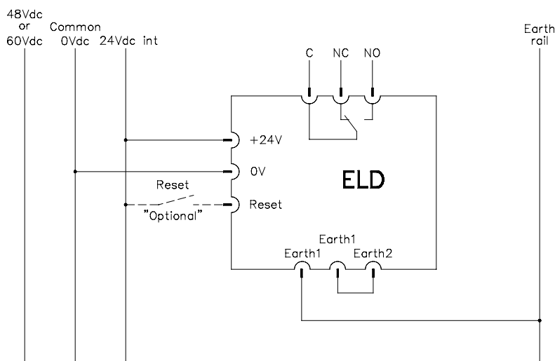
Figure 4 ELD with single earth wire
