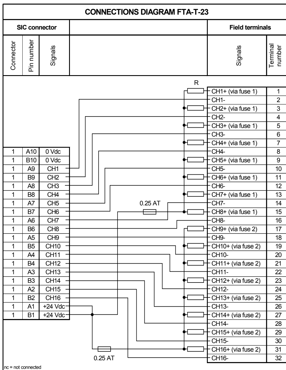
Figure 2 Connections diagram
