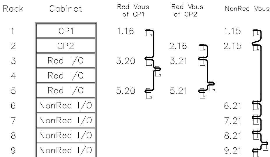
Figure 2 V-Buses example 2
