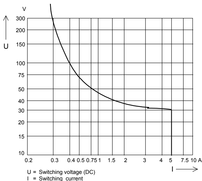
Figure 4 Maximum DC switched power curve for FTA-T-20 module
