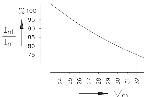
Figure 3 Maximum current derating vs. expected maximum supply voltage
