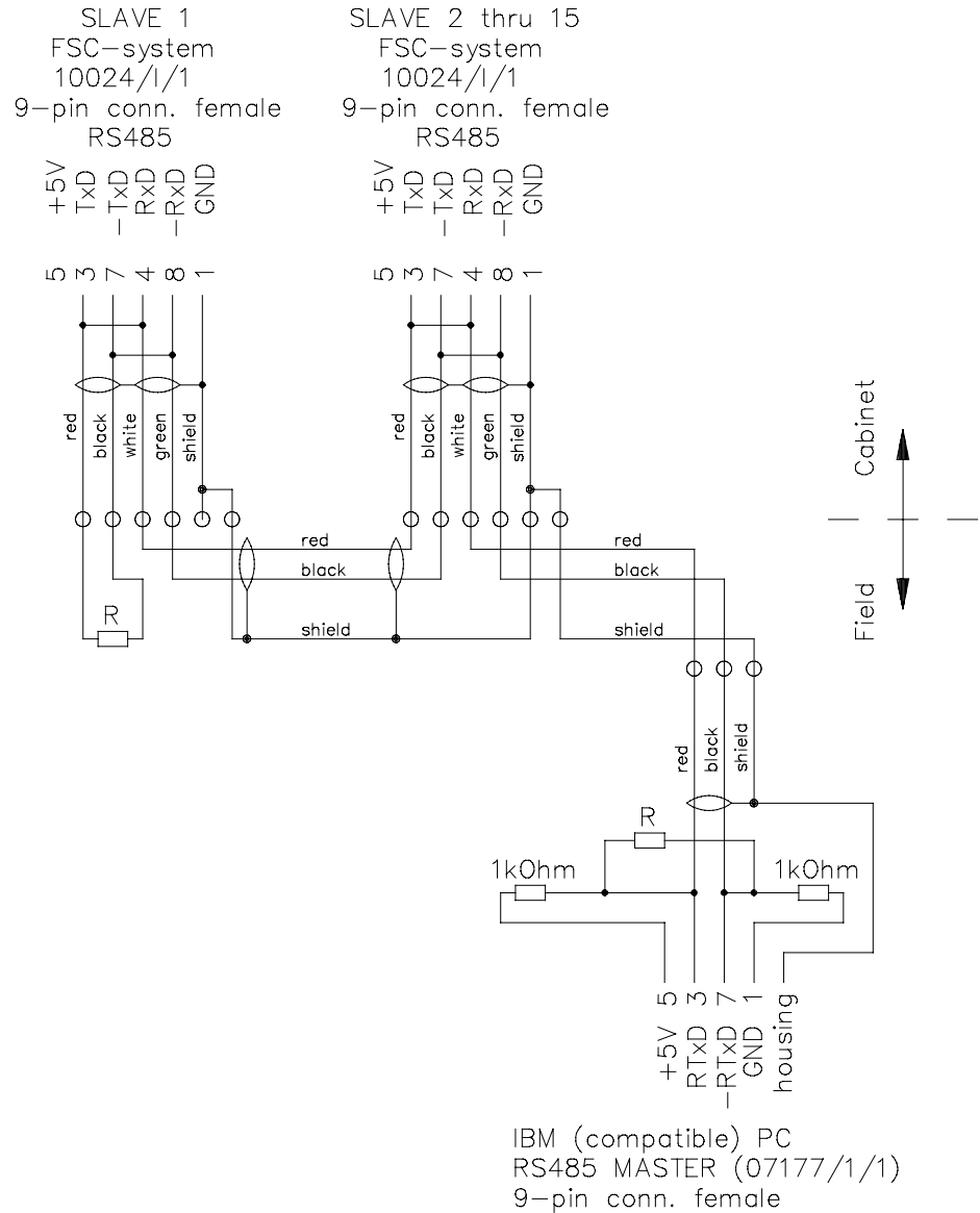
Figure 19 Connection between FSC system and FSC user station: simplex communication (using an I-interface)
