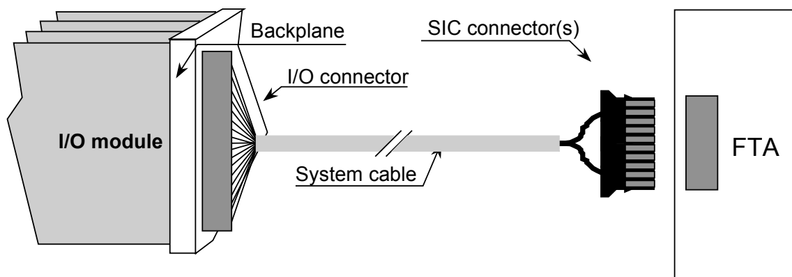
Figure 1 Principle of SIC-C connection method
