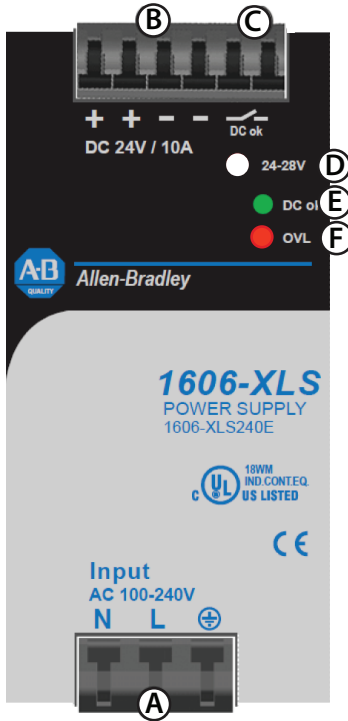
Fig. 13-1 Front side
