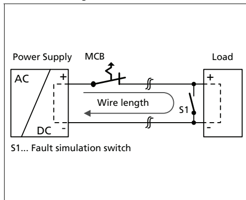
Fig. 23-5 Test circuit
