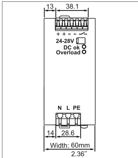
Fig. 22-1 Front view
