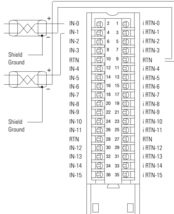
1756-IF16, 1756-IF16K Single-ended Voltage
