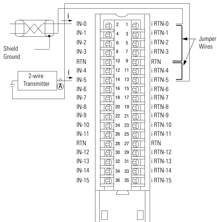
1756-IF16, 1756-IF16K Single-ended Current
