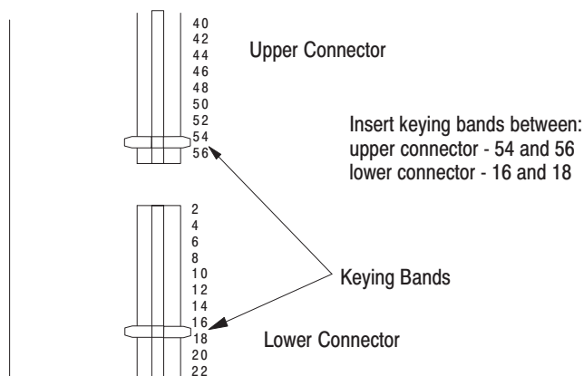
Figure 2.1 Keying Diagram
