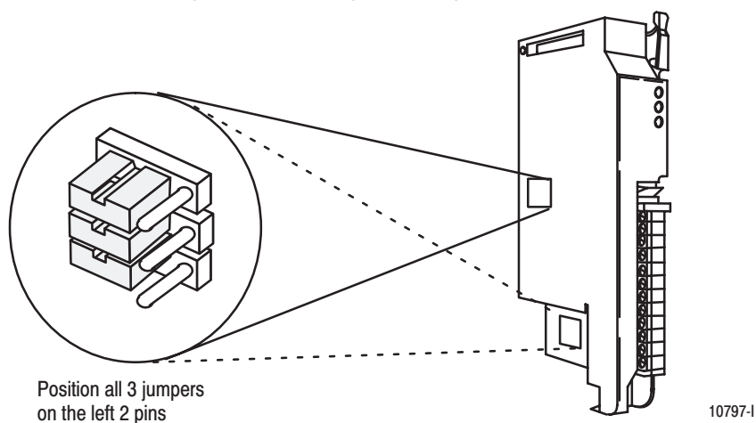
Figure 2.2 Setting the Module Configuration Plug
