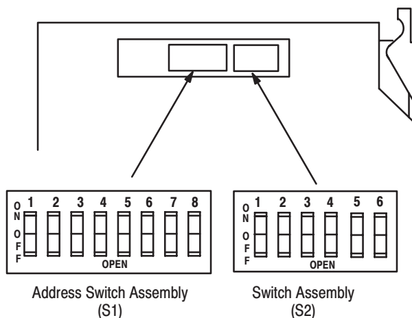
Figure 2.3 S1 and S2 Switch Assembly Locations
