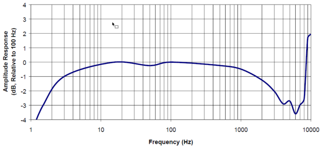
Figure 3: Typical Amplitude Response
