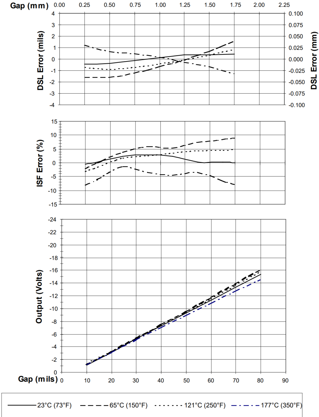
Figure 4: Typical 3300 NSv Probe + 1 m Cable @ High Temperature (Proximito Sensor + 4 m of Extension Cable @ 25°C)
