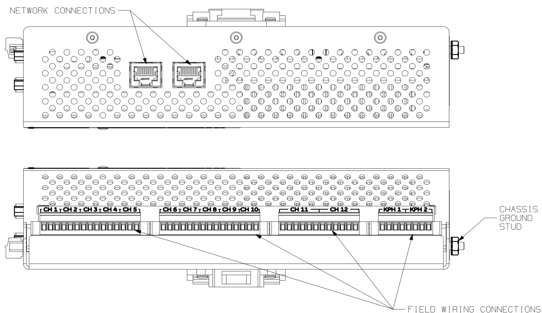
Figure 3: 60M100 Monitor Top and Bottom Views
