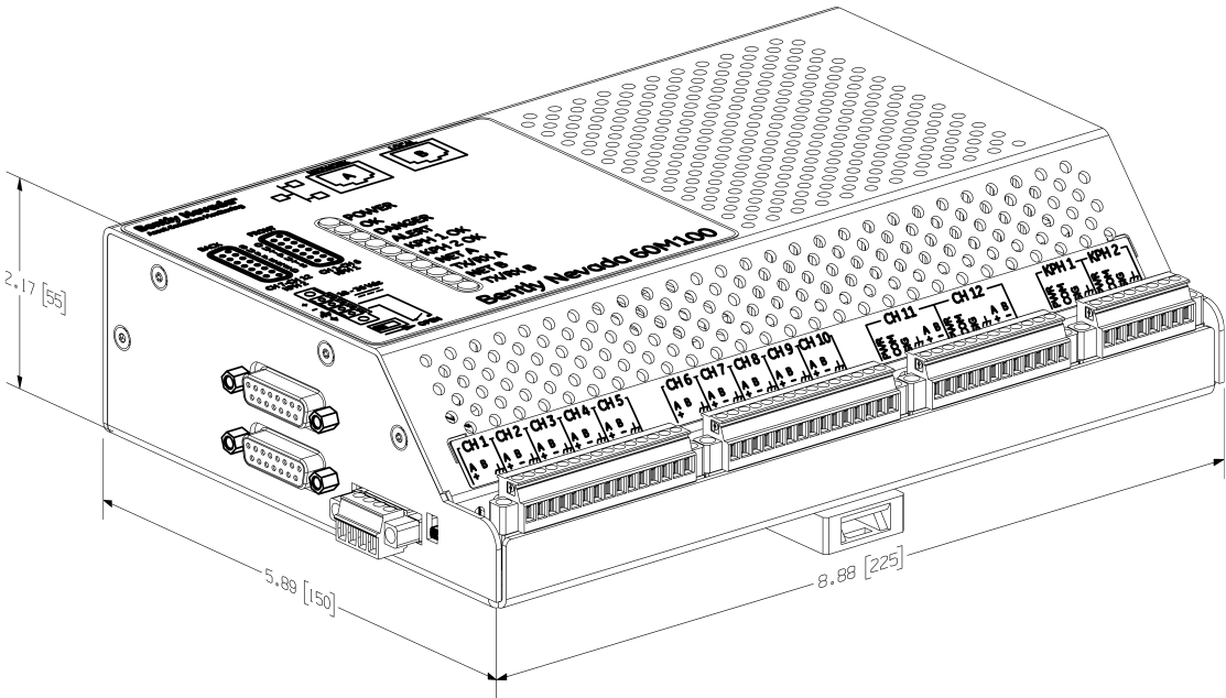
Figure 1: 60M100 Monitor Overall Dimensions
