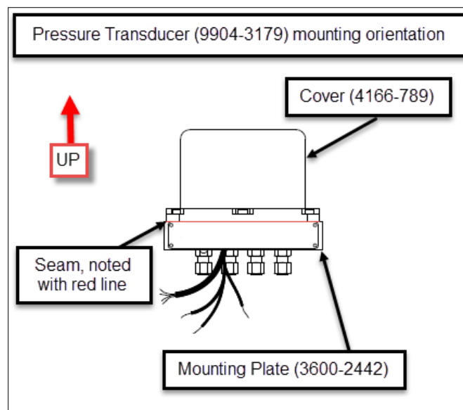
Figure R-1. Pressure Transducer Assembly Mounting Orientation
