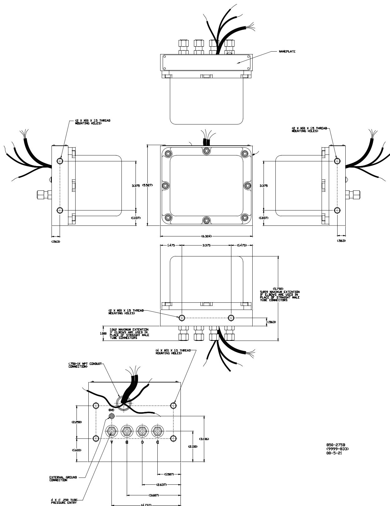
Figure 2-1. Outline Drawing of Pressure Transducer Manifold
