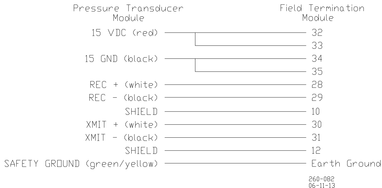
Figure 2-3. Wiring Schematic for Interface Module Port #2
