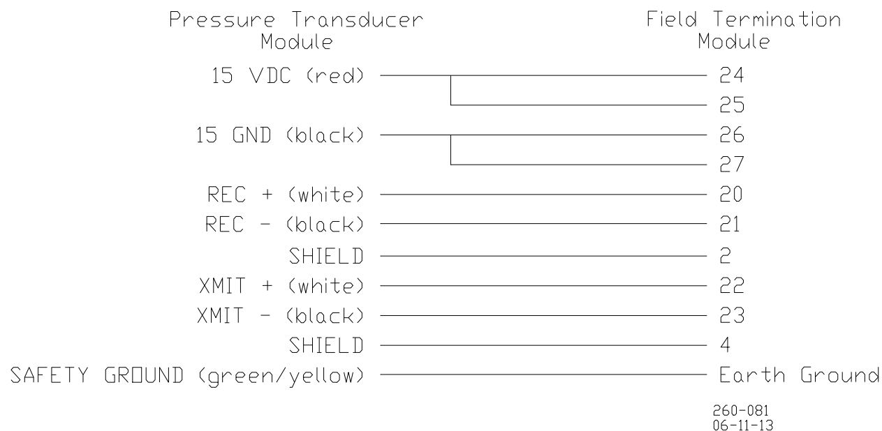
Figure 2-2. Wiring Schematic for Interface Module Port #1
