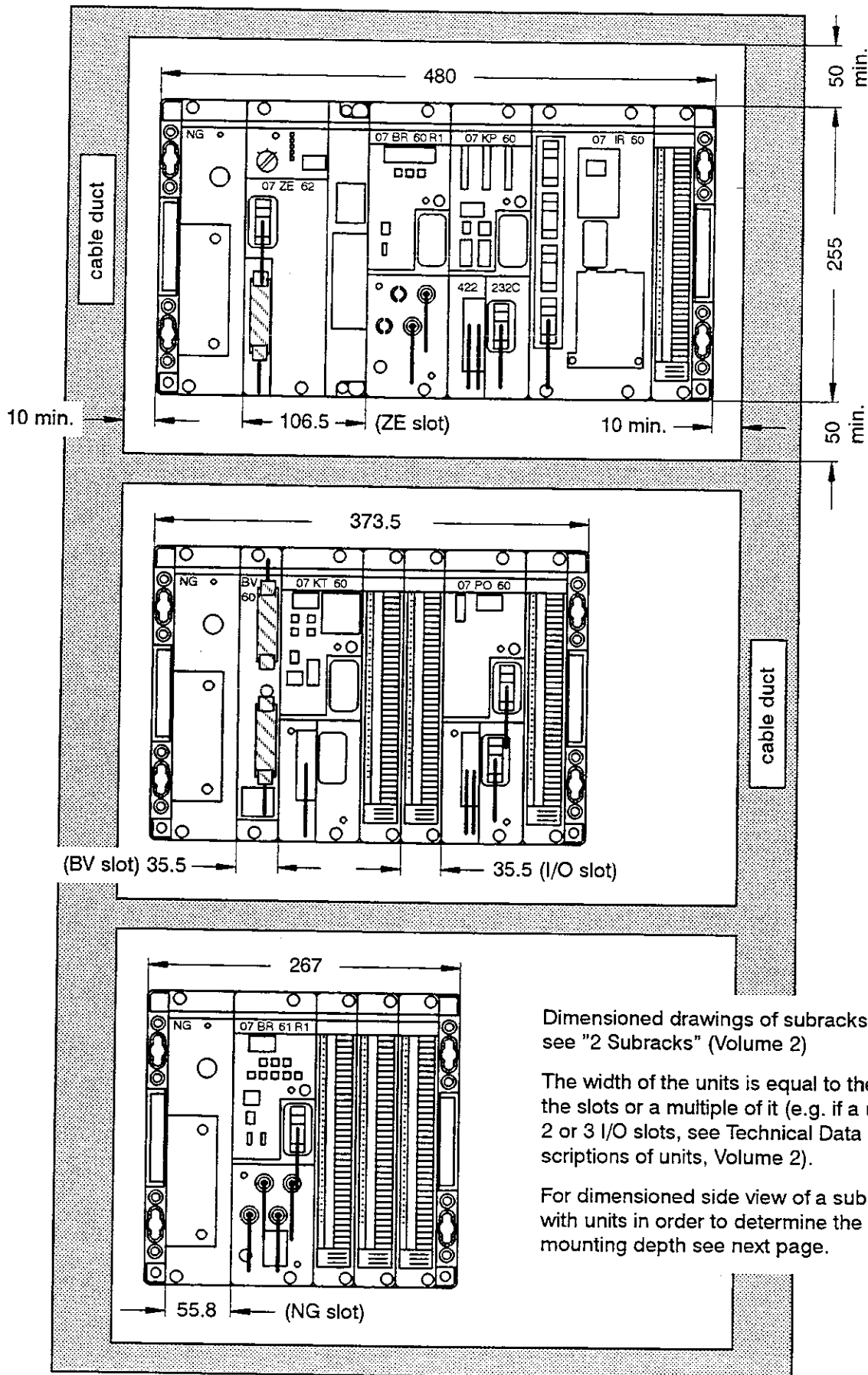
Fig. 2.1: Mounting dimensions of ABB Procontic T200
