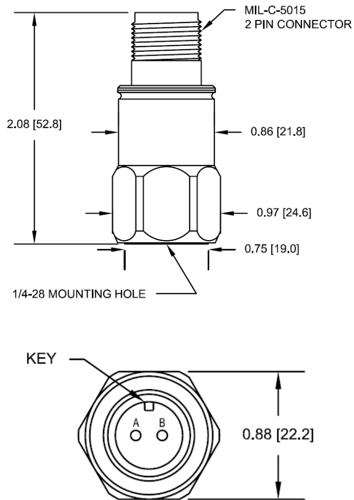
Figure 3: AP3500T2-Z1 dimensions
