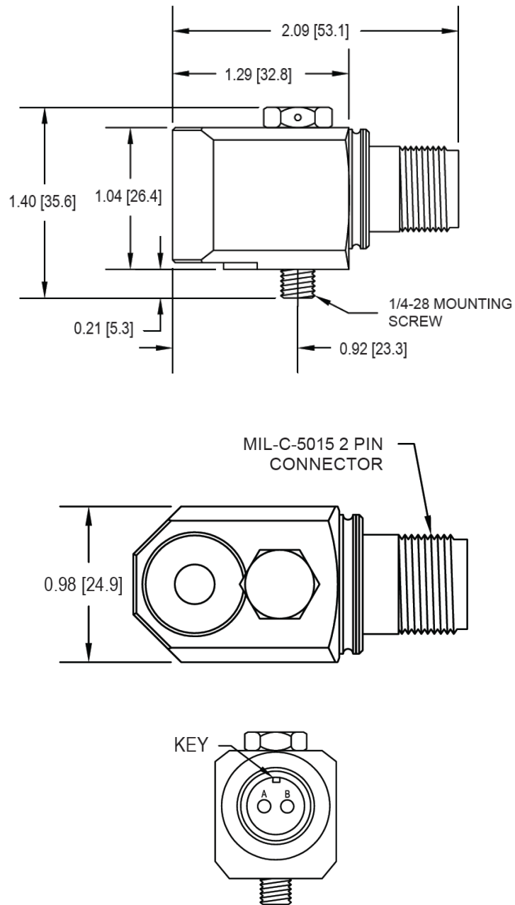
Figure 4: AP3500S2-Z1 dimensions
