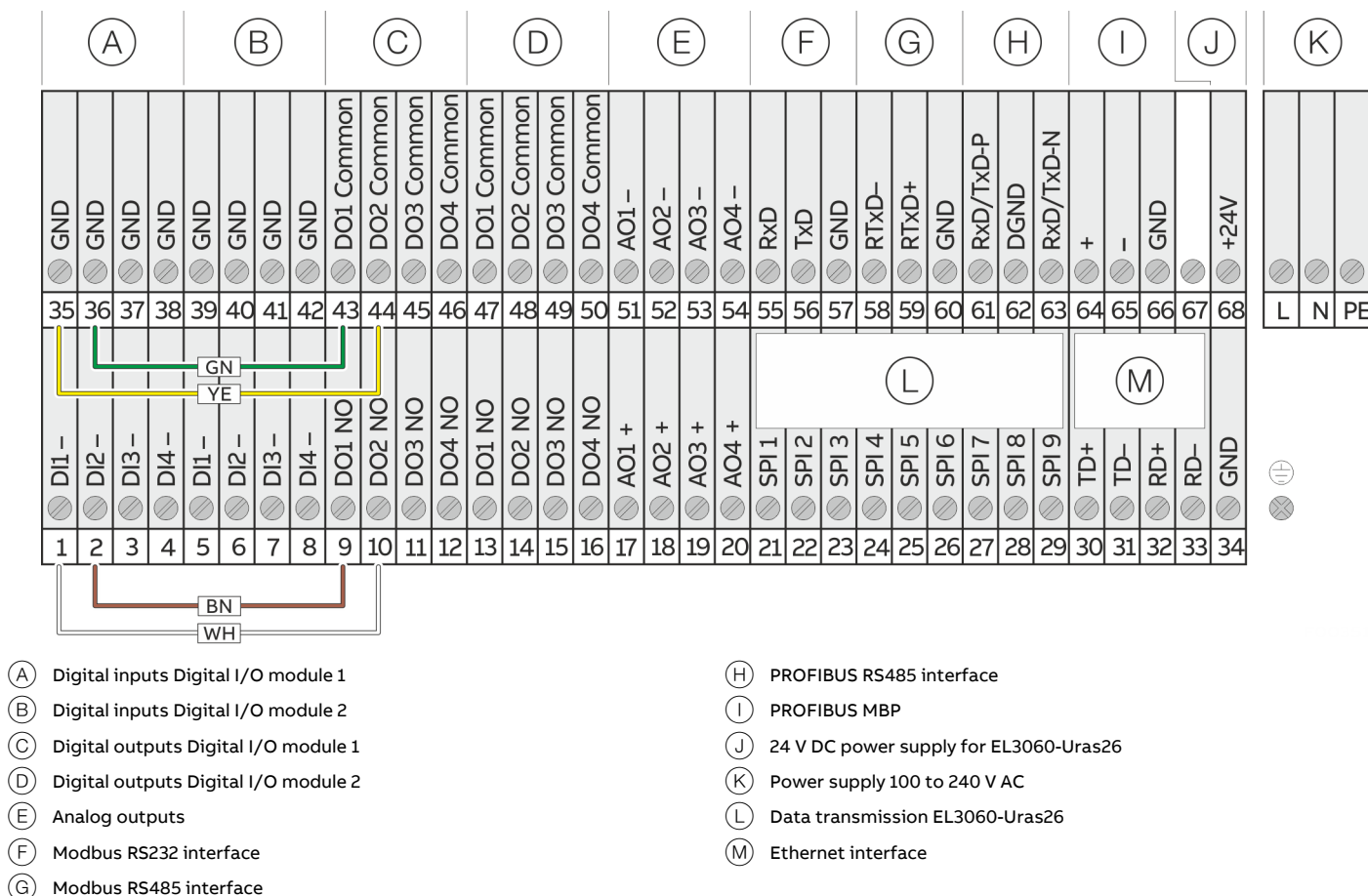
Figure 5: ‘Nitrogen Header’ application terminal assignment
