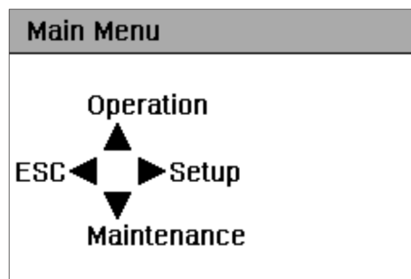
Figure 13: Main menu
