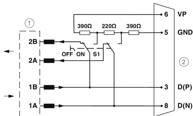
Figure 8: Connection to the D-SUB bus terminating connector
