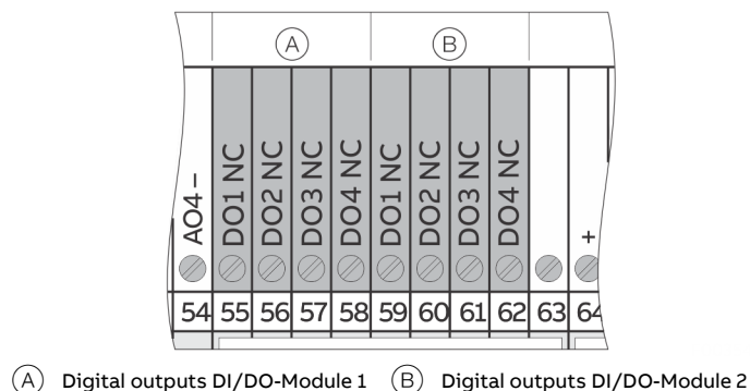
Figure 6: New assignment of terminals 55 to 63
