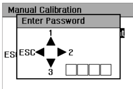
Figure 14: Password entry
