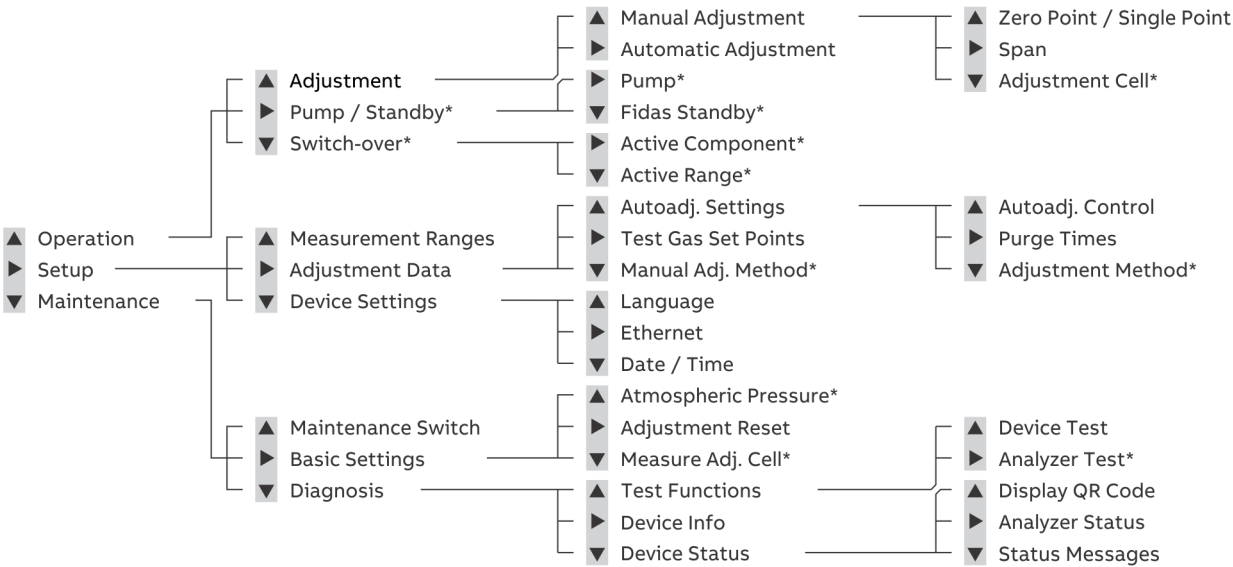
Figure 17: Menu overview
