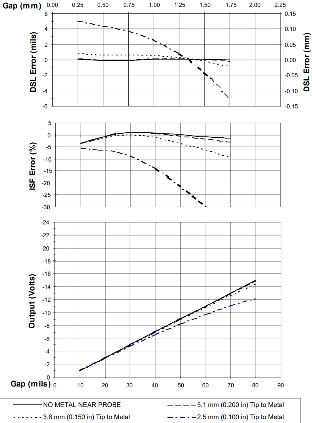
Figure II: Effect of Rear Surface Clearance (4140 Material)
