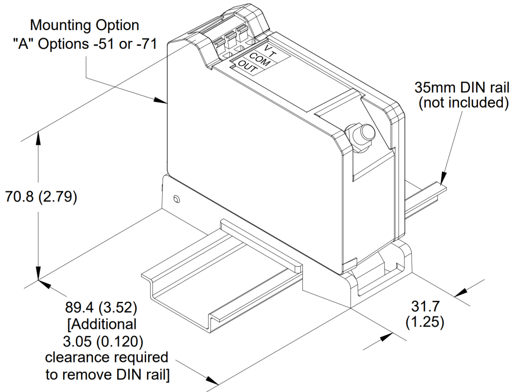
Figure 23: DIN Mount 3300 XL NSv Proximitior Sensor
