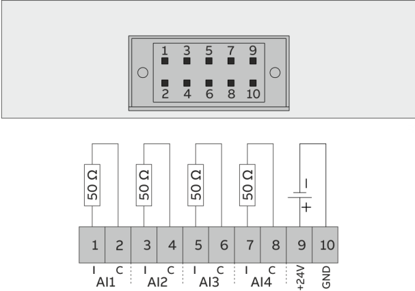
Figure 12: Analog input module
