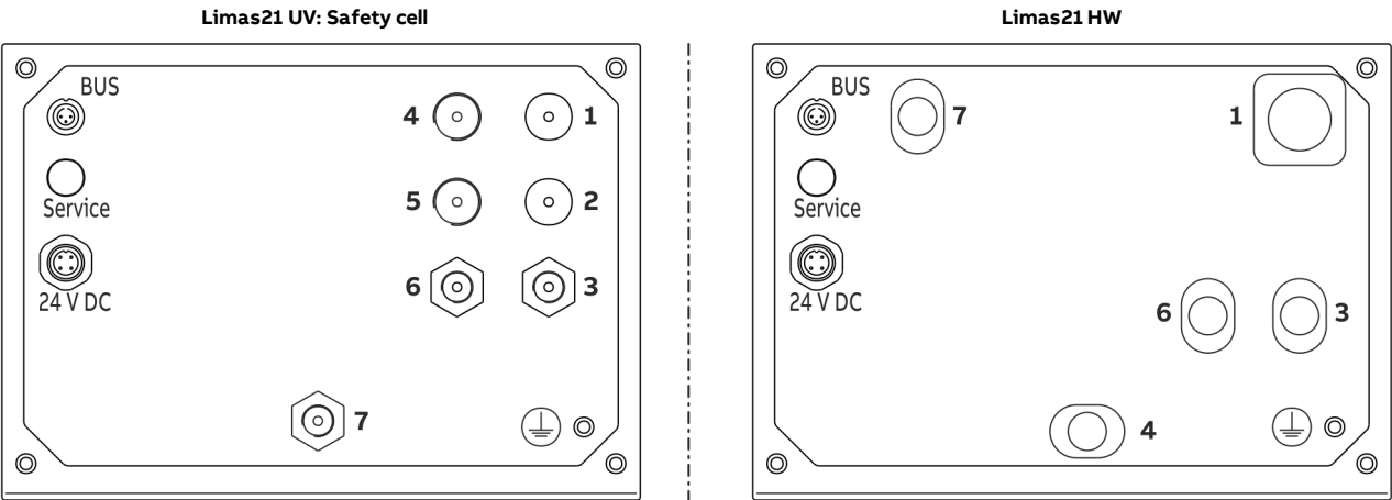
Figure 15: Limas21 UV and HW gas connections
