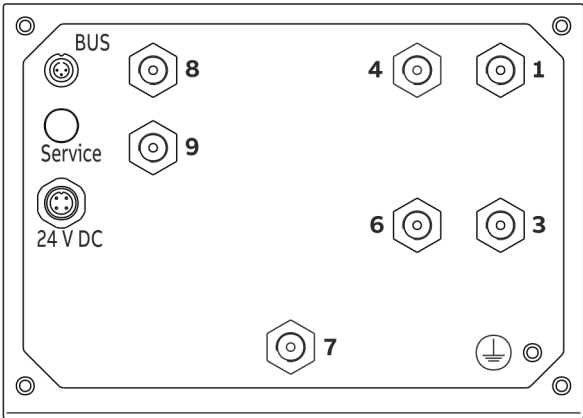
Figure 14: Limas21 UV gas connections
