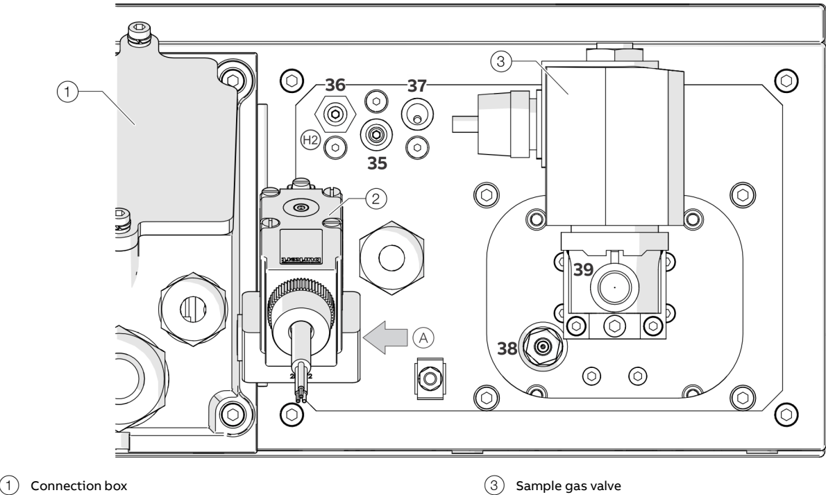
Figure 22: Position of the gas connections AO2040-Fidas24 Ex
