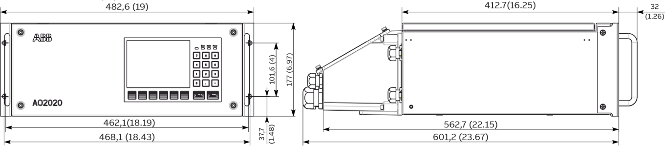
Figure 24: AO2020 dimensions
