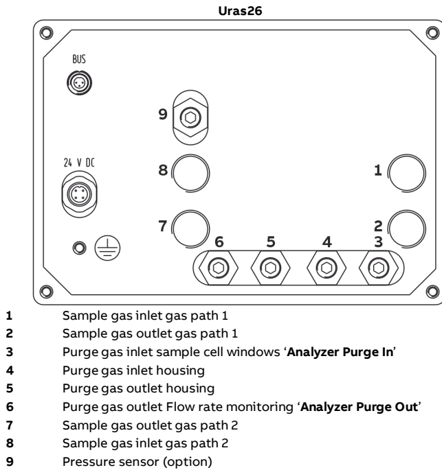
Figure 4: 'Safety Concept' gas connections Uras 26, Magnos28
