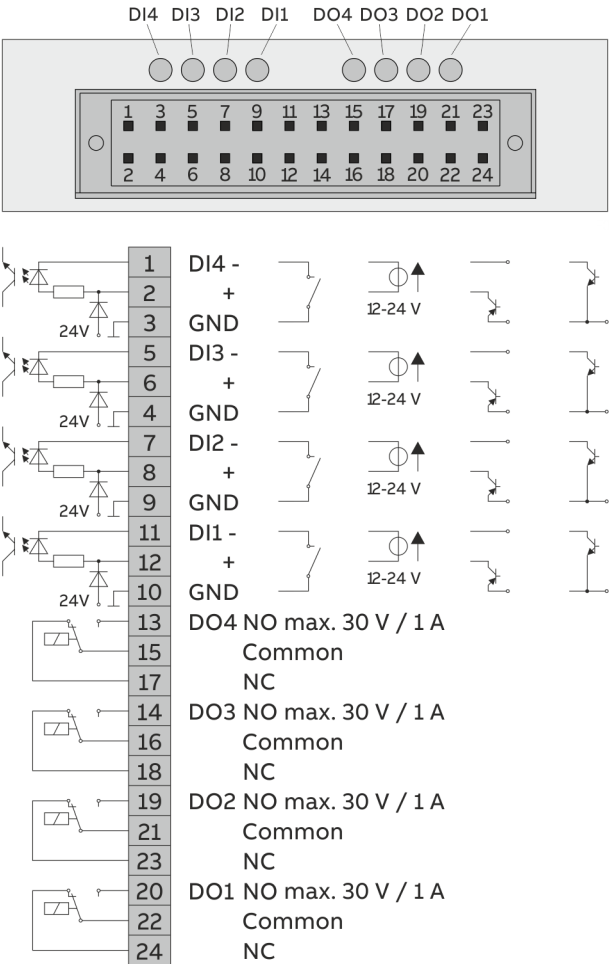
Figure 9: Electrical connections, digital I/O module
