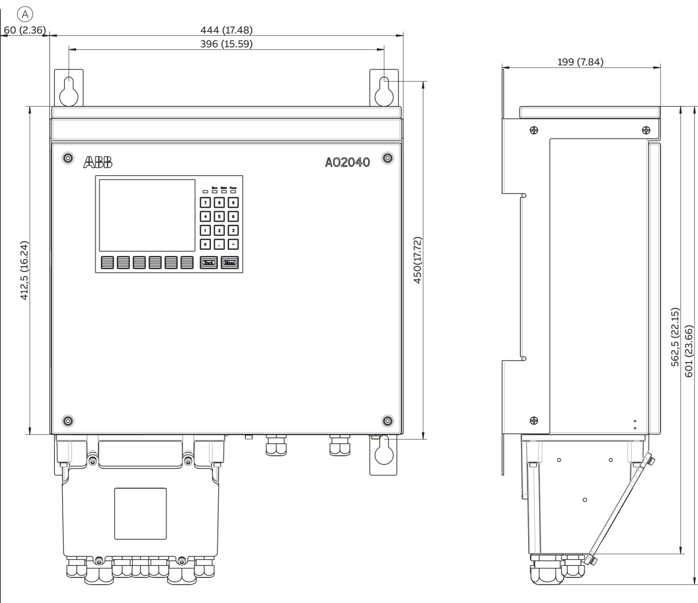
Figure 25: AO2040 dimensions
