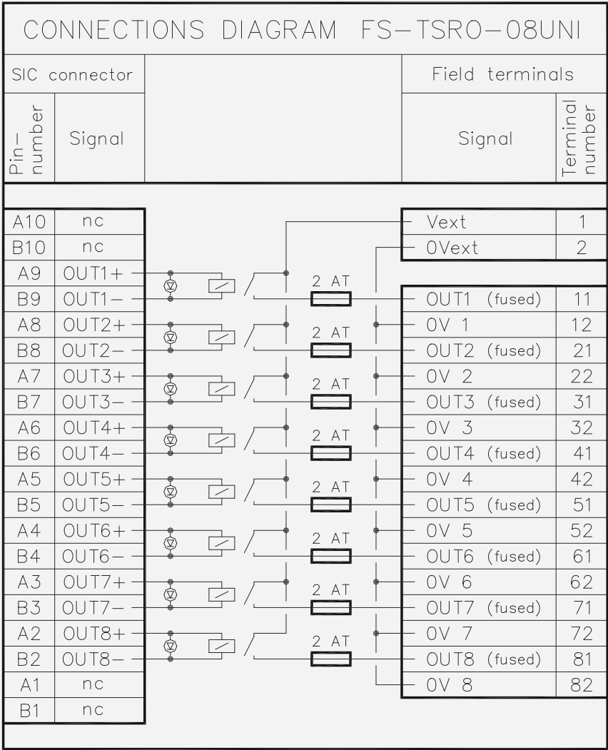
Figure 15-138: Connections diagram
