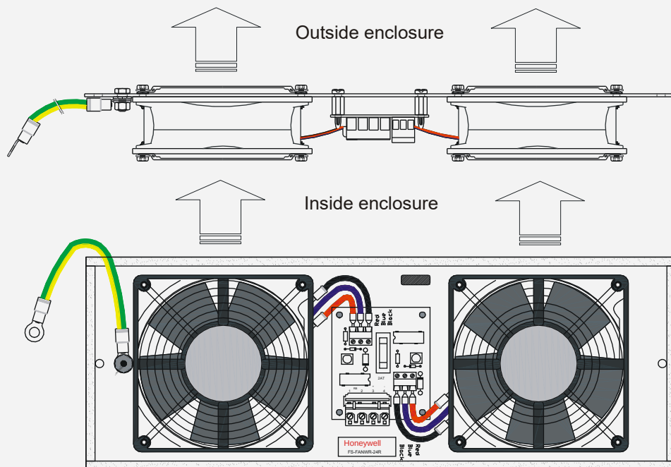
Figure 4-2: Layout of the FANWR-24R fan unit and direction of air flow
