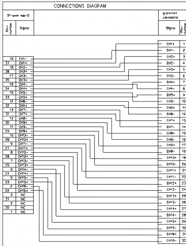
Figure 16-13: Connections diagram
