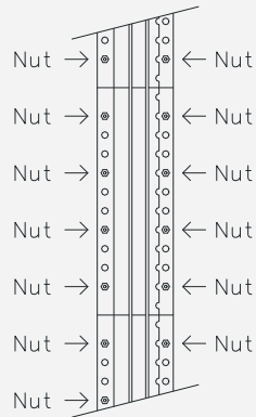
Figure 18-27: Section of the MB-0001 mains power rail
