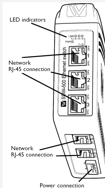
Figure 15-32: SDW-550 EC connections
