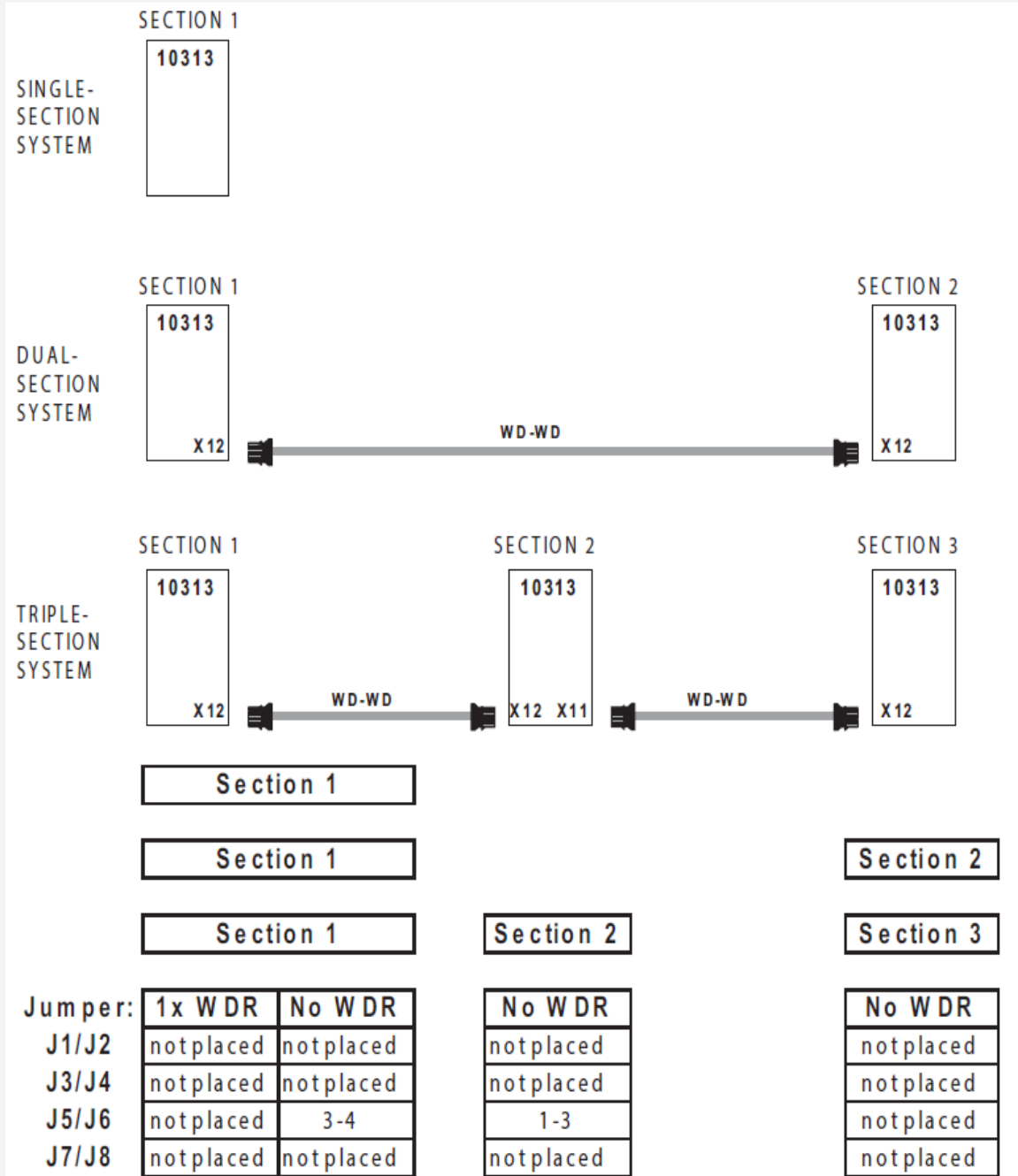
Figure 13-25: Distribution example
