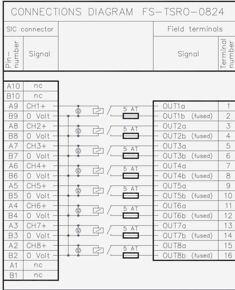
Figure 15-133: Connections diagram
