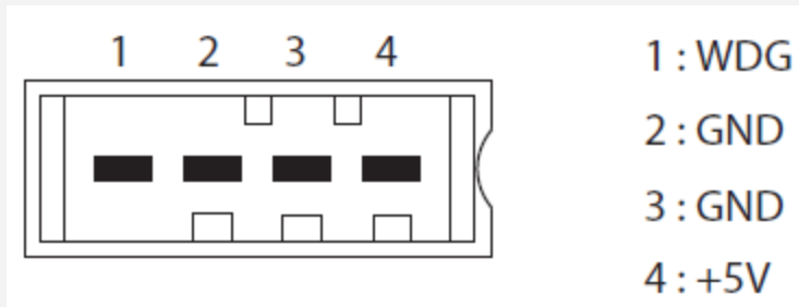
Figure 13-20: Pin connections of 'CP' and 'CP/CP-1' connector
