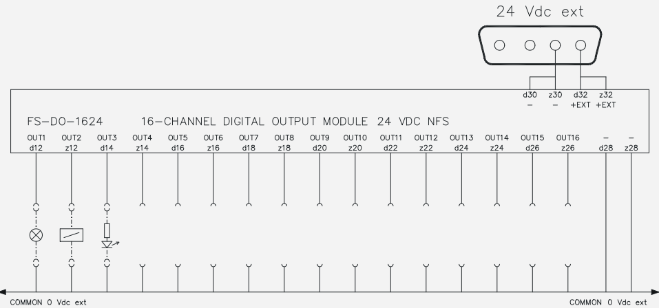
Figure 10-30: IO connection example for DO-1624 module for non-redundant IO configurations
