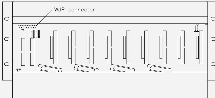
Figure 19-3: Position of the WdP connector on a redundant IO chassis
