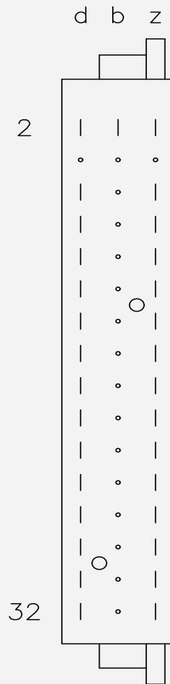
Figure 8-9: Back view and pin allocation of the SDI-1648 module connector
