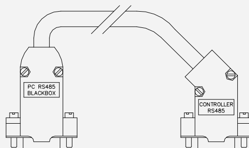
Figure 17-13: Pin assignment and layout of the CCE-485-02/Lx communication cable
