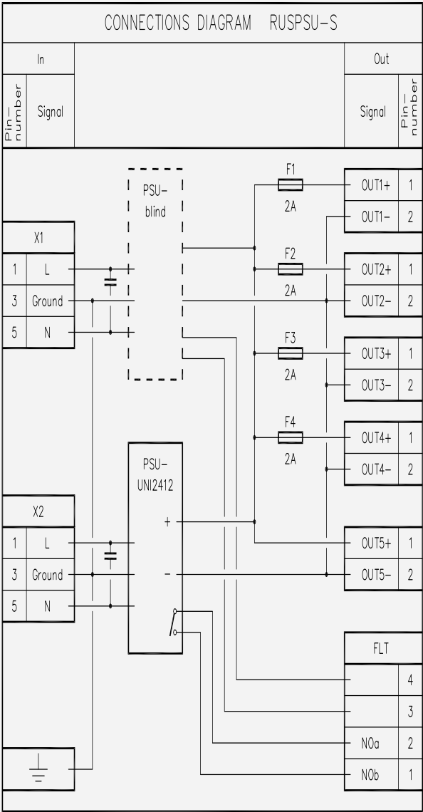
Figure 6-54: Connection diagram
