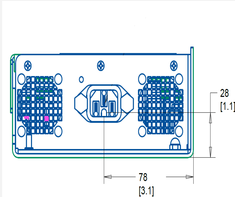
Figure 6-5: AC Input
