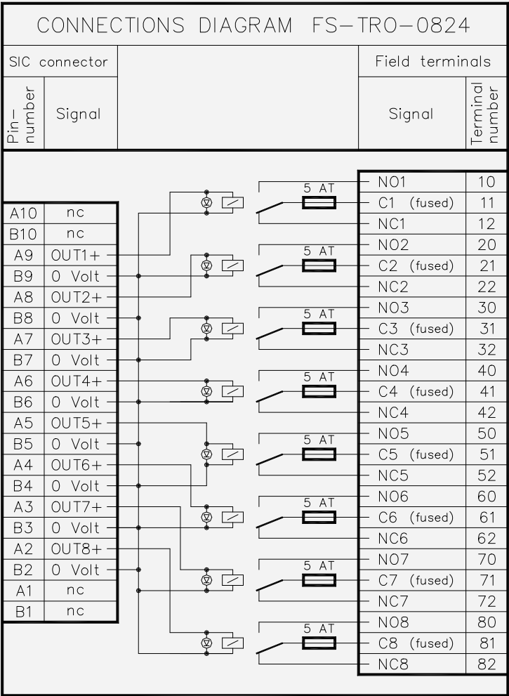
Figure 15-70: Connections diagram
