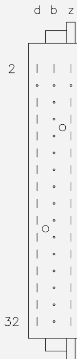
Figure 10-28: Back view and pin allocation of the DO-1624 module connector
