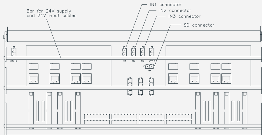
Figure 16-5: Safety Manager - Position of the SD, IN1, IN2 and IN3 connectors on the CP-backplane.
