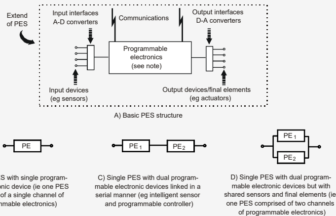
Figure 21-3: Programmable electronic system (PES): structure and terminology
