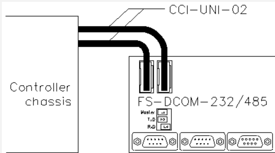
Figure 17-2: Redundant internal communication wiring to a DCOM-232/485 module
