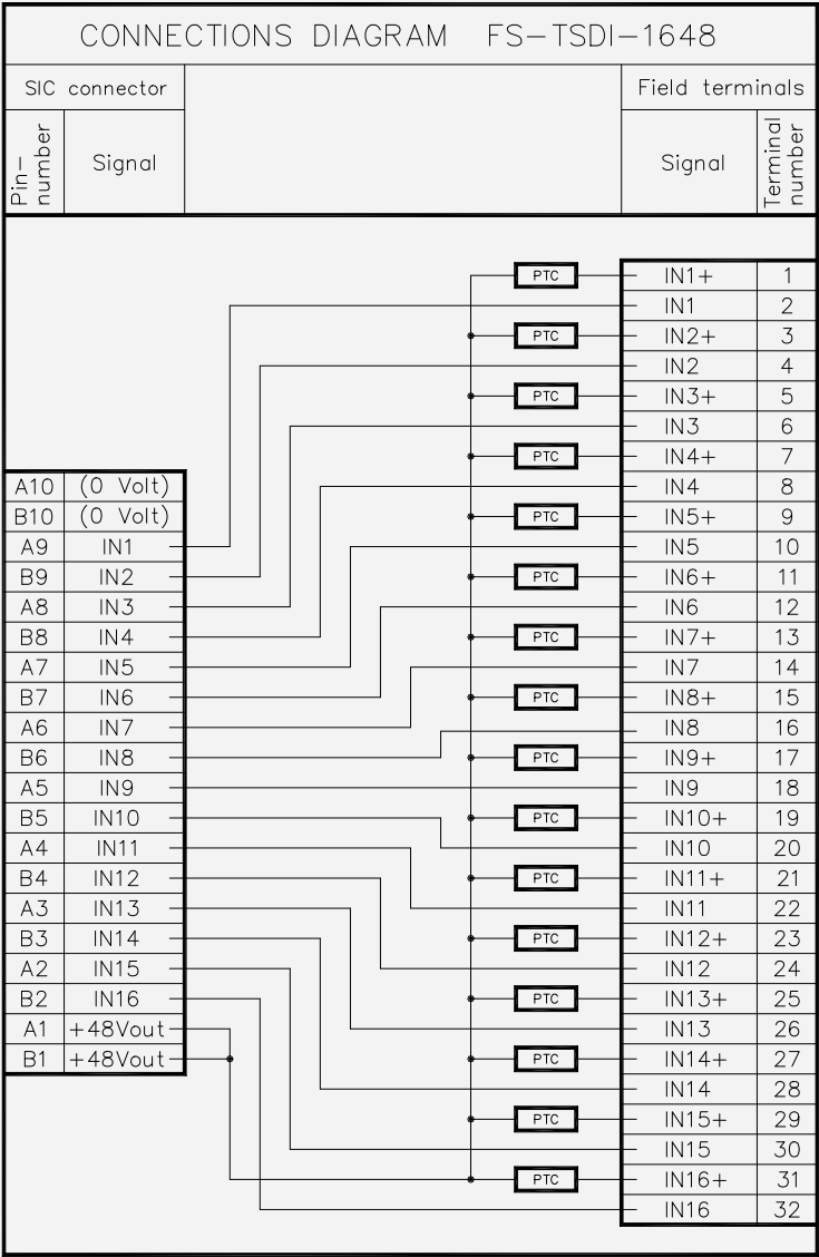
Figure 15-97: Connection diagram
