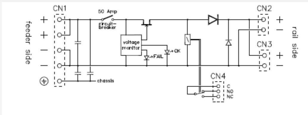
Figure 6-48: FDOVP-2450 Block Diagram
