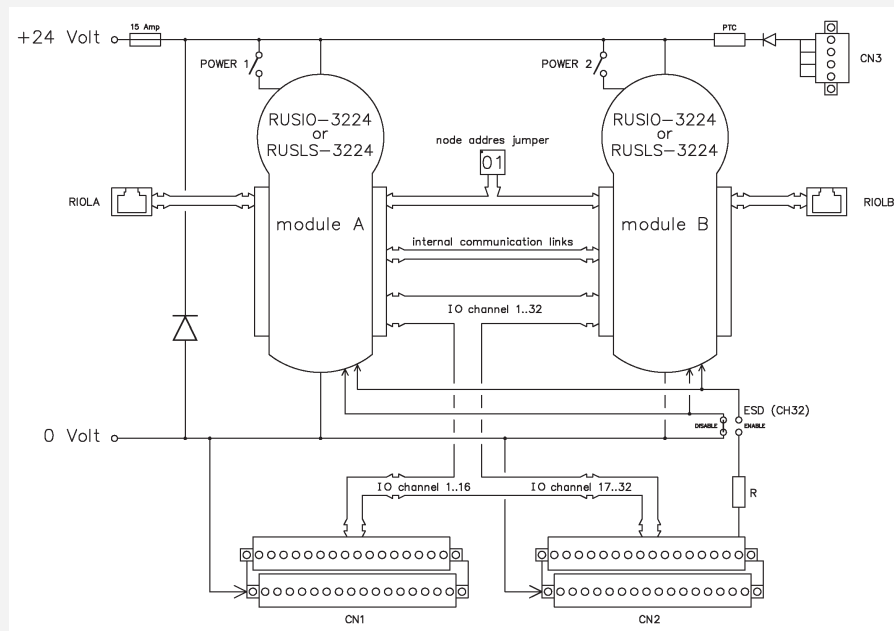
Figure 15-18: Block diagram
