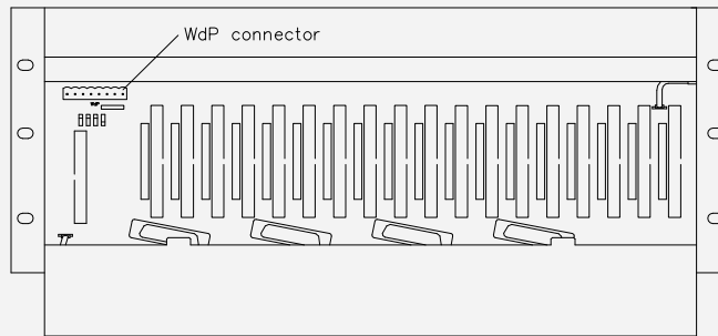
Figure 19-2: Position of the WdP connector on a non-redundant IO chassis
