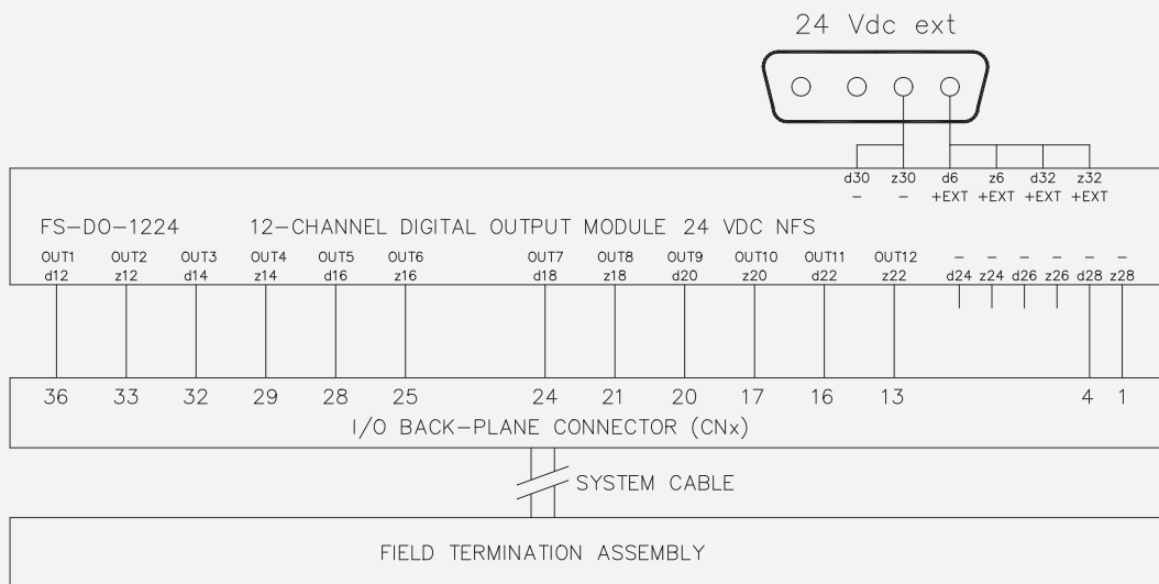
Figure 10-20: IO connection example for DO-1224 module for non-redundant IO configurations
