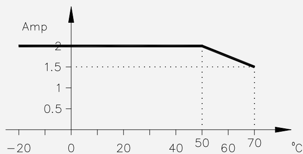
Figure 15-54: Derating curve (channel load vs ambient temperature) for the TDOL-0724P
