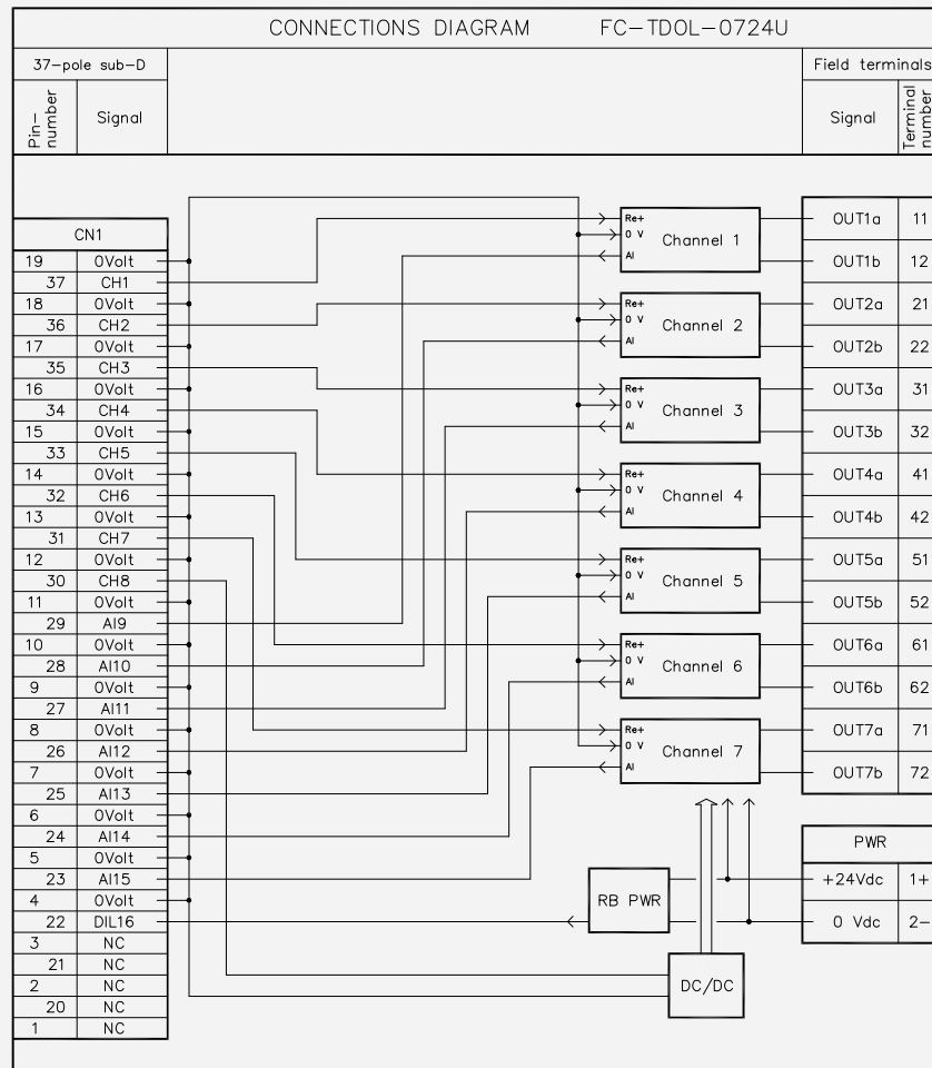
Figure 15-60: Connections diagram
