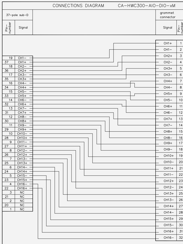
Figure 16-15: Connections diagram
