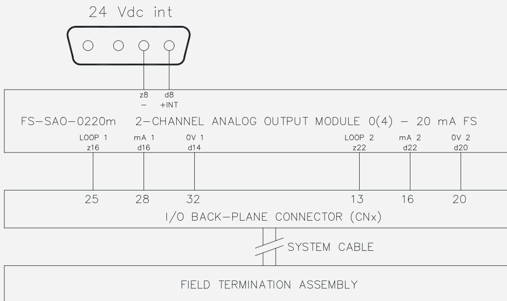
Figure 10-14: Connection example of SAO-0220m module to FTA for non-redundant IO configurations
