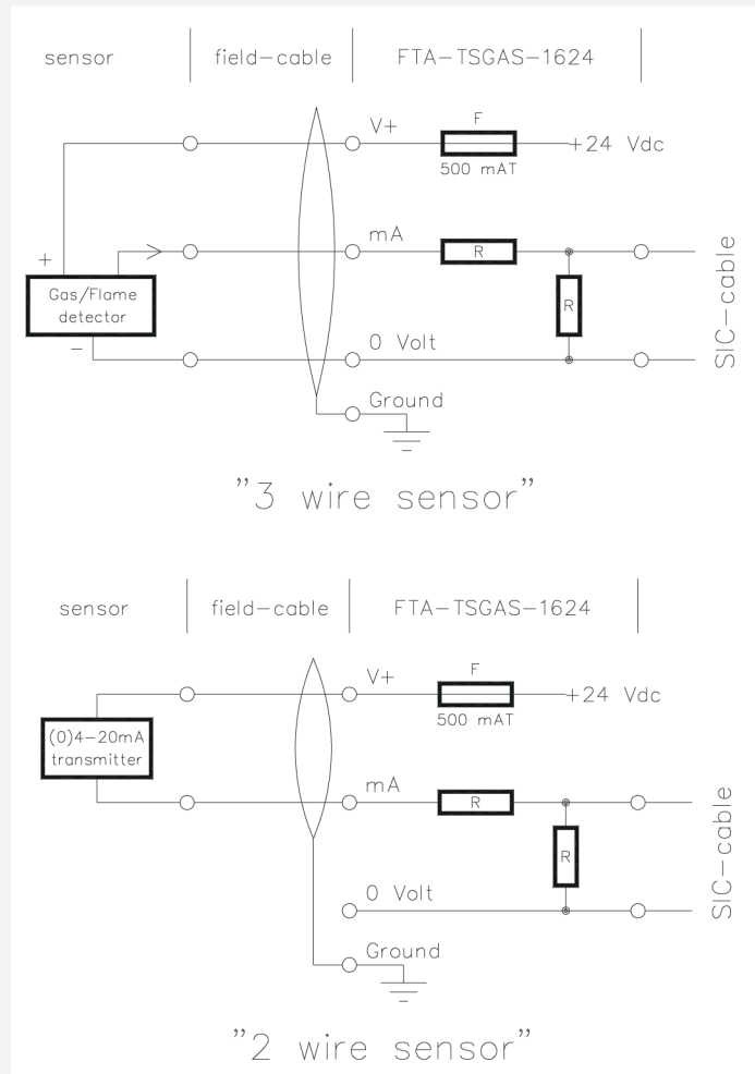
Figure 15-114: Schematic diagram for connecting a transmitter
