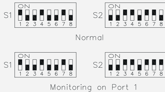
Figure 15-35: Advised DIP switch settings
