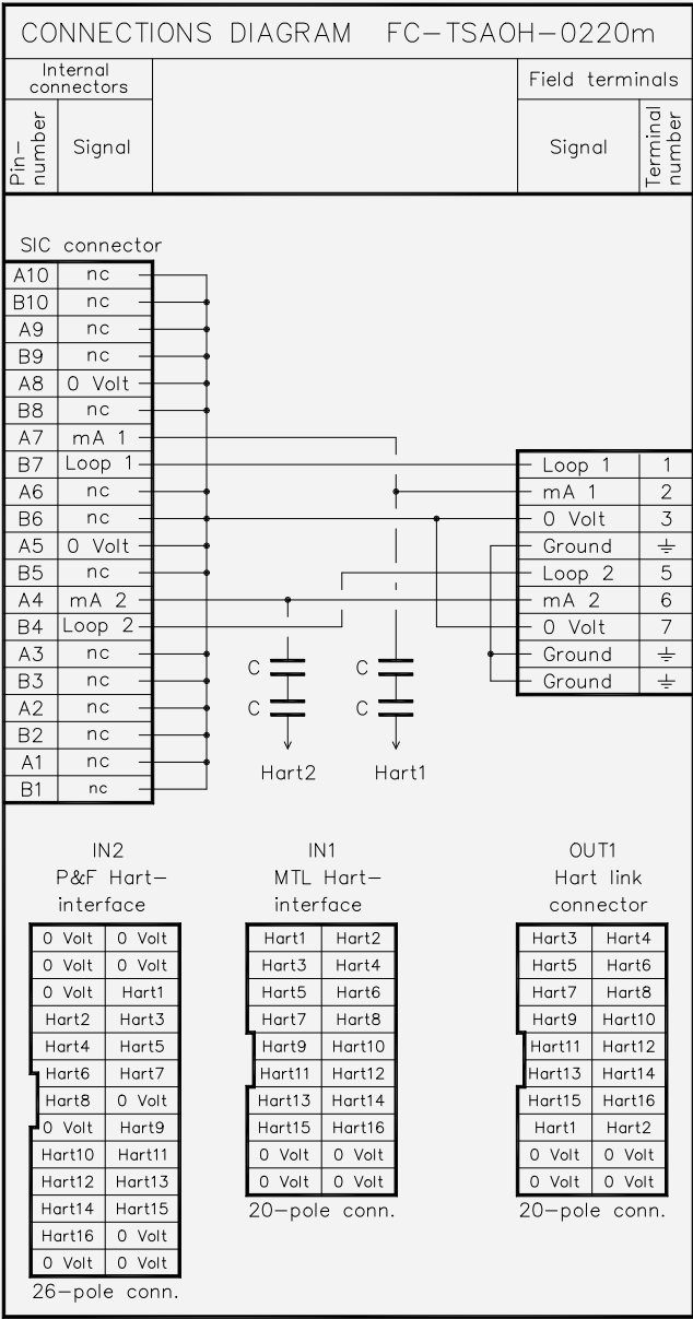
Figure 15-83: Connections diagram
