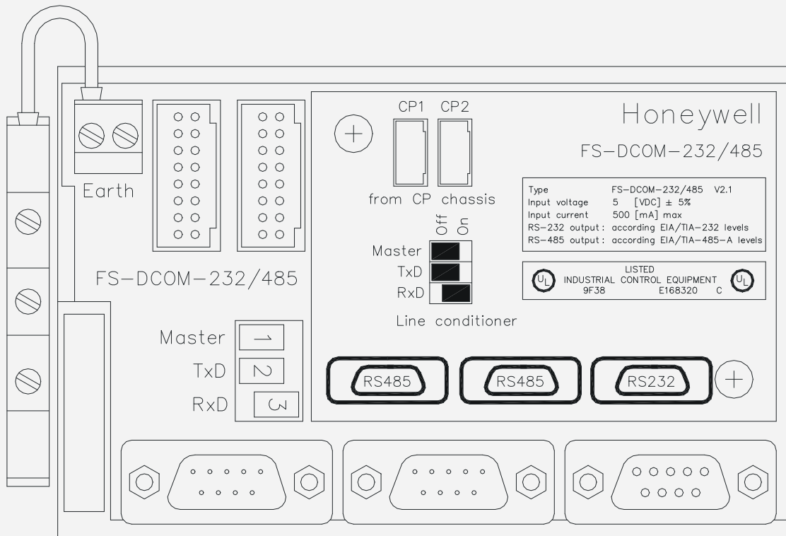
Figure 15-1: Top view of the DCOM-232/485 communication FTA
