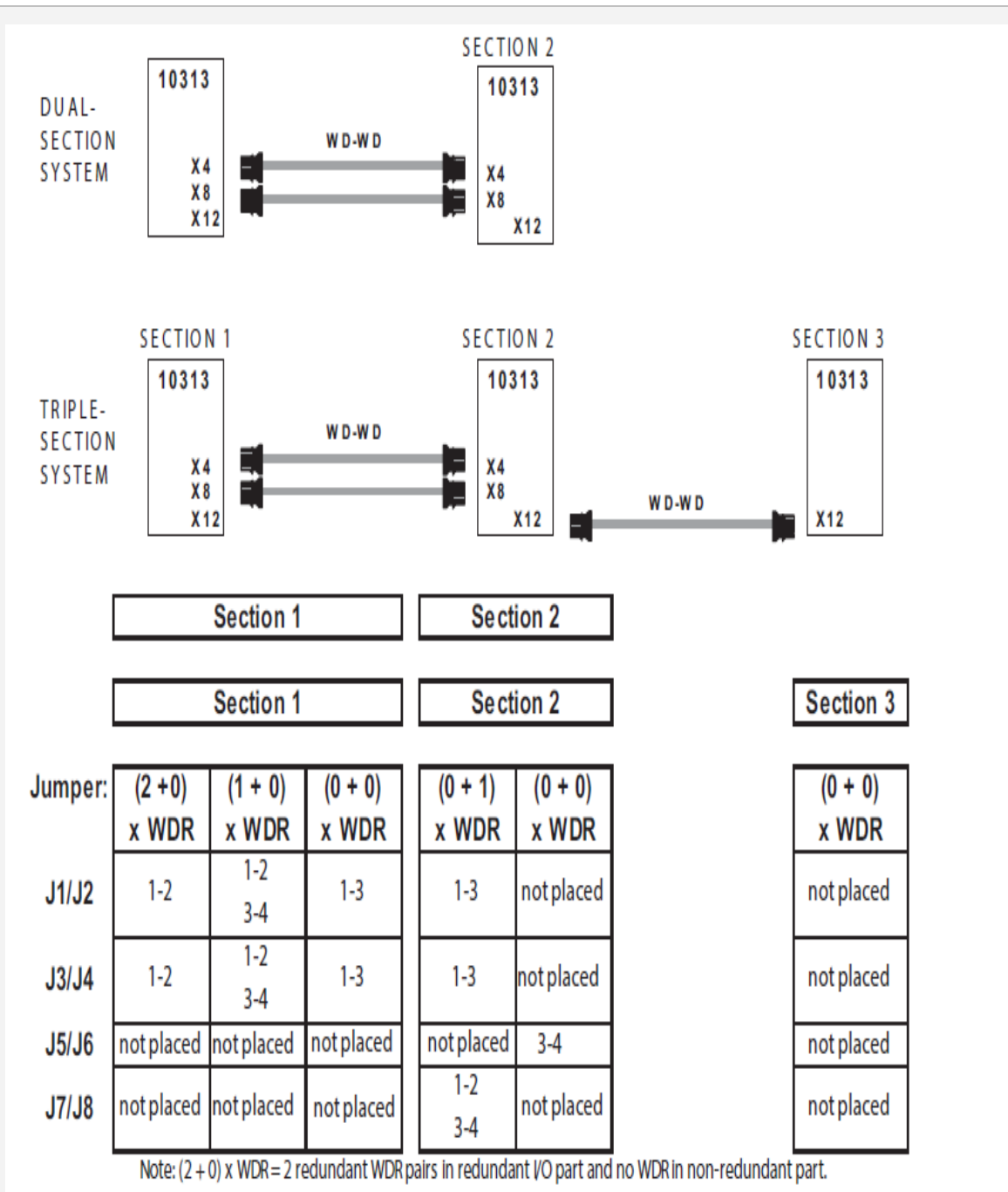
Figure 13-28: Distribution example
