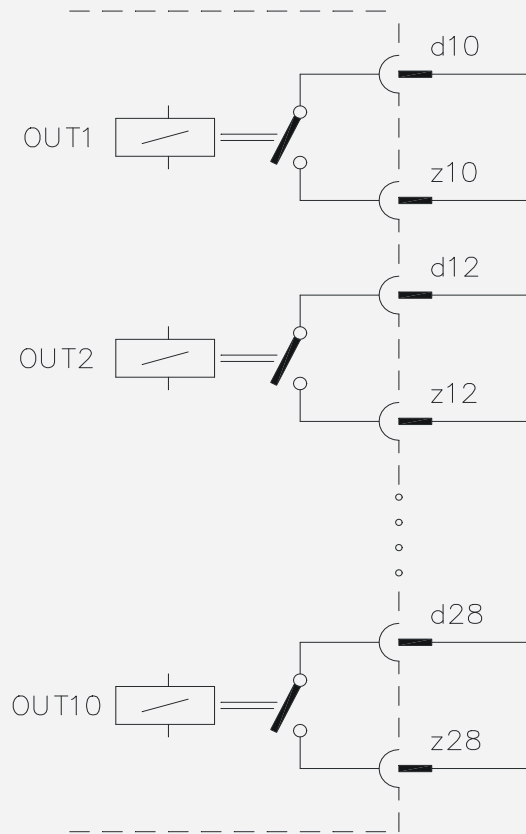
Figure 10-22: Schematic diagram for RO-1024 module
