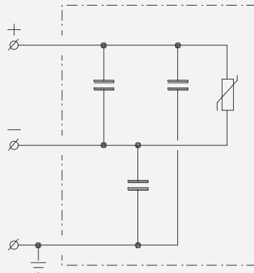
Figure 18-6: SIF-X circuit
