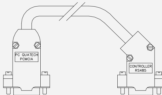
Figure 17-15: Pin assignment and layout of the CCE-485-05/Lx communication cable
