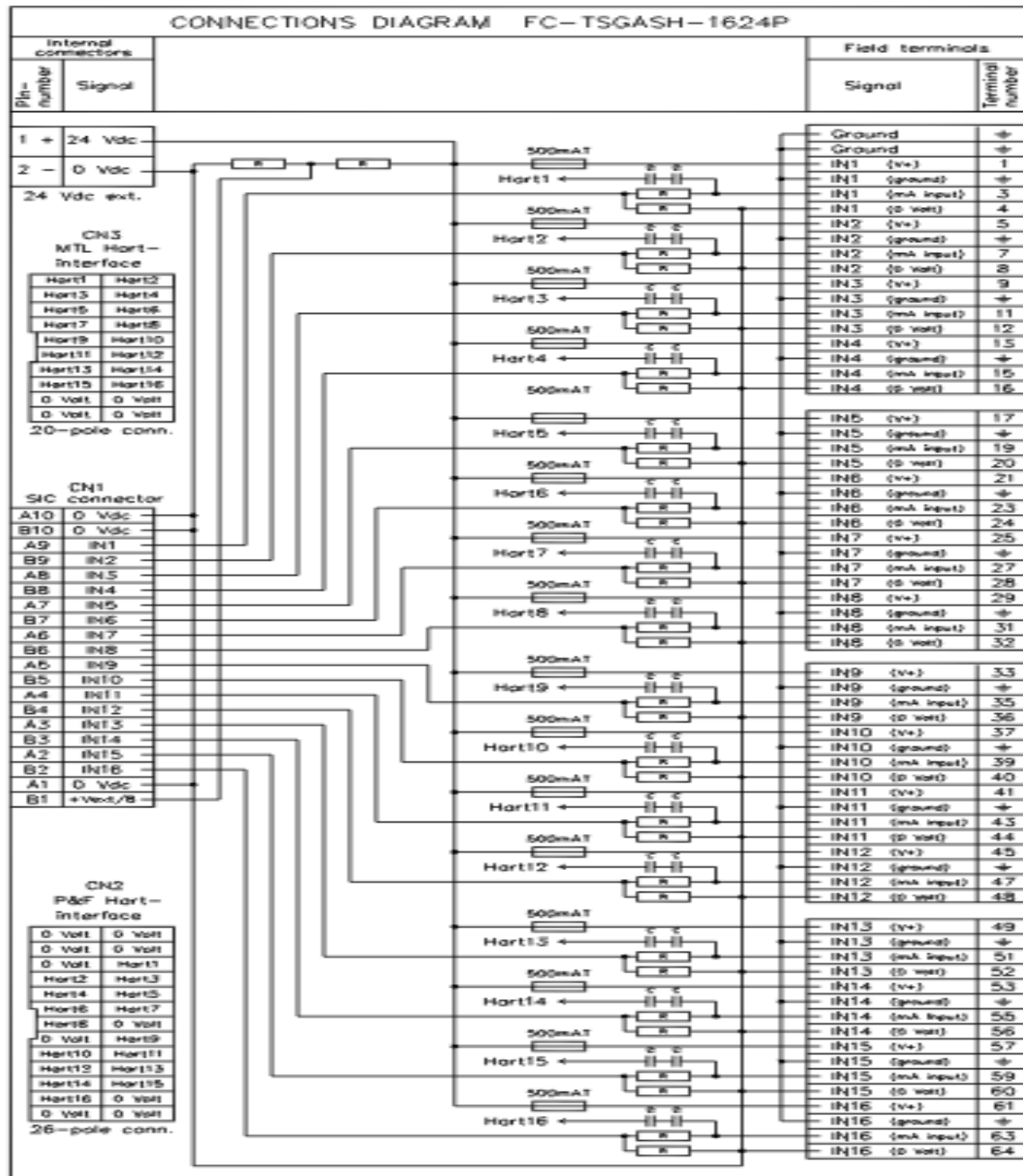
Figure 15-116: Connections diagram
