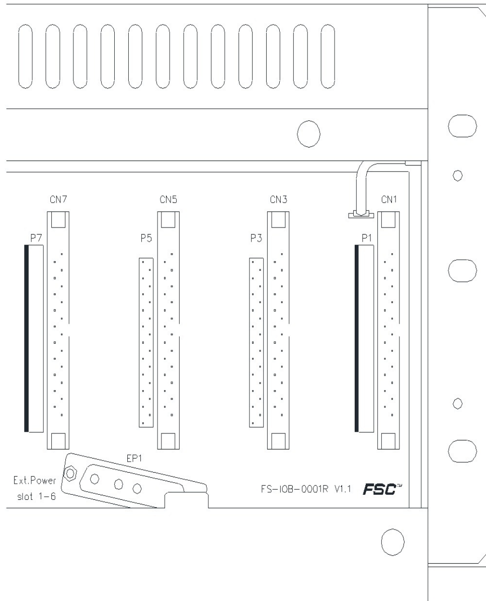
Figure 11-1: Detail of the back of a non-redundant IO chassis
