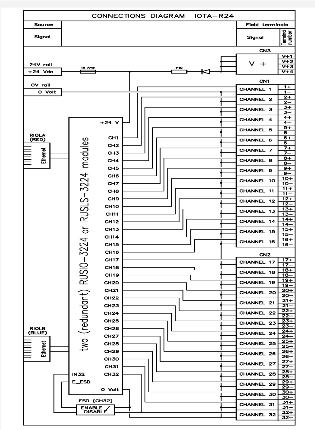
Figure 15-25: Connection diagram
