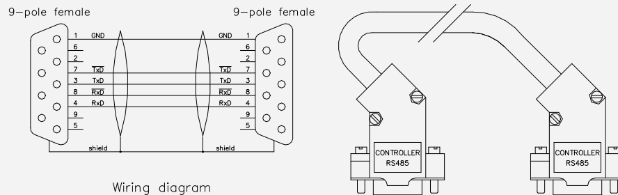
Figure 17-12: Pin assignment and layout of the CCE-485-01/Lx communication cable
