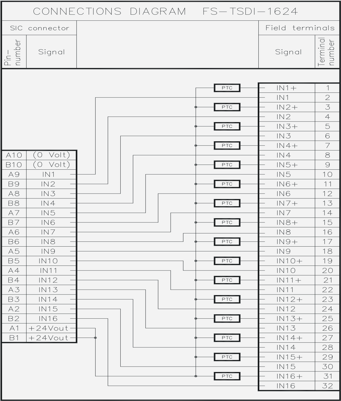
Figure 15-93: Connection diagram
