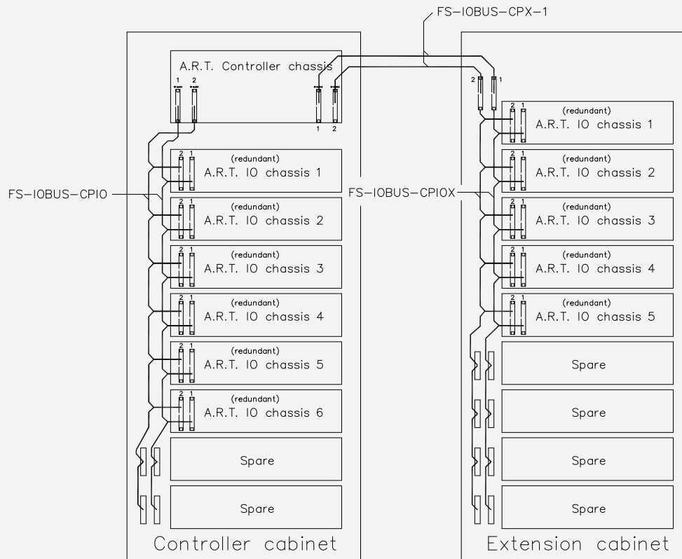
Figure 14-5: IO busses example for a IO chassis in the extension cabinet
