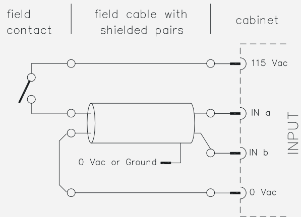
Figure 15-88: Field cable with shielded pairs
