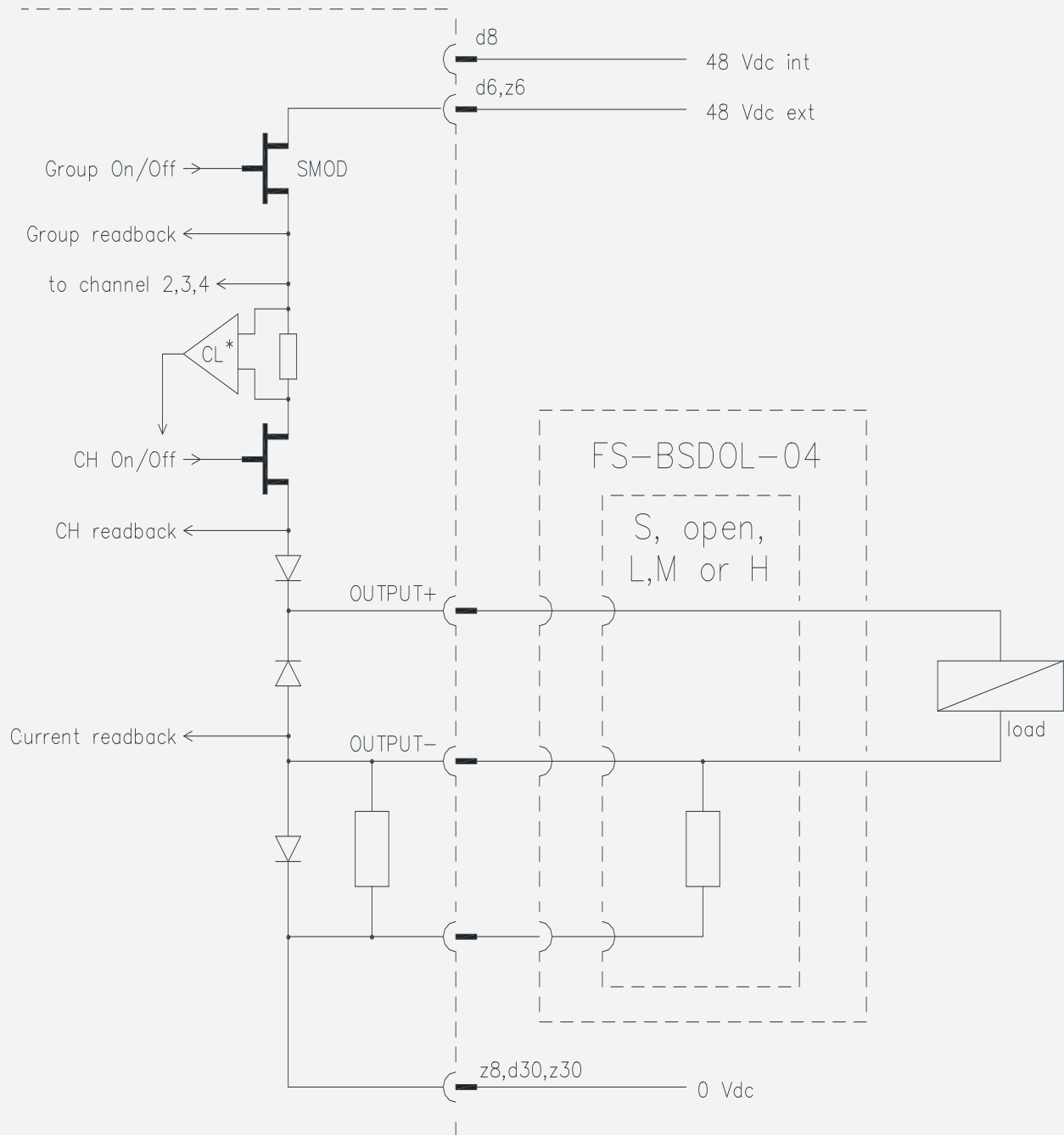
Figure 10-50: Schematic diagram for connection of one output to the SDOL-0448 module
