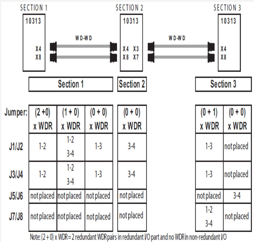
Figure 13-29: Distribution example
