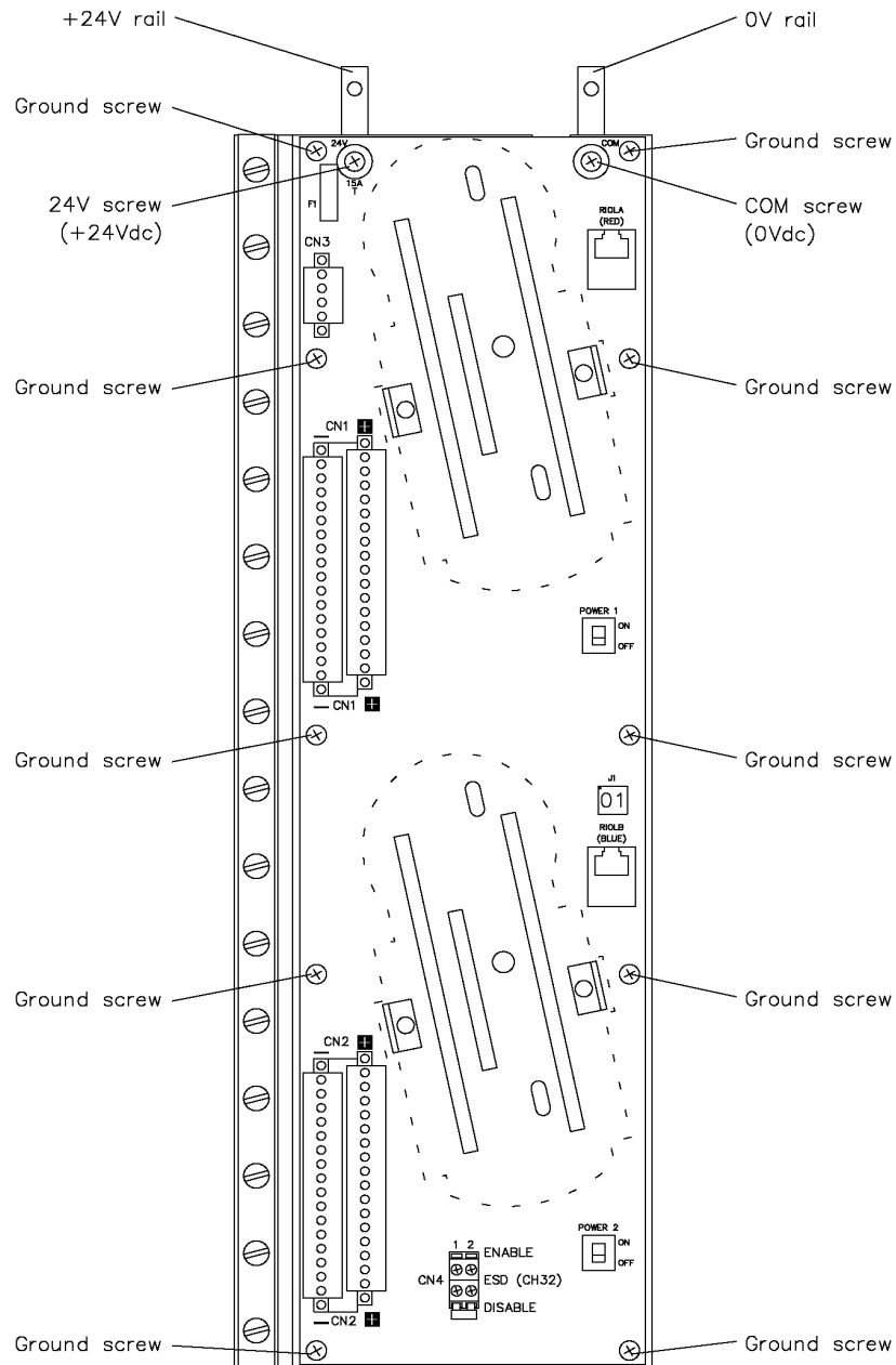
Figure 4-8: MCAR-01 with a mounted IOTA-R24
