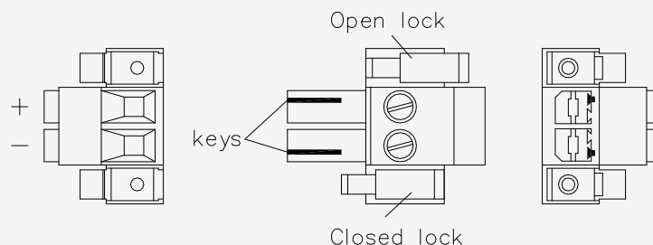
Figure 15-53: Power input connector (Weidmuller BVZ 7.62HP/02/180F SN) top, side and bottom view
