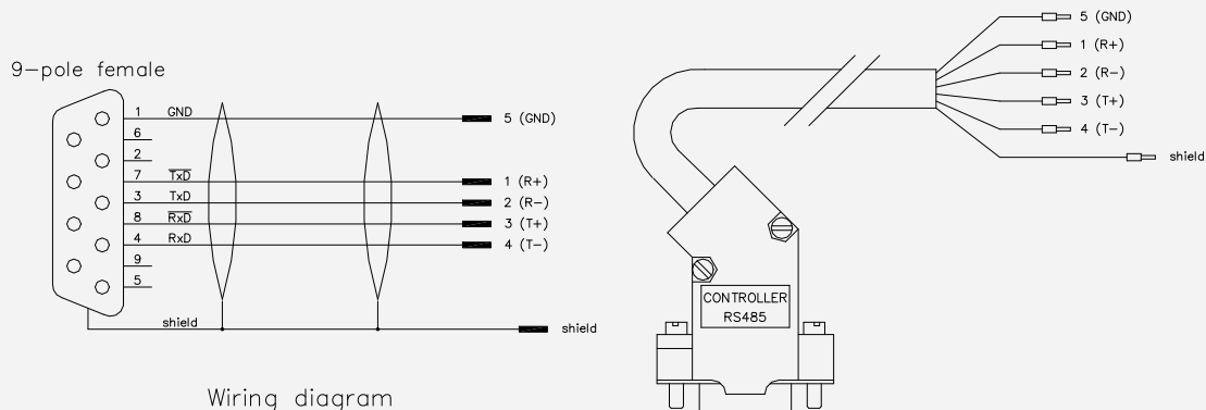
Figure 17-17: Pin assignment and layout of the CCE-485-FO-02/Lx communication cable
