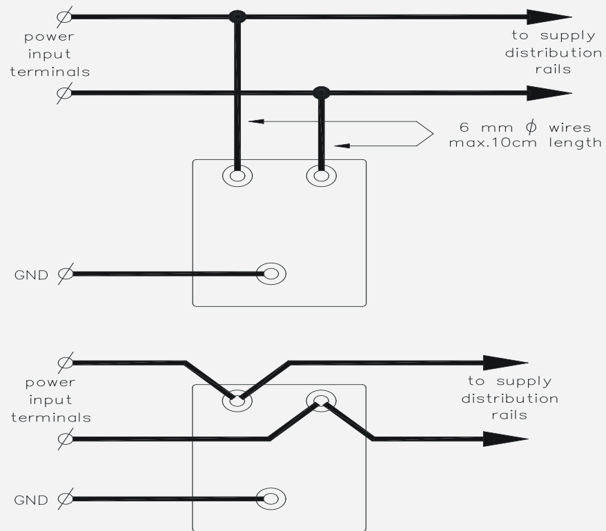
Figure 18-7: Wiring examples for SIF-X modules
