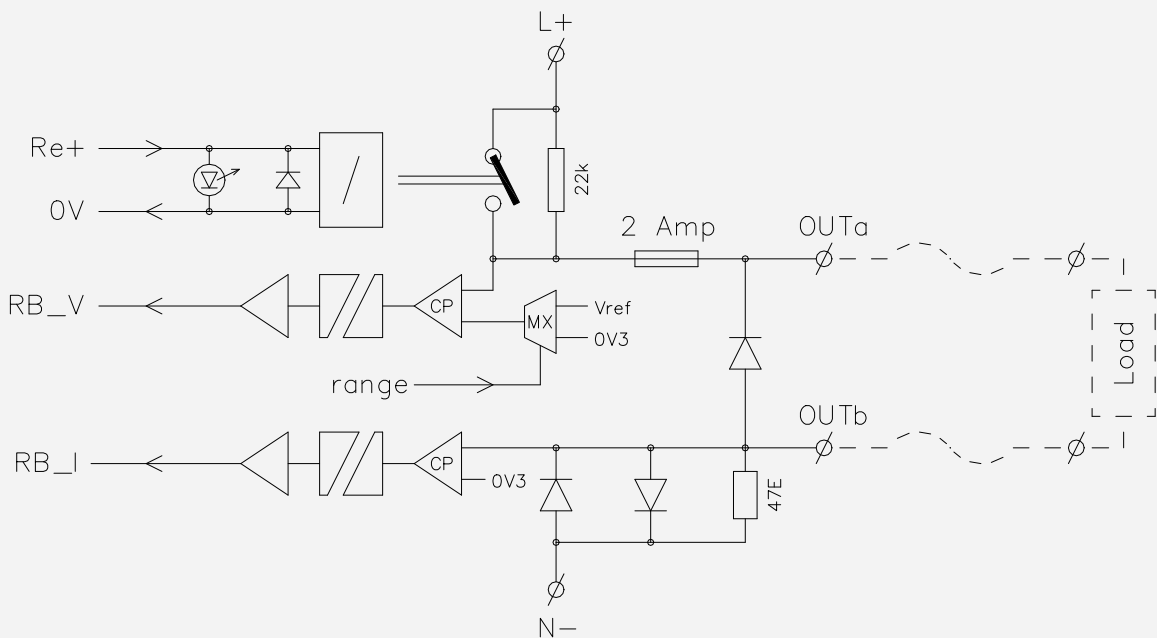
Figure 15-47: Schematic diagram of a channel
