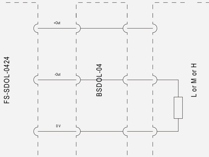
Figure 11-5: Schematic diagram for a channel with range setting sub-module
