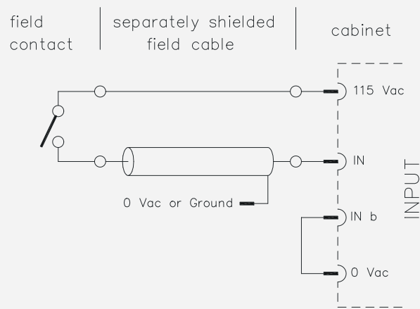
Figure 15-87: Field cable with separately shielded wires
