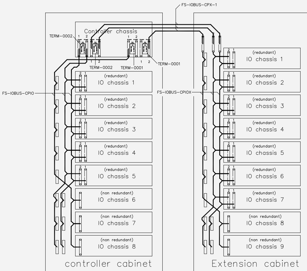
Figure 14-2: IO busses example for a two cabinet system
