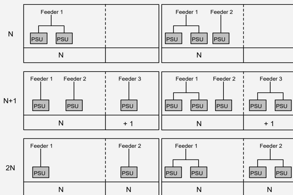
Figure 6-1: Power Supply Units configurations (2 examples for each configuration)
