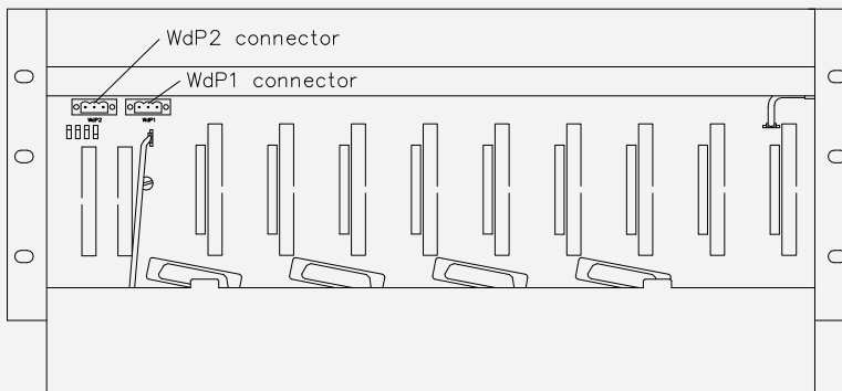
Figure 19-9: Position of the WdP connector on a redundant IO chassis
