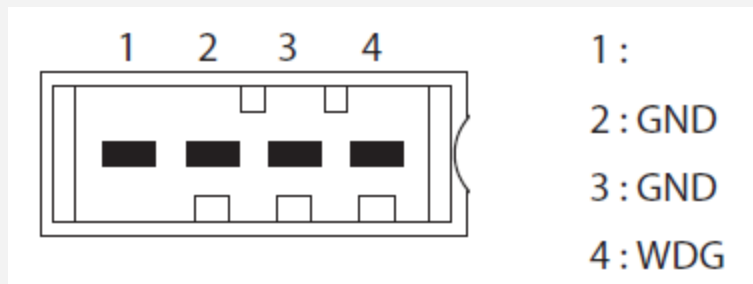
Figure 13-22: Pin connections of 'OUT/IN' connectors
