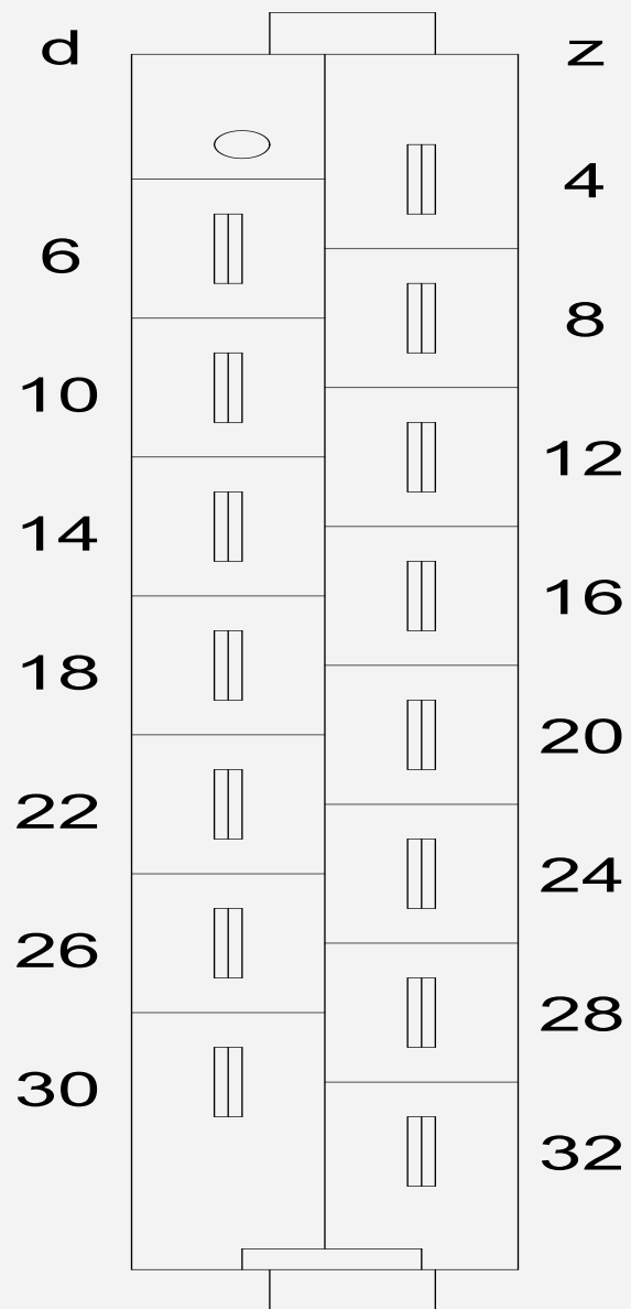
Figure 7-13: Back view and pin allocation of the PSU-240516 module
