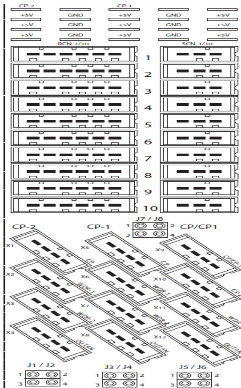
Figure 13-16: Top View
