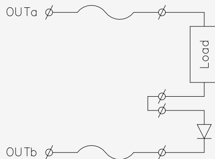
Figure 15-48: Additional diode for loads < 400 \Omega
