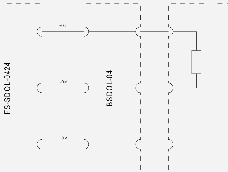
Figure 11-6: Schematic diagram for a spare channel
