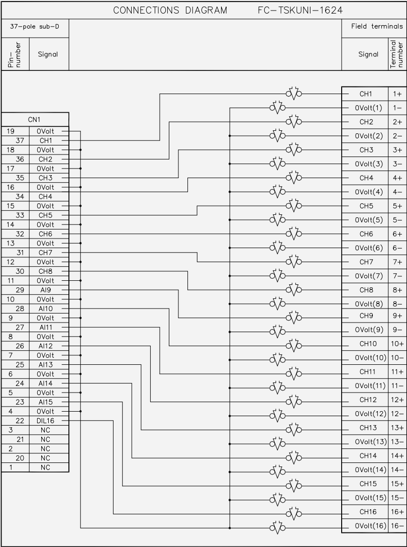
Figure 15-123: Connection diagram
