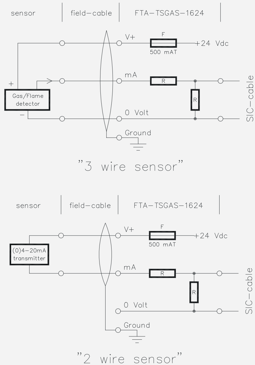
Figure 15-111: Schematic diagram for connecting a transmitter
