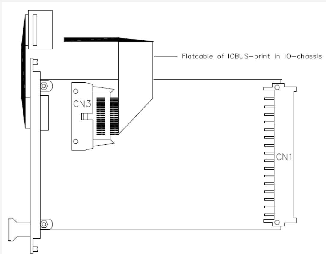
Figure 14-6: Side view of the IO-0001 module with a flatcable from a non-redundant IO chassis
