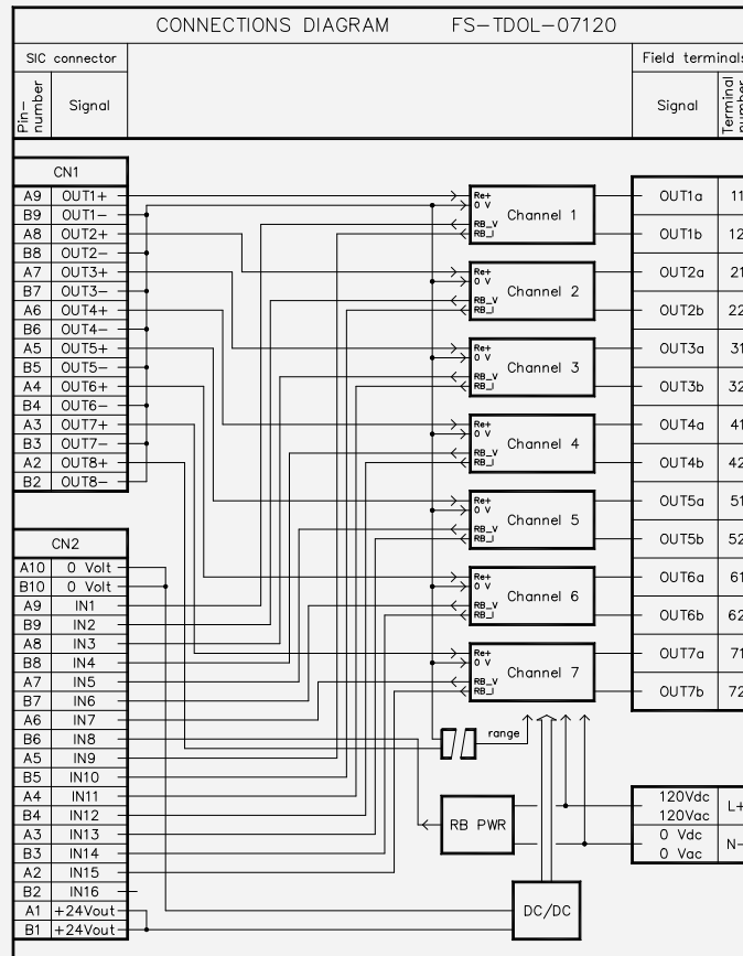
Figure 15-44: Connections diagram
