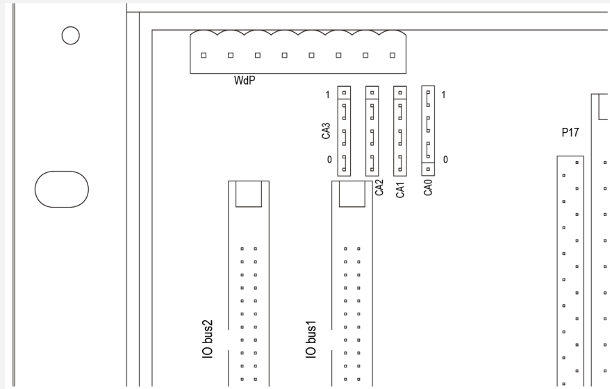
Figure 14-10: Jumpers on the CPB-0001R
