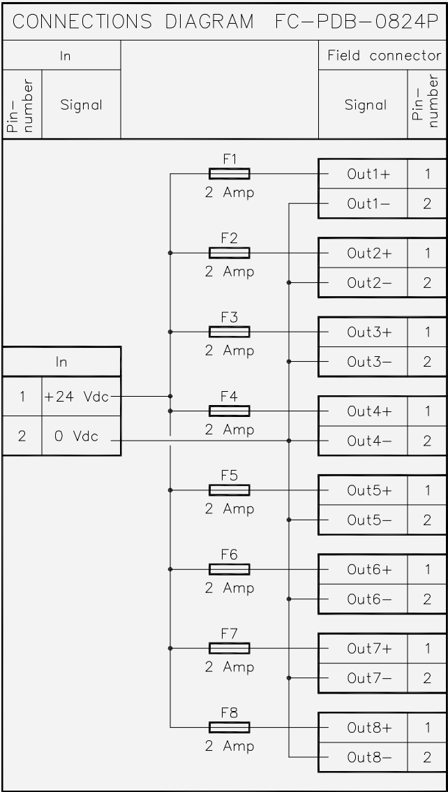
Figure 18-25: Connection diagram
