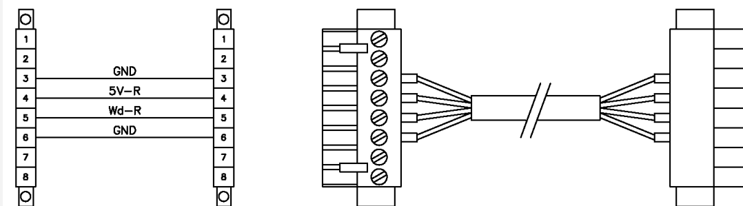
Wiring diagram
