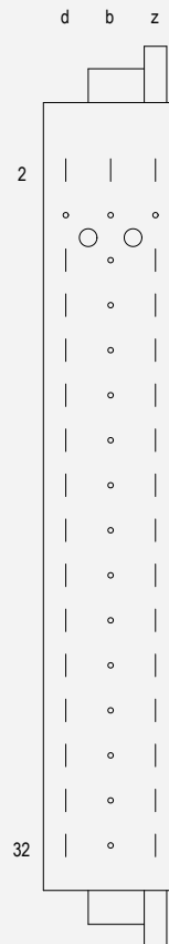
Figure 8-3: Back view and pin allocation of the SDI-1624 module connector
