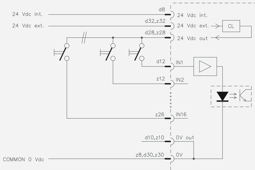
Figure 8-2: Schematic diagram for connection of inputs to the SDI-1624 module
