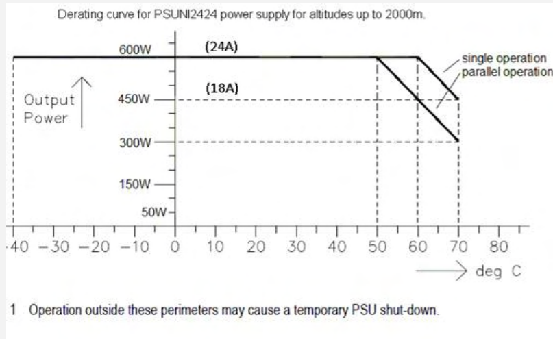
Figure 6-8: Output derating curve
