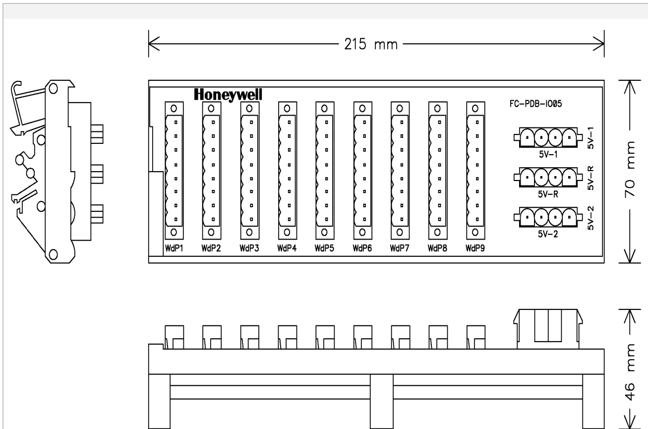
Figure 19-19: PDB-IO05 board layout
