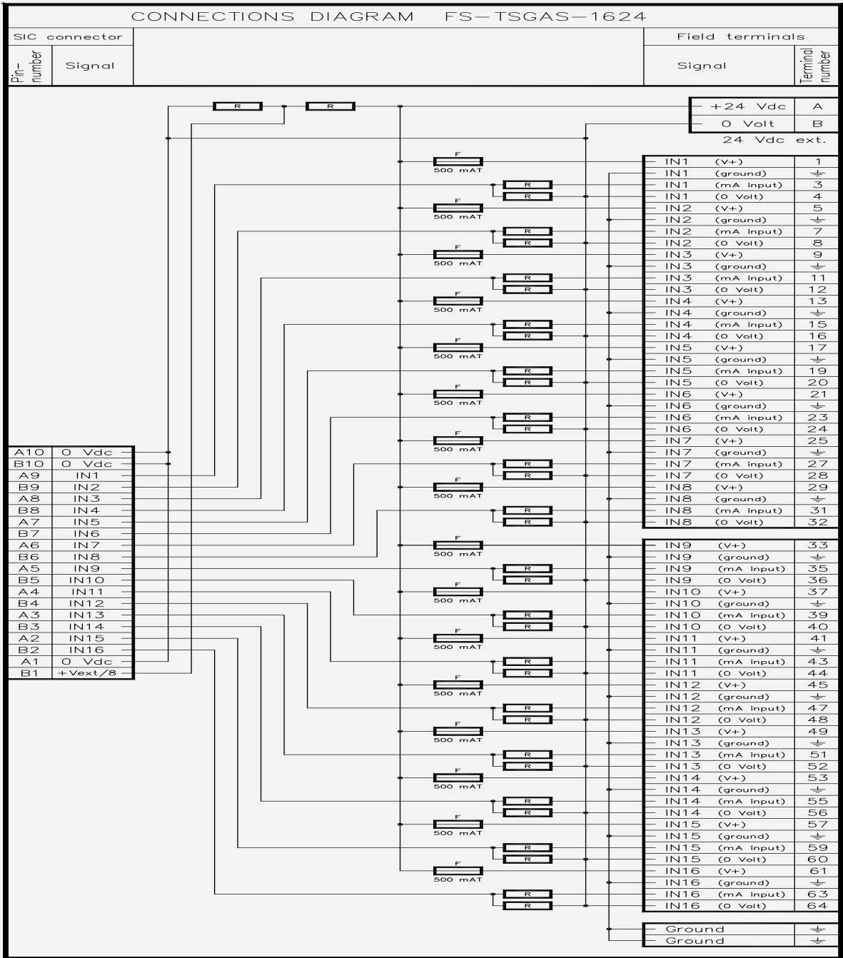
Figure 15-112: Connections diagram
