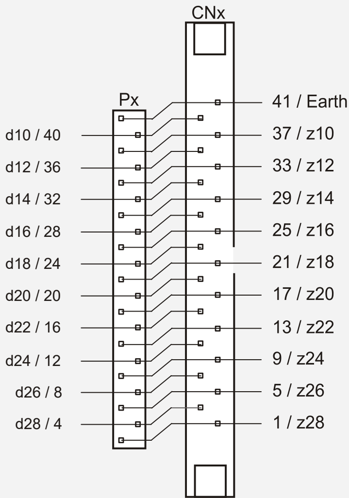
Figure 5-34: Pin mapping from IO connector to SIC cable (CNx) and converter (Px) connector
