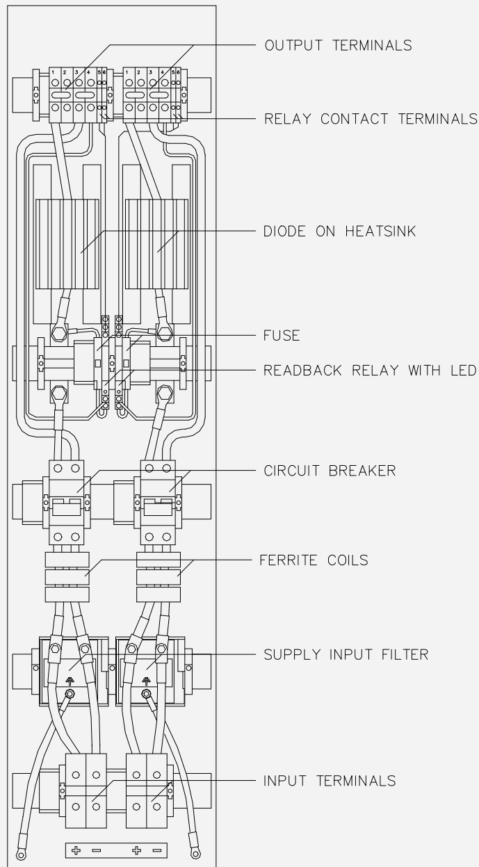
Figure 6-42: Layout of the 48 V DC Feeder unit redundant
