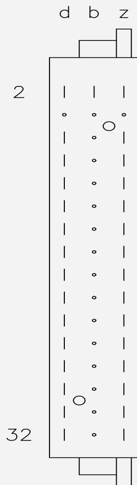
Figure 8-26: Back view and pin allocation of the SDIL-1608 module connector
