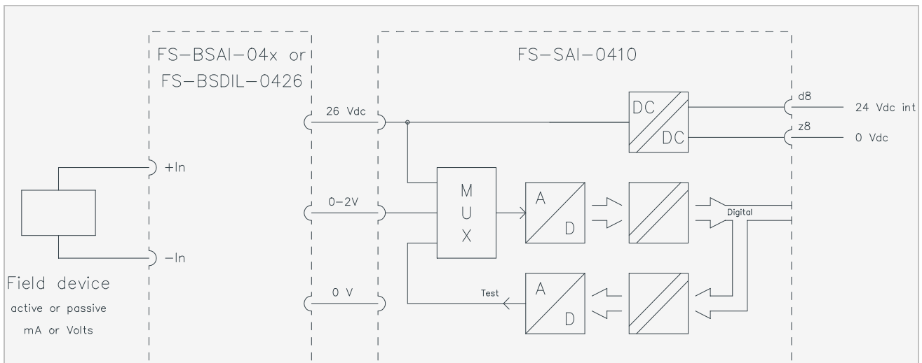
Figure 8-18: Schematic diagram for connection of inputs to the SAI-0410 module
