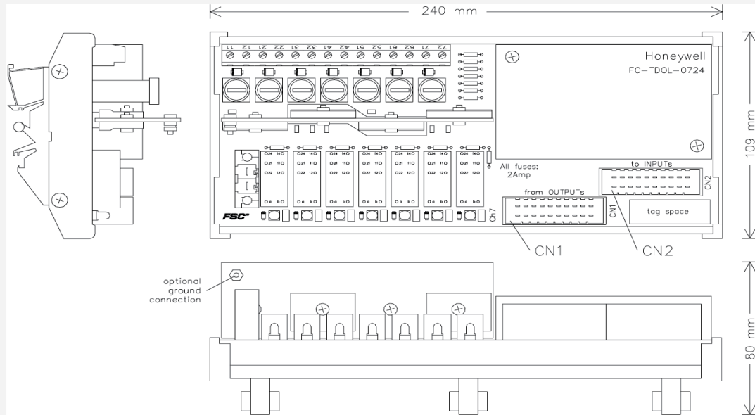
Figure 15-46: Mechanical layout
