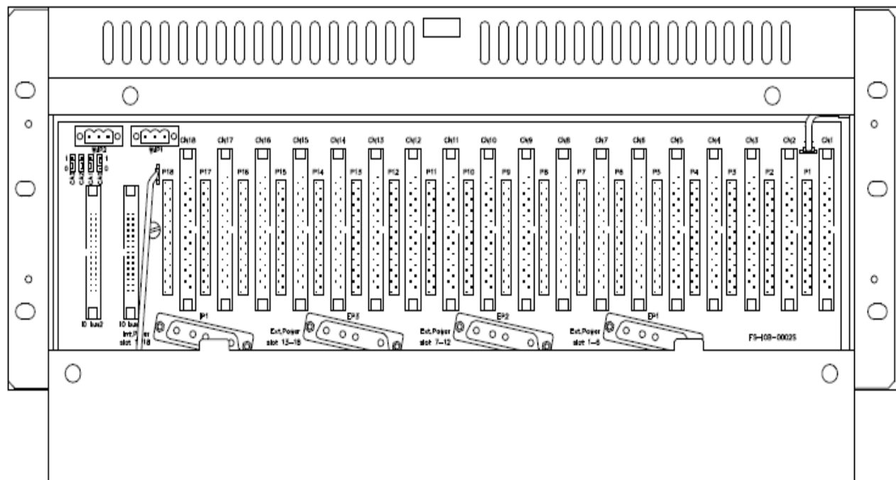
Figure 5-25: Back view of an open IOCHAS-0002S
