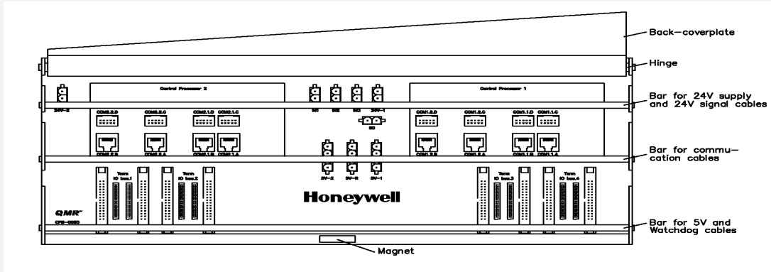
Figure 5-41: Back view of an empty Controller chassis
