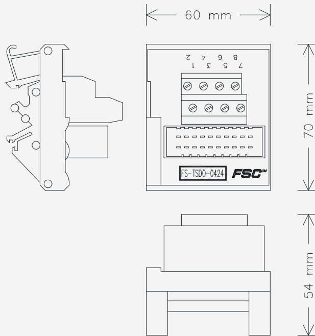
Figure 15-100: Mechanical layout
