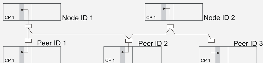
Figure 21-2: Example of a multidrop connection based on Ethernet
