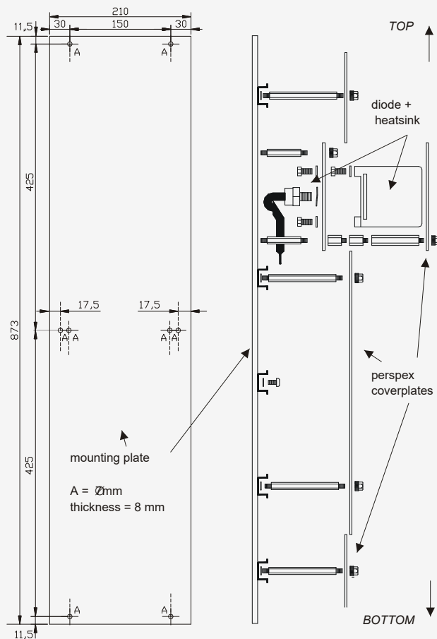
Figure 6-40: Mounting plan and measurements of the FEEDER-24R
