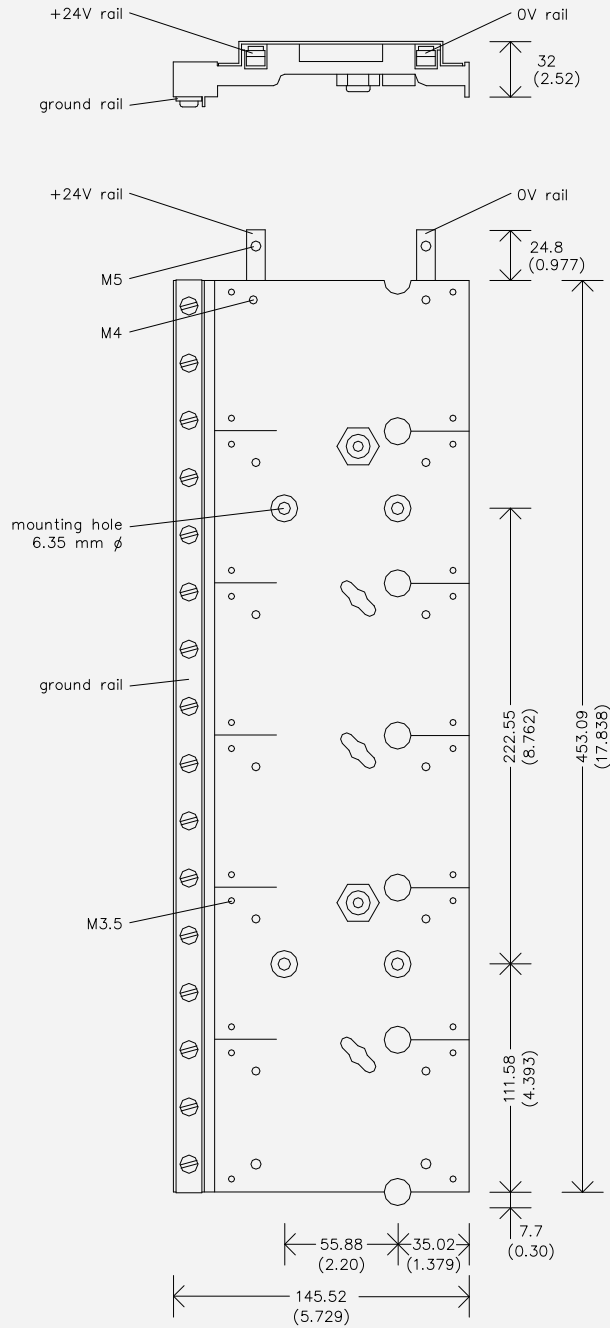
Figure 4-7: Mechanical layout
