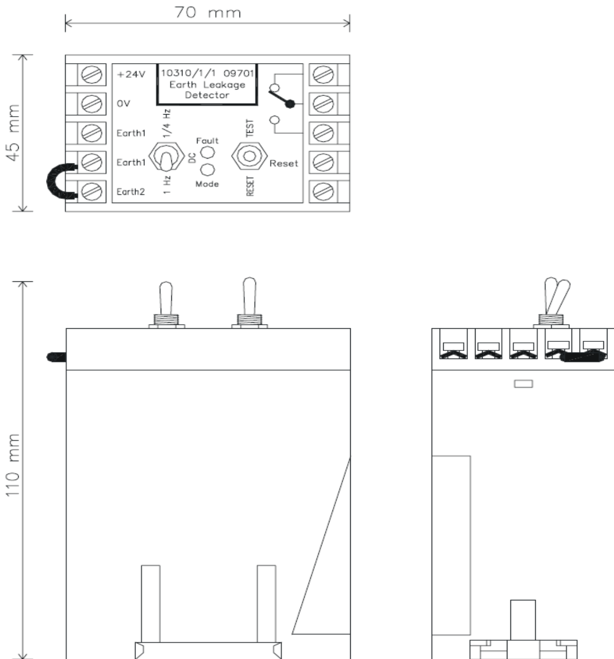
Figure 13-12: ELD module
