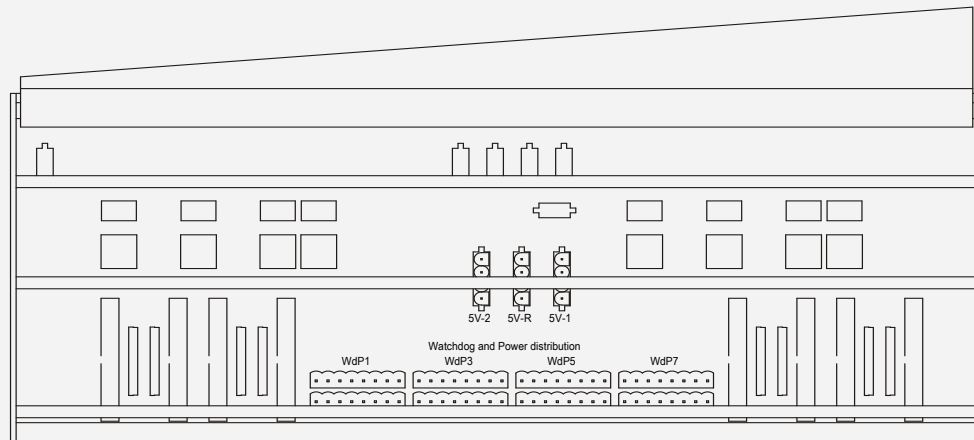
Figure 19-1: Position of the 5V and Wd connectors on a Controller backplane
