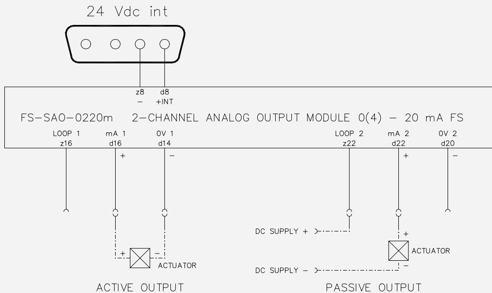
Figure 10-15: IO connection example for SAO-0220m module for non-redundant IO configurations (one channel active, one channel passive)
