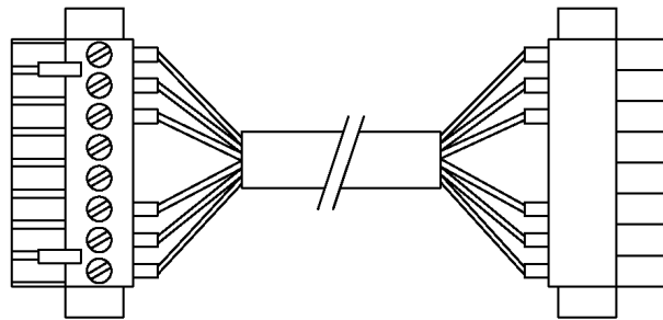
Figure 19-25: Pin assignment and layout of the PDC-IOR05A cable
