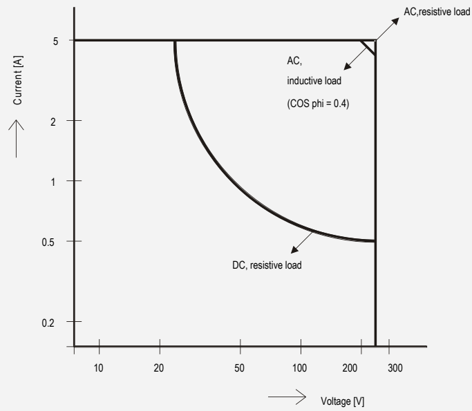
Figure 15-134: Maximum switched power
