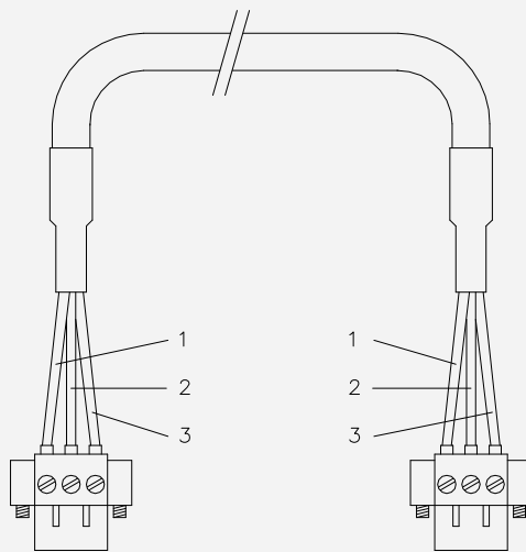
Figure 19-28: Wire assignment of the PDC-ART05 cable
