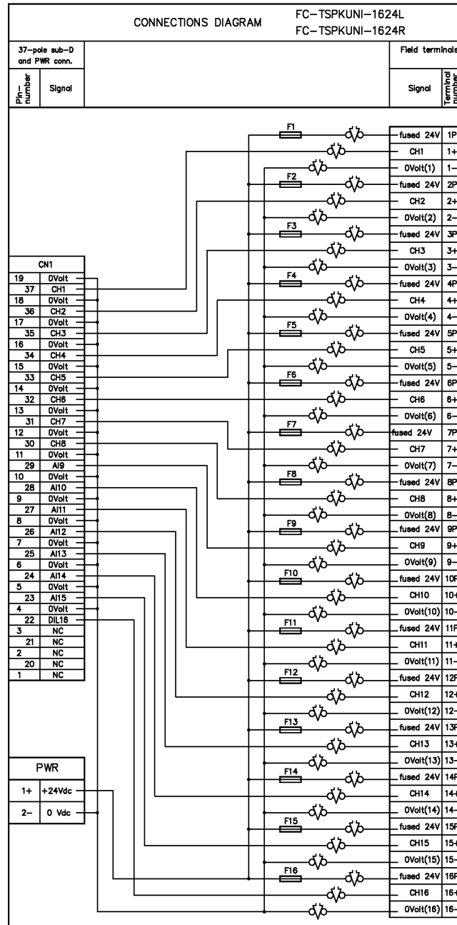
Figure 15-128: Connections diagram
