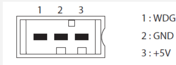
Figure 13-19: Pin connections of SCN-x
