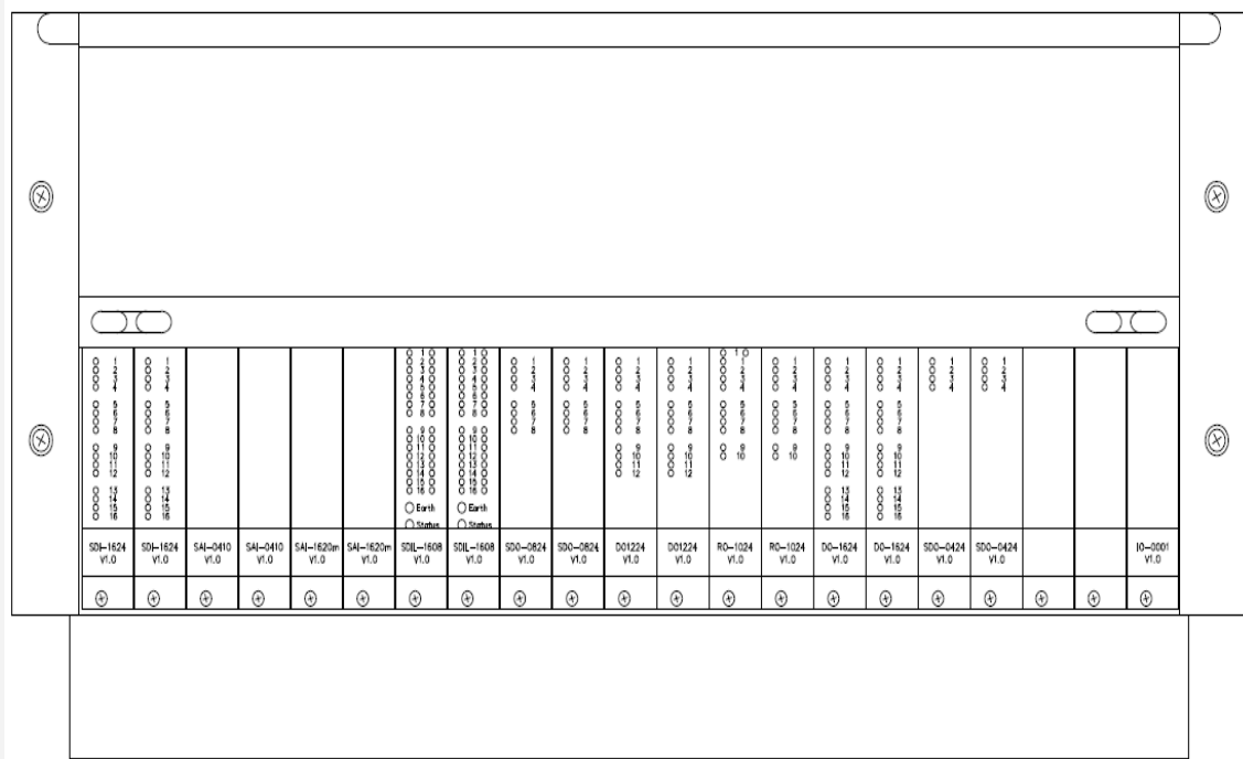
Figure 5-11: Front view of a filled, closed IOCHAS-0001S
