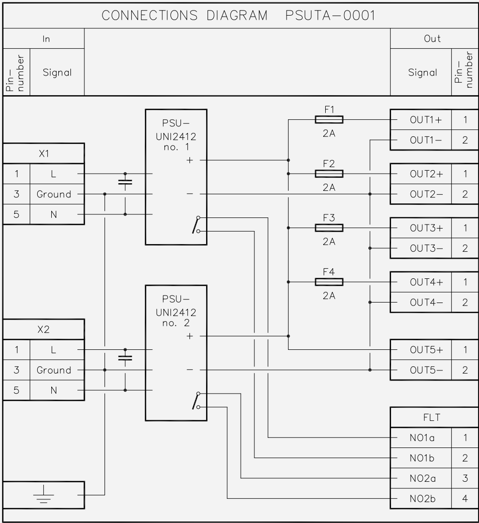
Figure 6-64: Connection diagram
