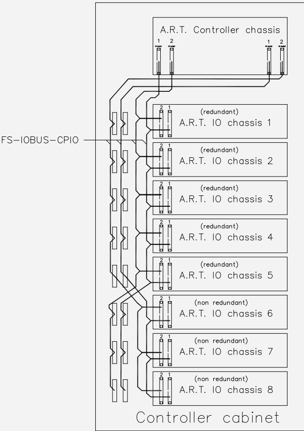
Figure 14-4: IO busses example for a IO chassis in the Controller cabinet
