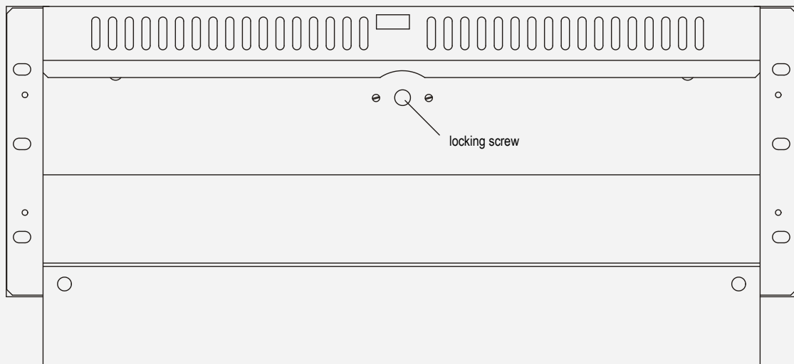
Figure 5-32: Back view of a closed IOCHAS-0002R
