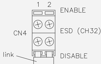
Figure 15-14: ESD (CH32) link
