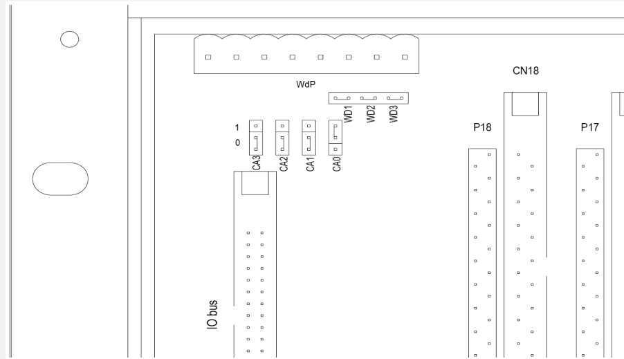
Figure 14-9: Jumpers on the CPB-0001S
