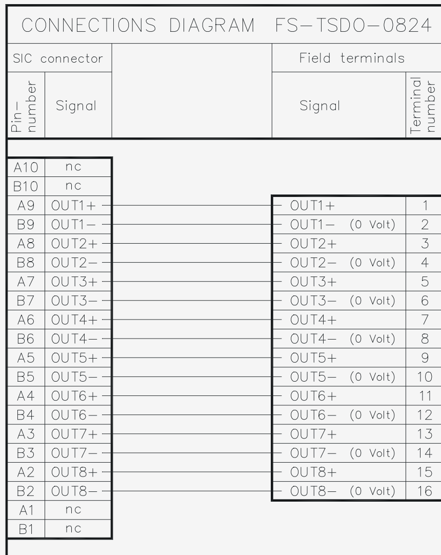
Figure 15-103: Connections diagram
