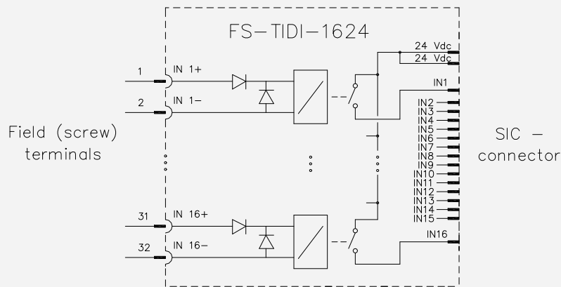
Figure 15-64: Schematic diagram
