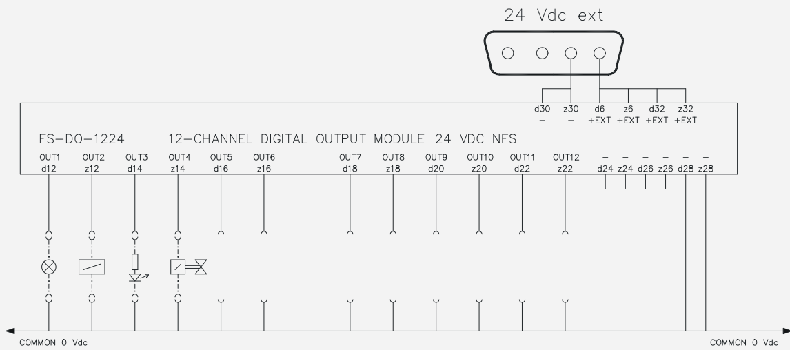
Figure 10-19: Connection example of DO-1224 module to FTA for both non-redundant and redundant IO configurations
