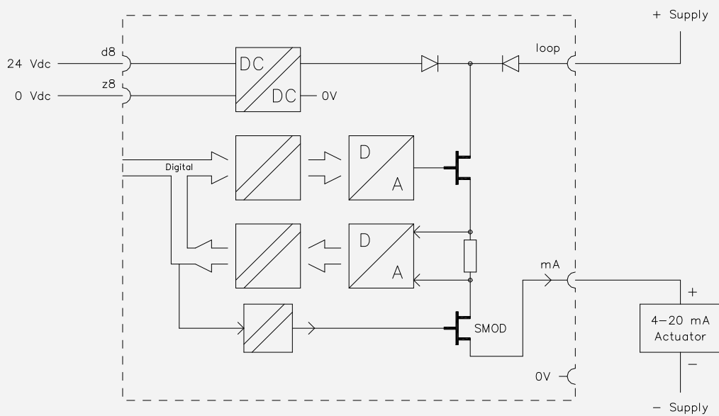
Figure 10-12: Schematic diagram for connection of the SAO-0220m module as a passive output
