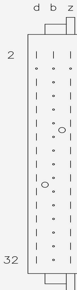
Figure 10-38: Back view and pin allocation of the SDO-0448 module connector
