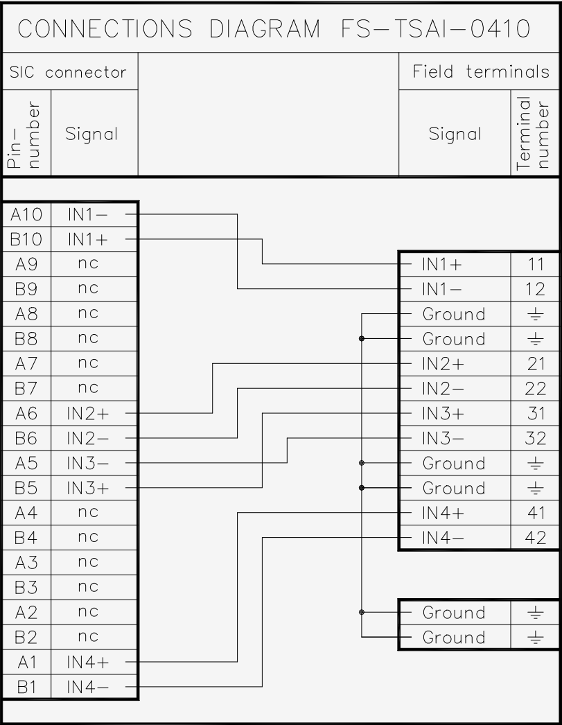
Figure 15-73: Connections diagram
