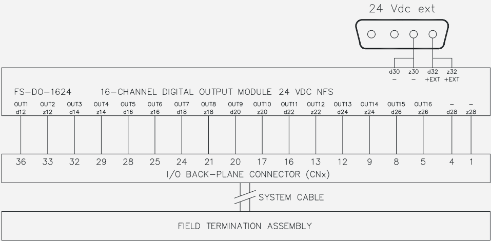
Figure 10-29: Connection example of DO-1624 module to FTA for both non-redundant and redundant IO configurations
