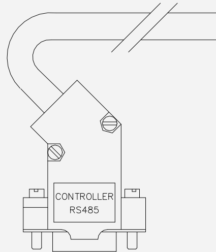
Figure 17-18: Pin assignment and layout of the CCE-485-FO-03/Lx communication cable
