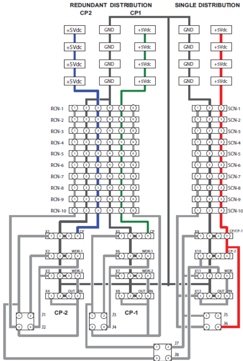
Figure 13-17: Connection diagram
