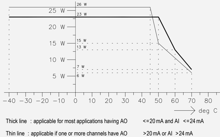
Figure 12-28: Module derating with a supply voltage of 31.2 V
