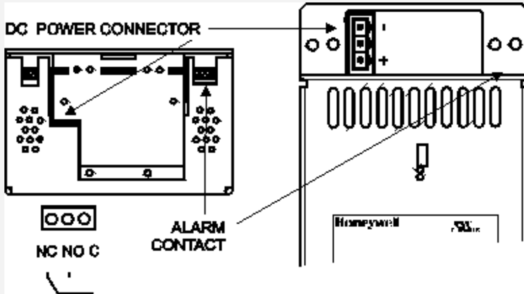
Figure 6-34: Connections on the output side of the PSU-UNI12010U
