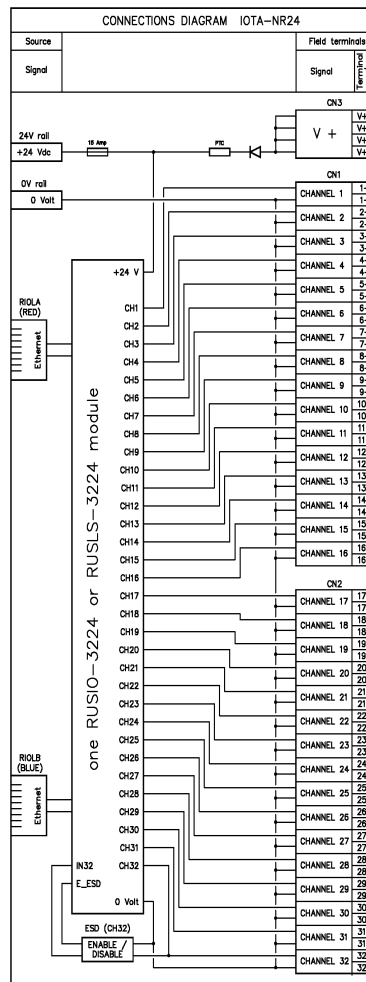
Figure 15-16: Connection diagram
