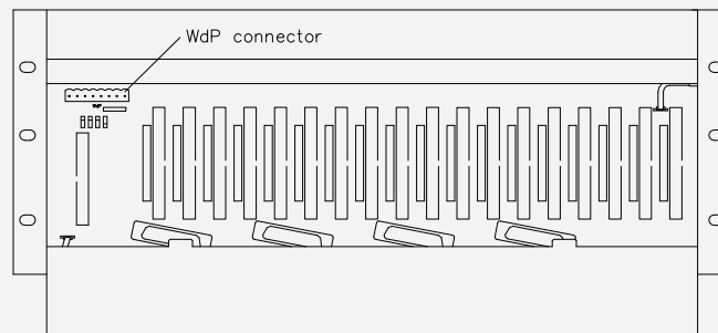
Figure 19-14: Position of the WdP connector on a non-redundant IO chassis
