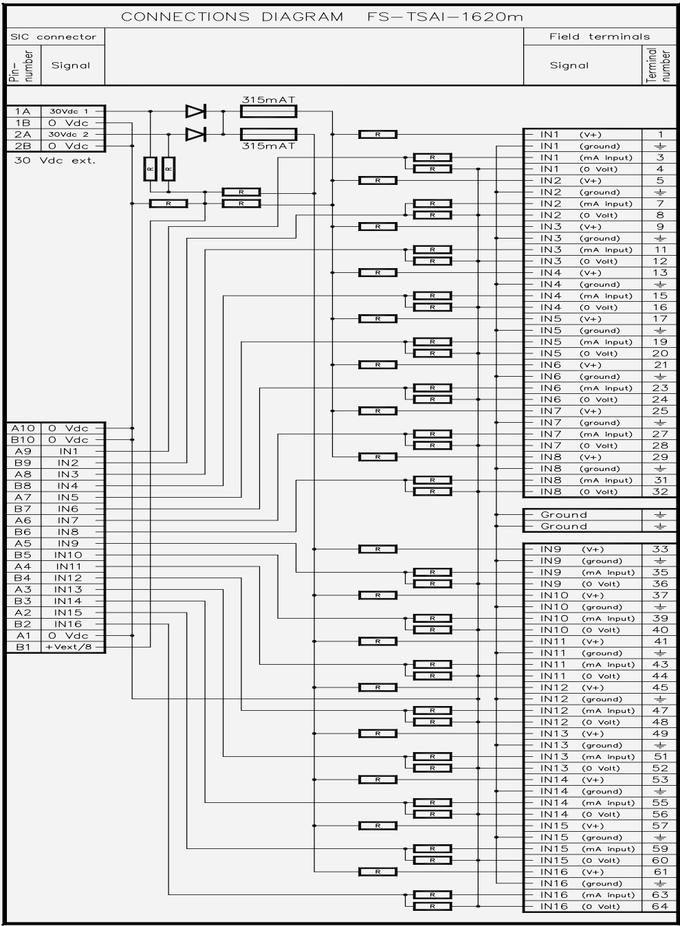
Figure 15-78: Connections diagram
