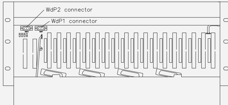
Figure 19-8: Position of the WdP connector on a non-redundant IO chassis
