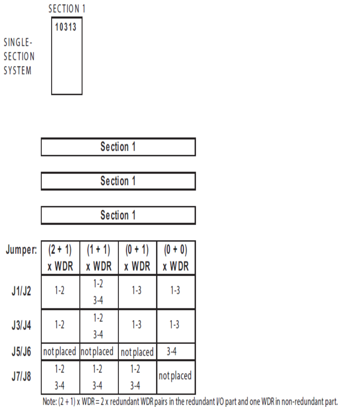
Figure 13-27: Distribution example
