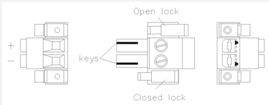
Figure 18-23: Power connector on In (Weidmuller BVZ 7.62HP/02F SN) top, side and bottom view
