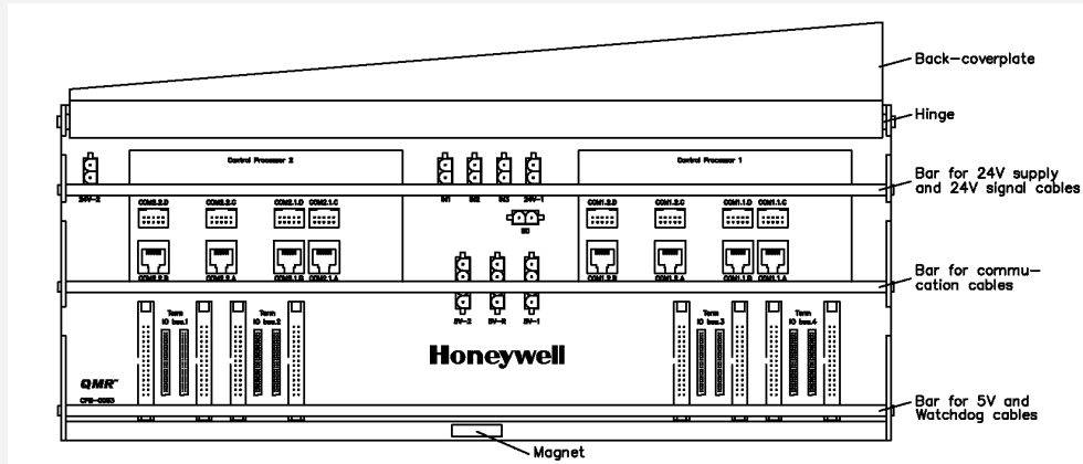
Figure 19-13: Position of the 5V and Wd connectors on a Controller backplane
