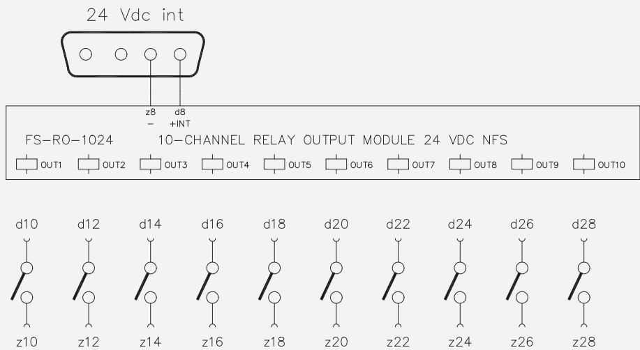
Figure 10-25: IO connection example for RO-1024 module for non-redundant IO configurations
