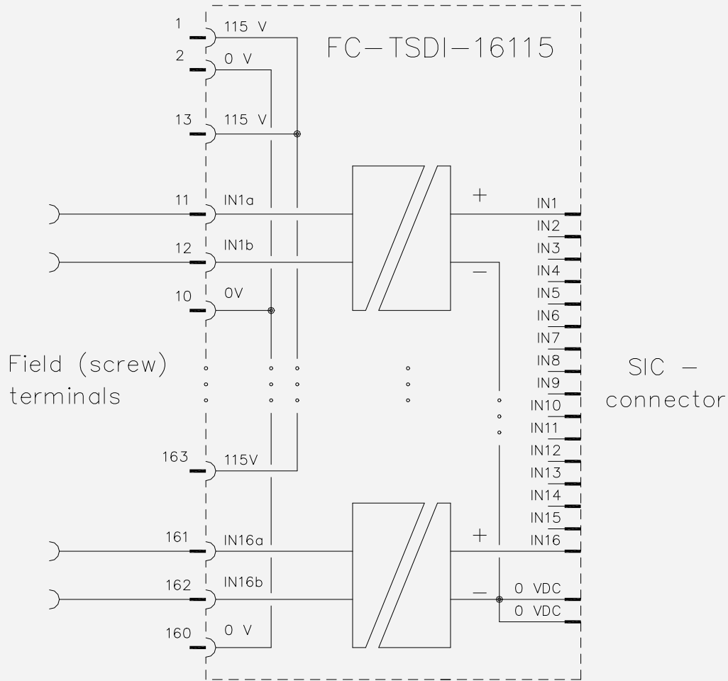
Figure 15-89: Schematic diagram for connecting active inputs
