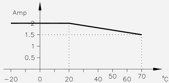
Figure 15-62: Derating curve (channel load vs ambient temperature) for the TDOL-0724U
