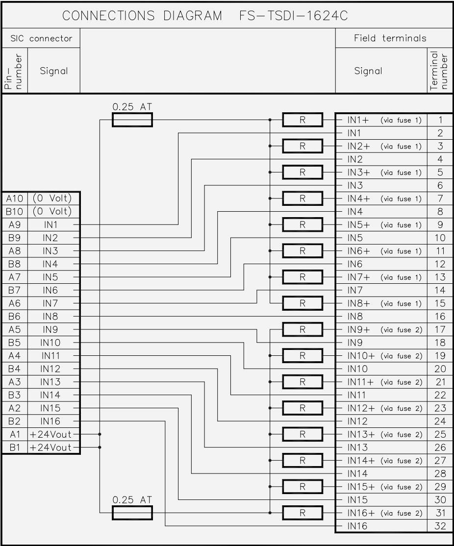
Figure 15-95: Connections diagram
