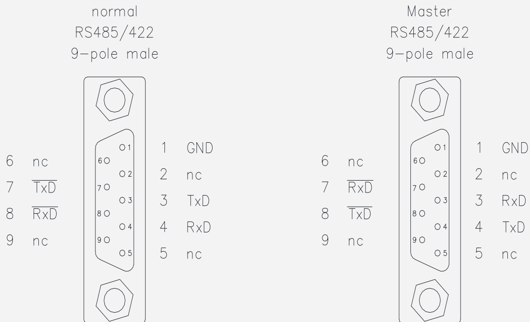
Figure 15-7: Pin allocation of the connectors on the DCOM-485
