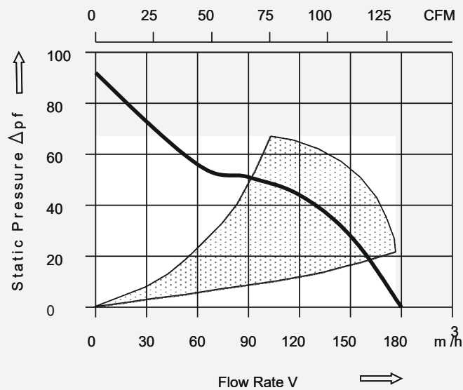
Figure 4-4: Flow rate against static pressure (per fan)
