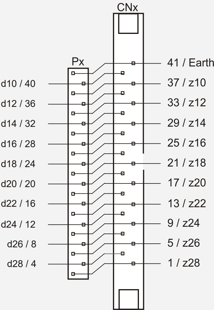
Figure 5-9: Pin mapping from IO connector to SIC cable (CNx) and converter (Px) connector
