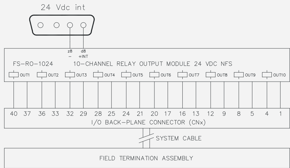
Figure 10-24: Connection example of RO-1024 module to FTA for both non-redundant and redundant IO configurations
