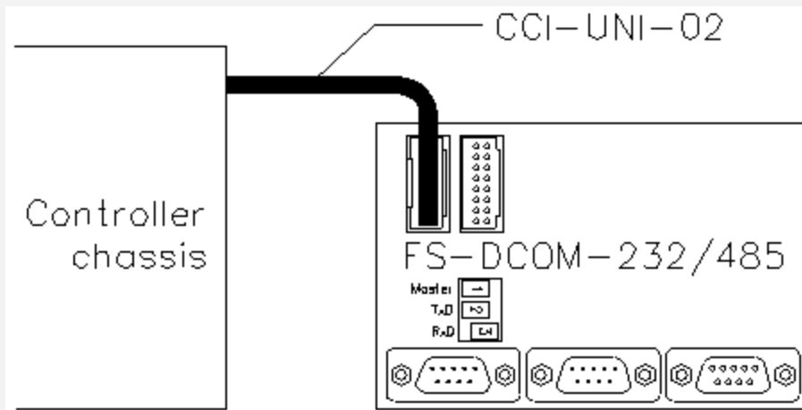
Figure 17-1: Non-redundant internal communication wiring to a DCOM-232/485 module
