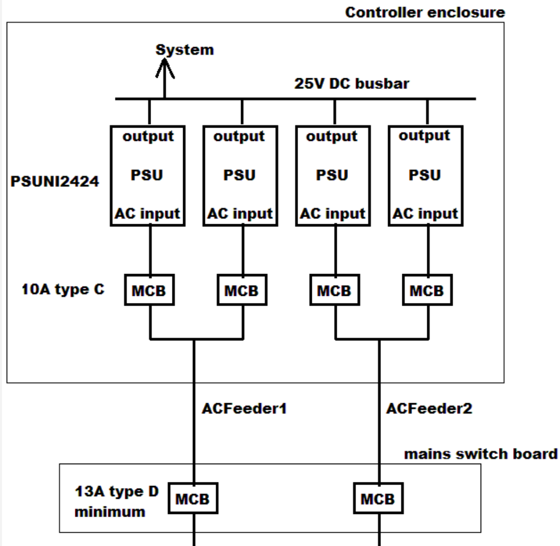
Figure 7-14: Controller power supply configuration
