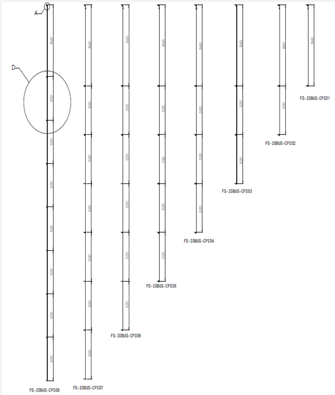
Figure 14-16: Separate cable assemblies
