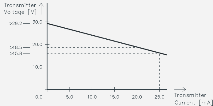
Figure 15-119: Transmitter voltage for passive transmitters
