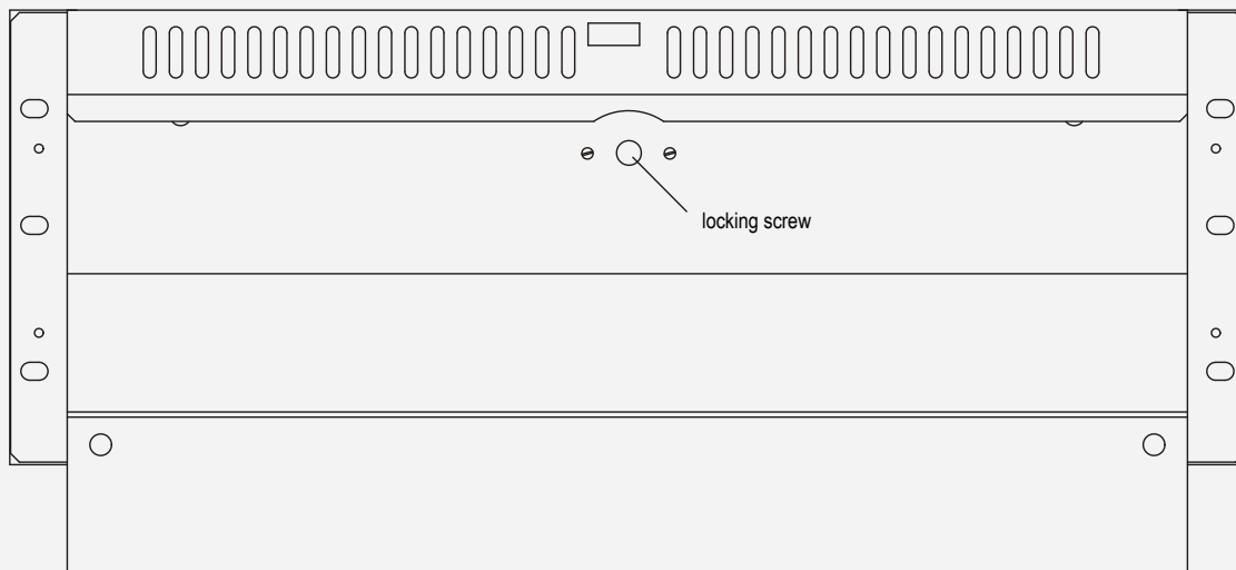
Figure 5-52: Back view of a closed IOCHAS-0003R
