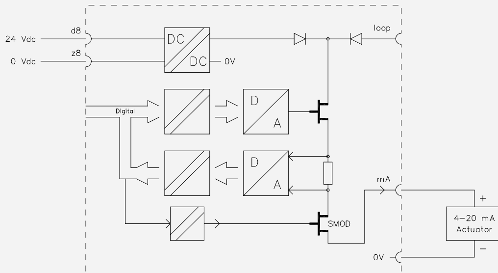
Figure 10-11: Schematic diagram for connection of the SAO-0220m module as an active output
