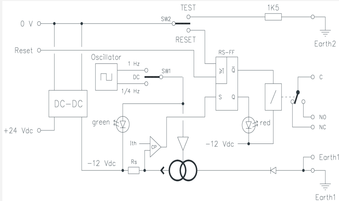
Figure 13-13: Block diagram of 10310/3/1 ELD
