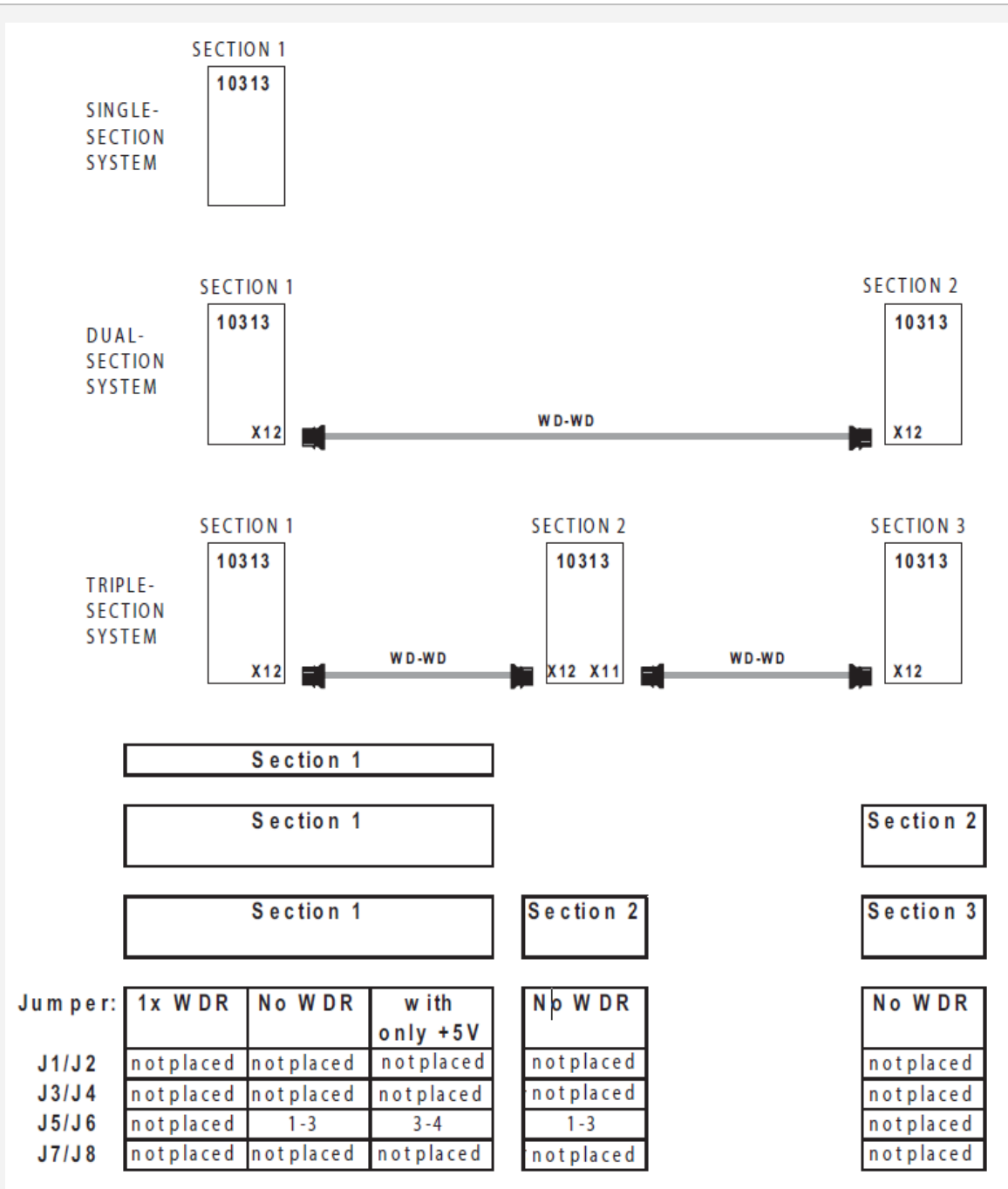
Figure 13-24: Distribution example
