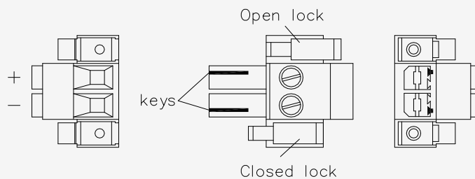
Figure 15-61: Power input connector (Weidmuller BVZ 7.62HP/02/180F SN) top, side and bottom view
