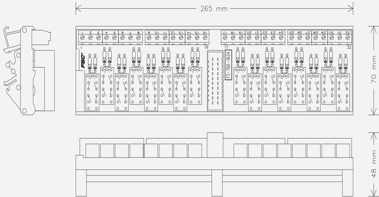
Figure 15-63: Mechanical layout
