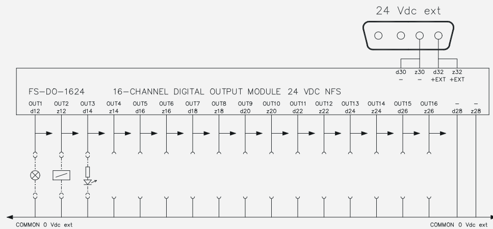
Figure 10-31: IO connection example for DO-1624 module for redundant IO configurations
