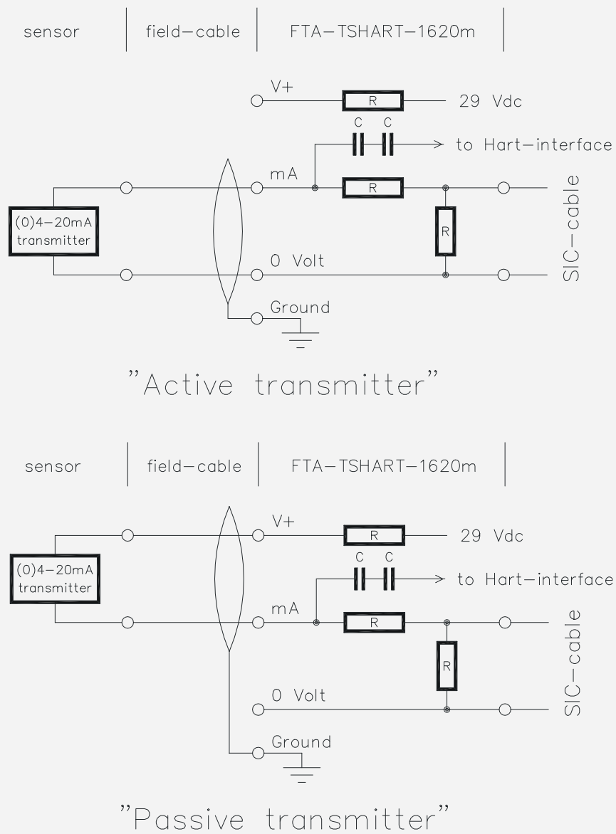
Figure 15-118: Schematic diagram for connecting a transmitter
