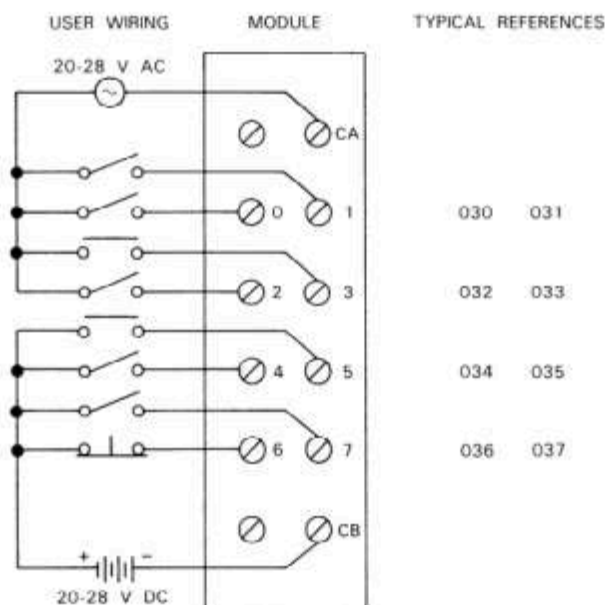
WIRING DIAGRAM
