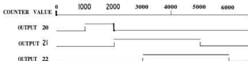
Figure 5.17 HIGH SPEED COUNTER TIMING CHART
