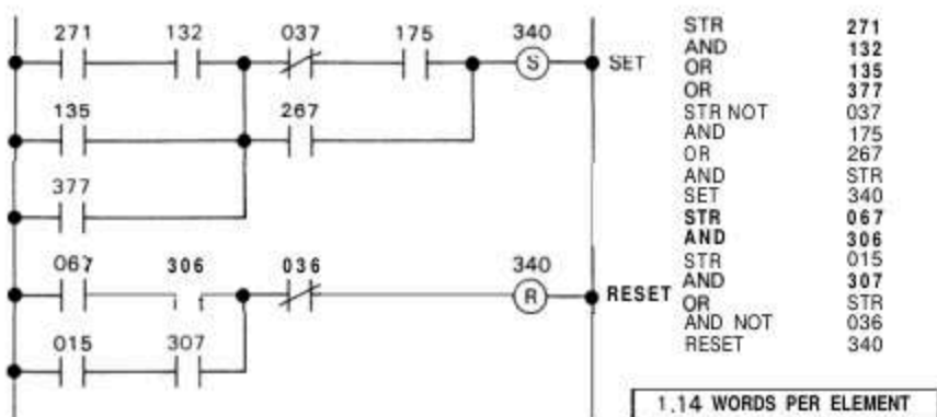
Figure 5.8 SAMPLE LATCHING LOGIC
