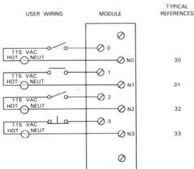
WIRING DIAGRAM
