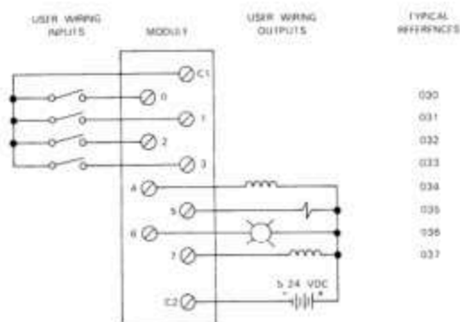
WIRING DIAGRAM
