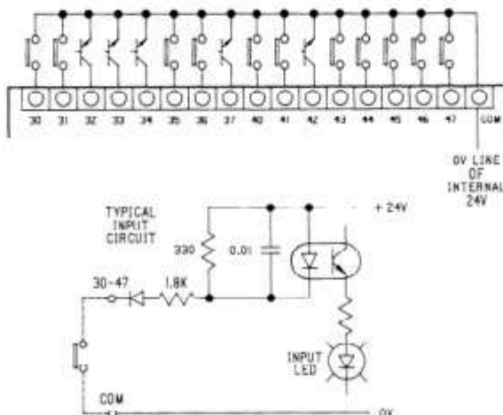
Figure 6.43 FIELD WIRING INFORMATION AND TYPICAL INPUT CIRCUIT
