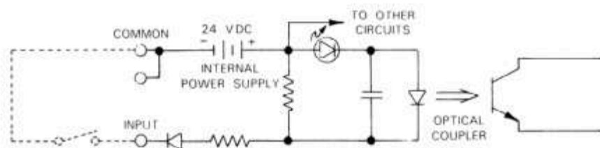
SAMPLE INPUT CIRCUIT
