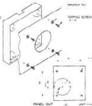
Figure 3.10 PROGRAMMER MOUNT ASSEMBLY
