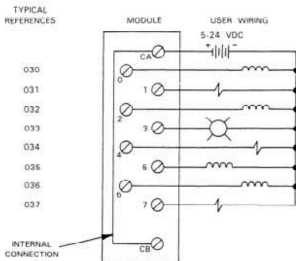
WIRING DIAGRAM
