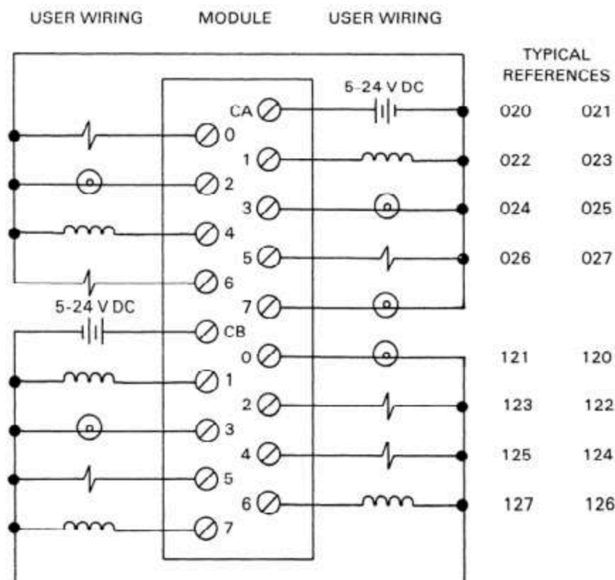
WIRING DIAGRAM
