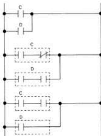
EXAMPLES OF OR (C + D)
