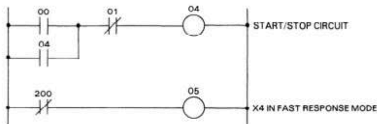
Figure 8.11 FAST RESPONSE START/STOP LOGIC
