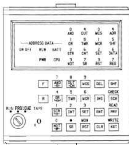
Figure 5.2 PROGRAMMER
