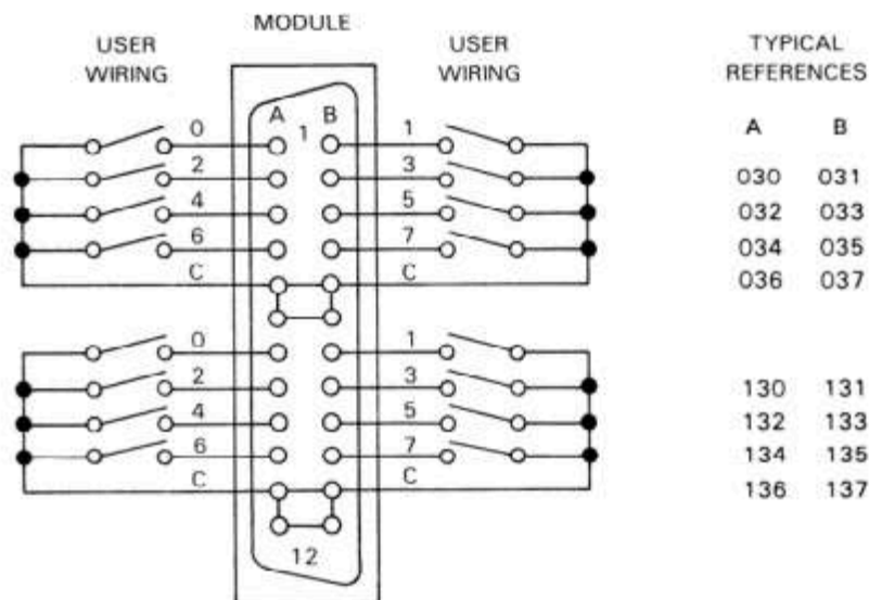
WIRING DIAGRAM
