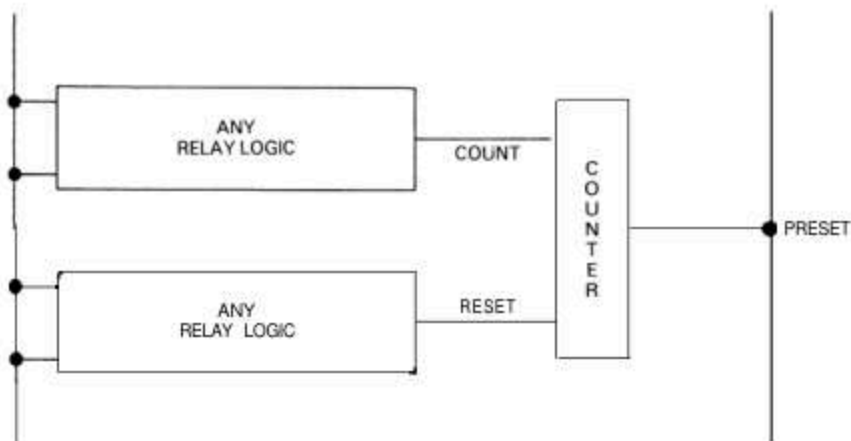
Figure 5.14 COUNTER LOGIC REQUIREMENTS
