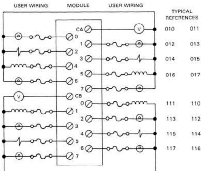
WIRING DIAGRAM
