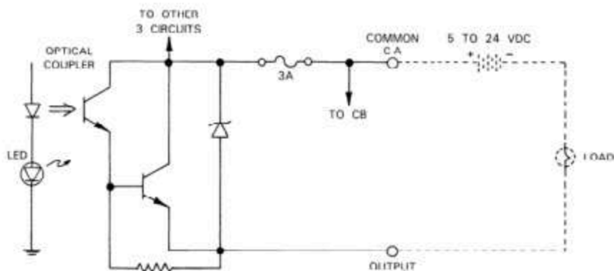
SAMPLE OUTPUT CIRCUIT
