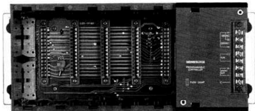
5-SLOT RACK
