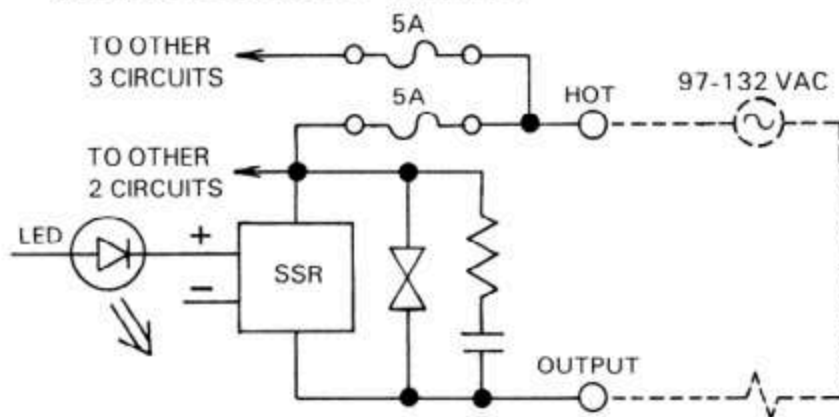
SAMPLE OUTPUT CIRCUIT
