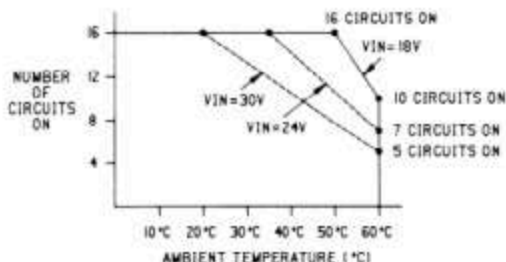
Figure 6.59 I/O POINTS VS TEMPERATURE CHART
