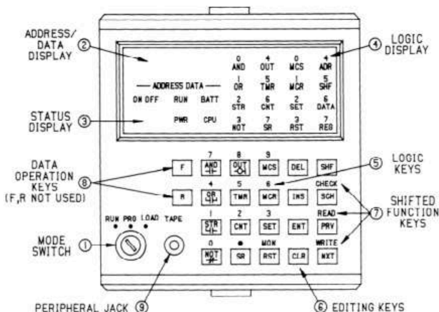
Figure 4.1 PROGRAMMER FEATURES
