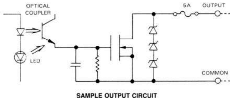
Figure 6.30 WIRING OF 24 V dc 2 AMP SINK/SOURCE OUTPUT
