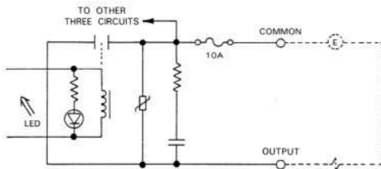
SAMPLE RELAY OUTPUT CIRCUIT
