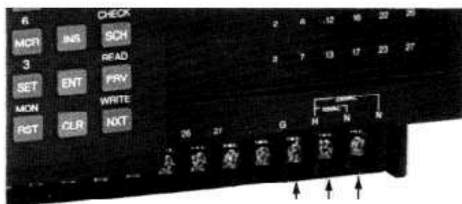
Figure 3.4 POWER CONNECTIONS
