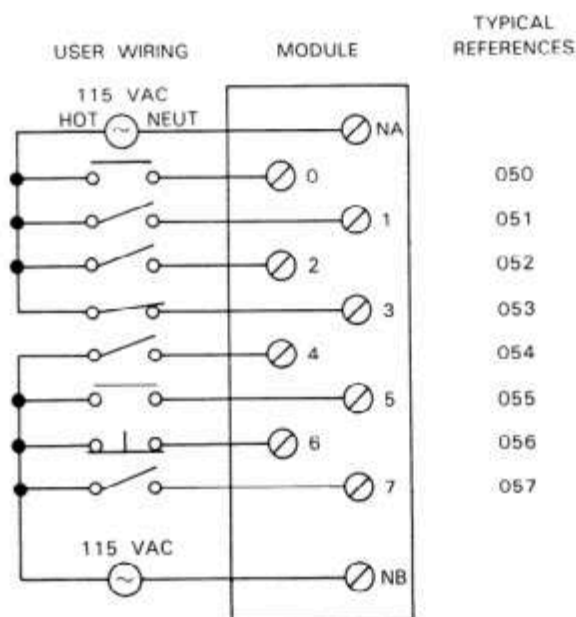
WIRING DIAGRAM
