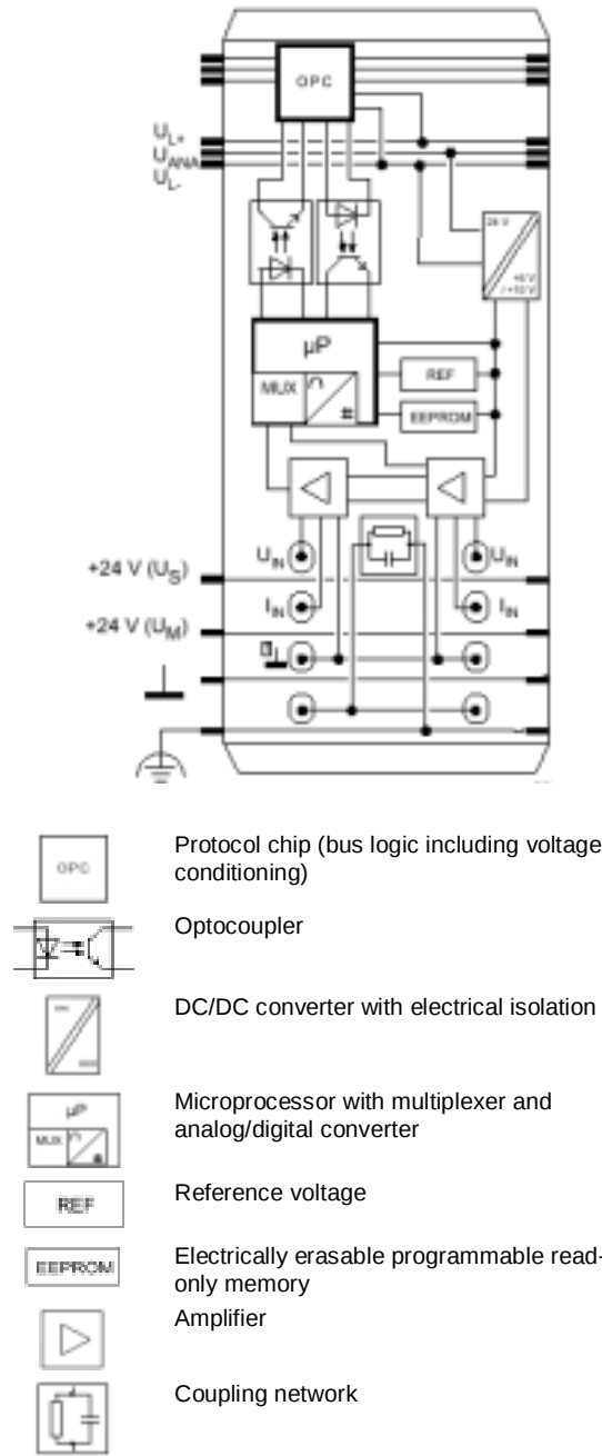
Internal Circuit Diagram
