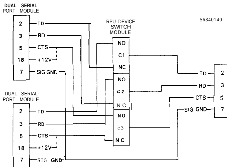
Figure 2. Peripheral Connections
