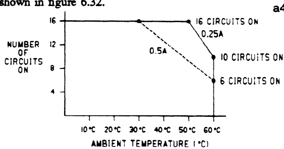
Figure 6-32. I/O Points vs Temperature
