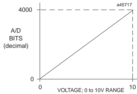
Figure 10-10. A/D Bits vs. Voltage Input for IC693ALG222
