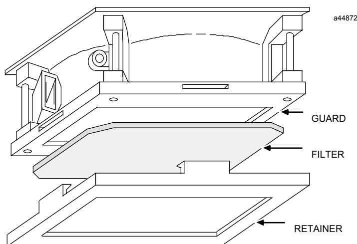
Figure 5. Filter Guard Assembly (AC Type Fan Shown)
