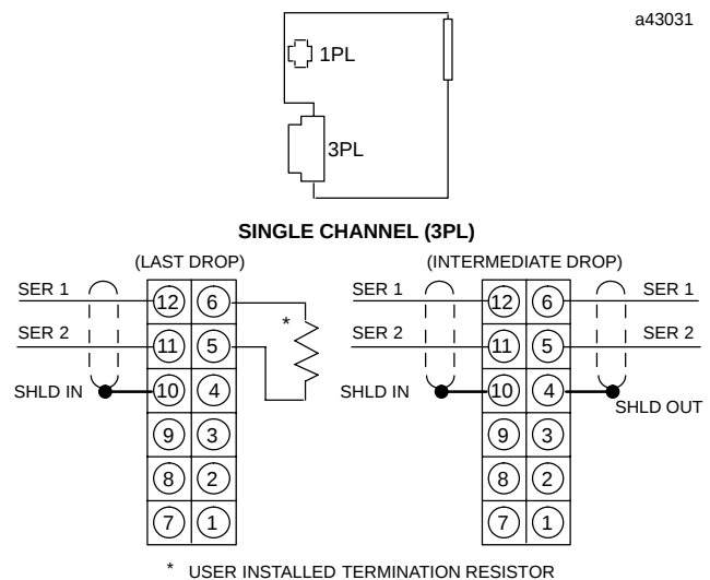
Figure 5. Wiring Diagram
