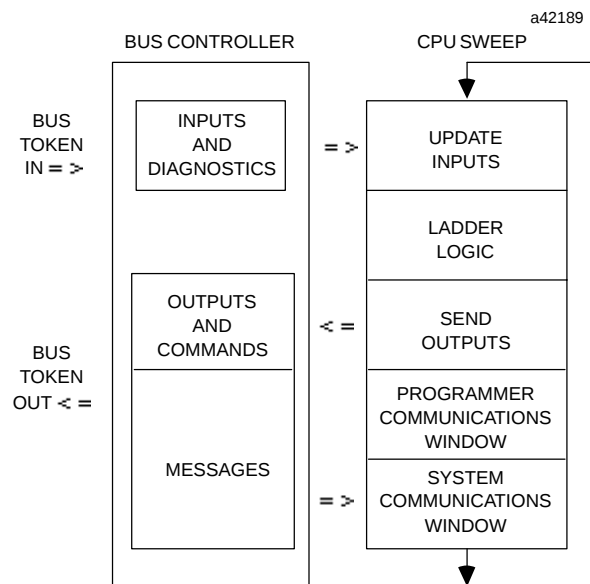
Figure 4. CPU Sweep
