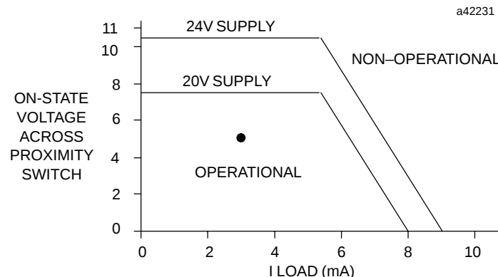
Figure 2. Proximity Switch Compatibility
