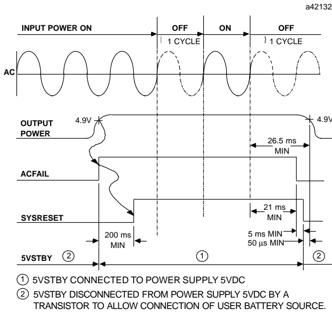
Figure 2. Timing Diagram
