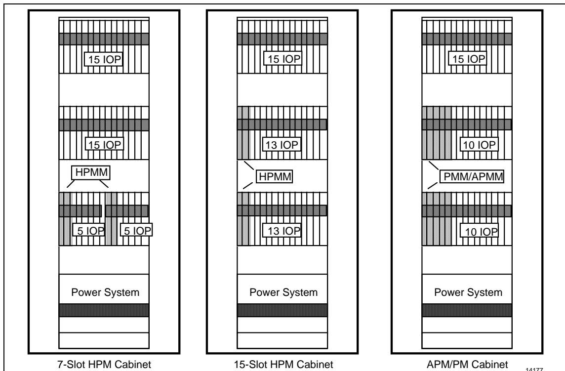
Figure 4 — Typical Cabinets
