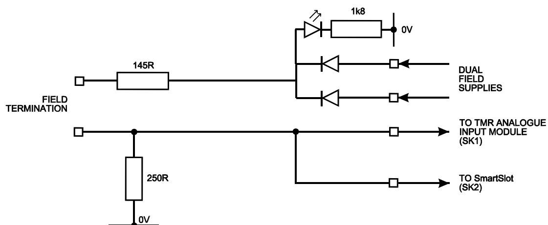
Figure 2 Single Channel Schematic
