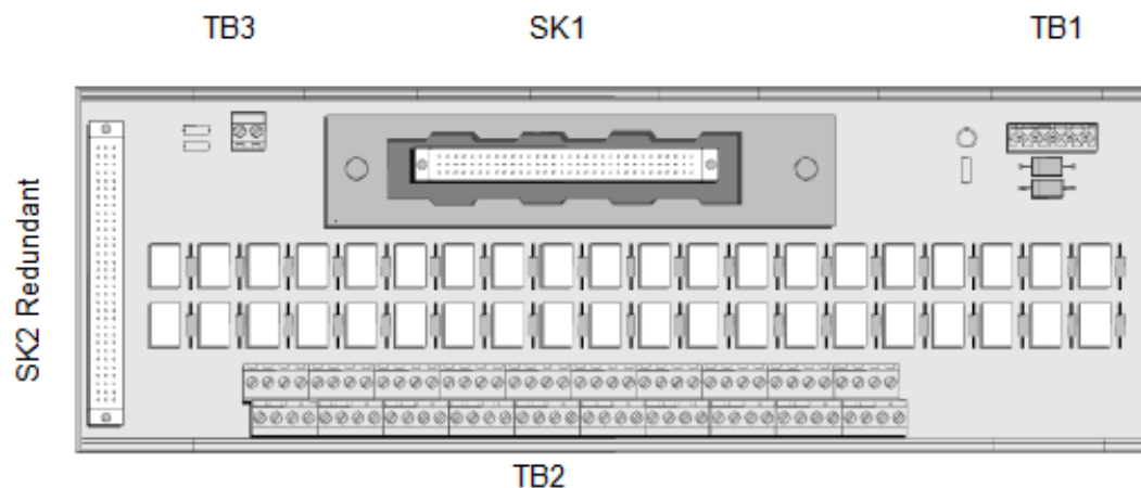
Figure 1 T8831 Layout
